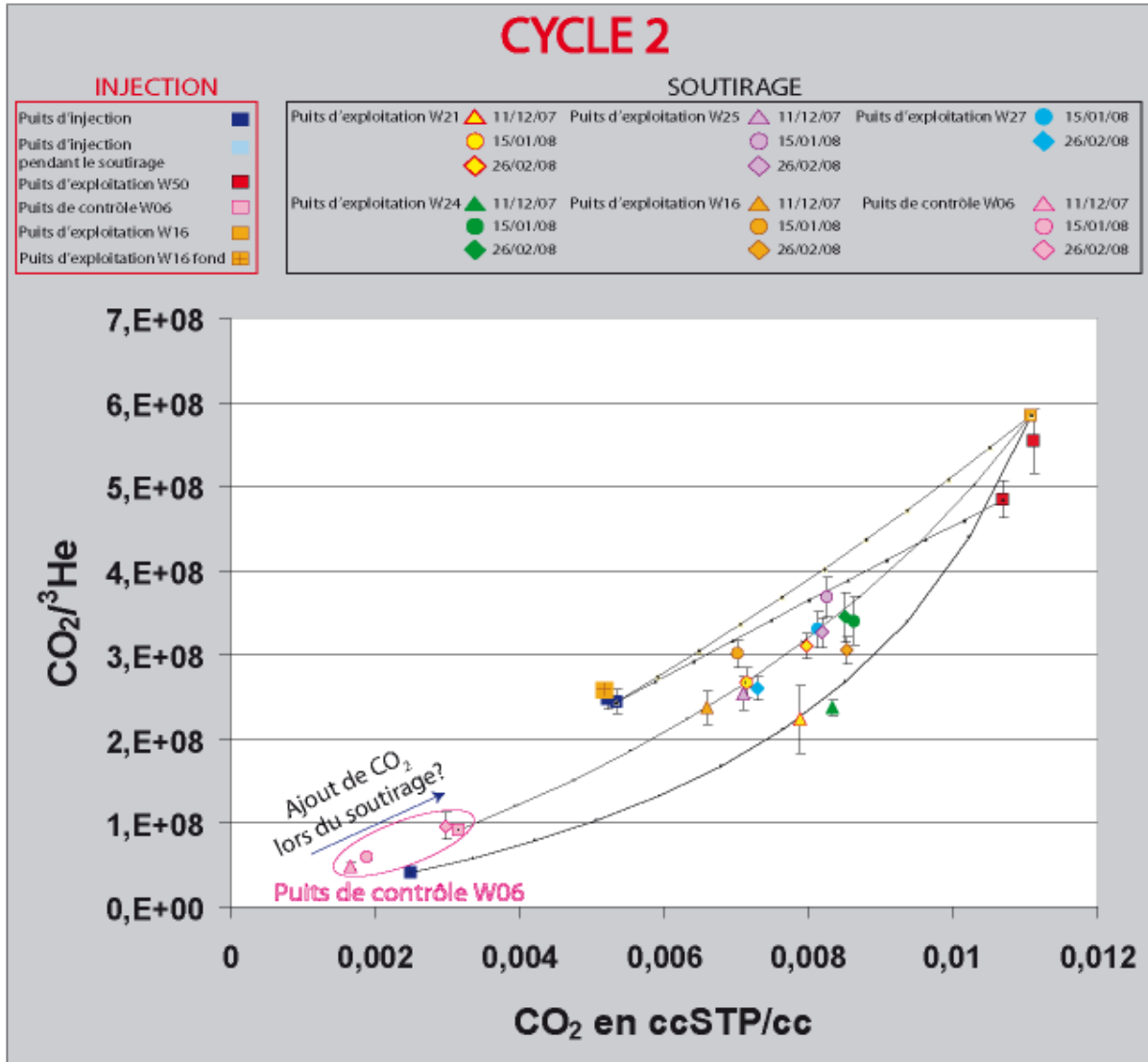
Figure 4.51: Diagramme CO_2/{}^3He versus CO_2 (cycle 2)
