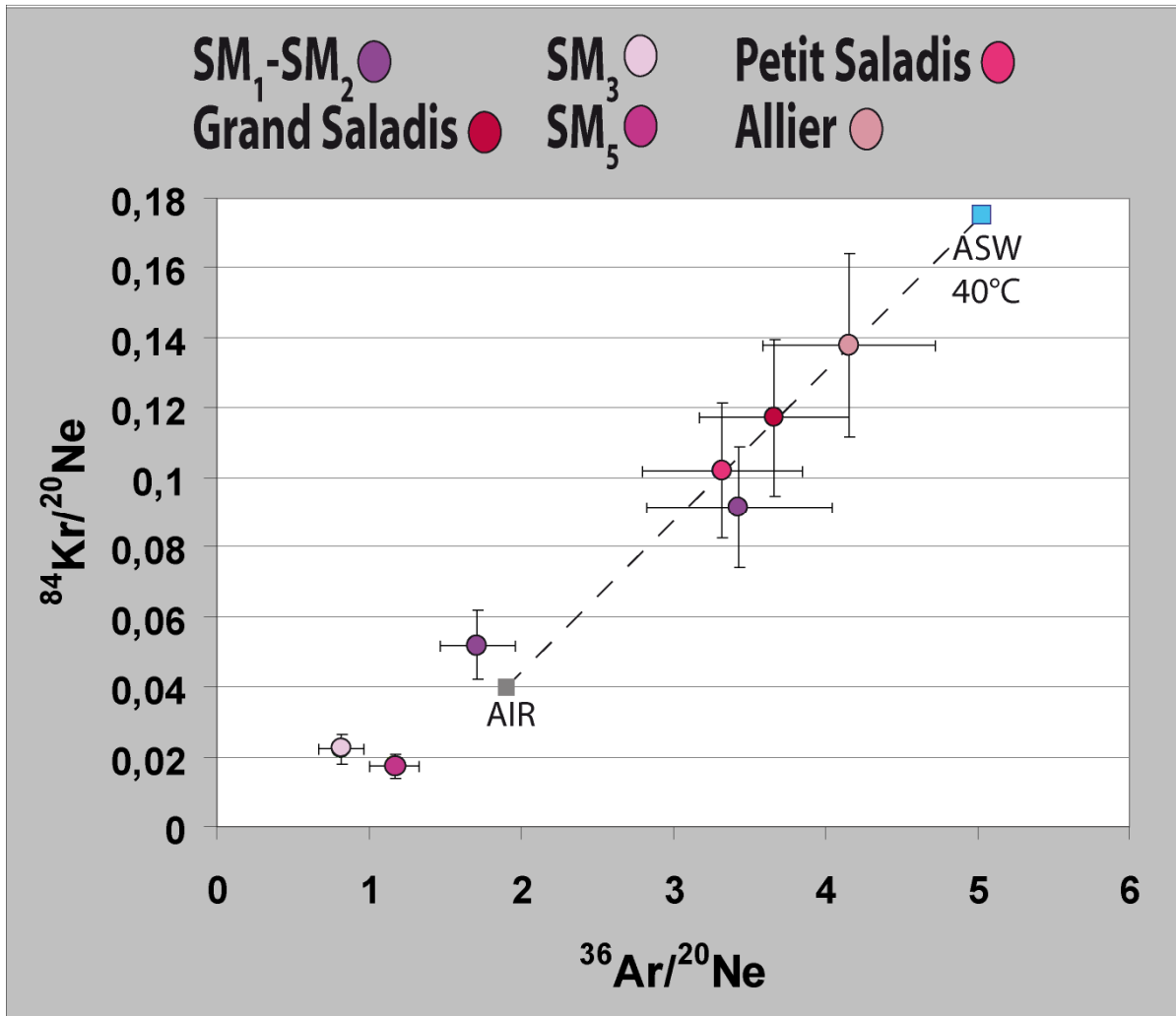
Figure 3.38: ^{84}\text{Kr}/^{20}\text{Ne} versus ^{36}\text{Ar}/^{20}\text{Ne} (Sainte Marguerite).
