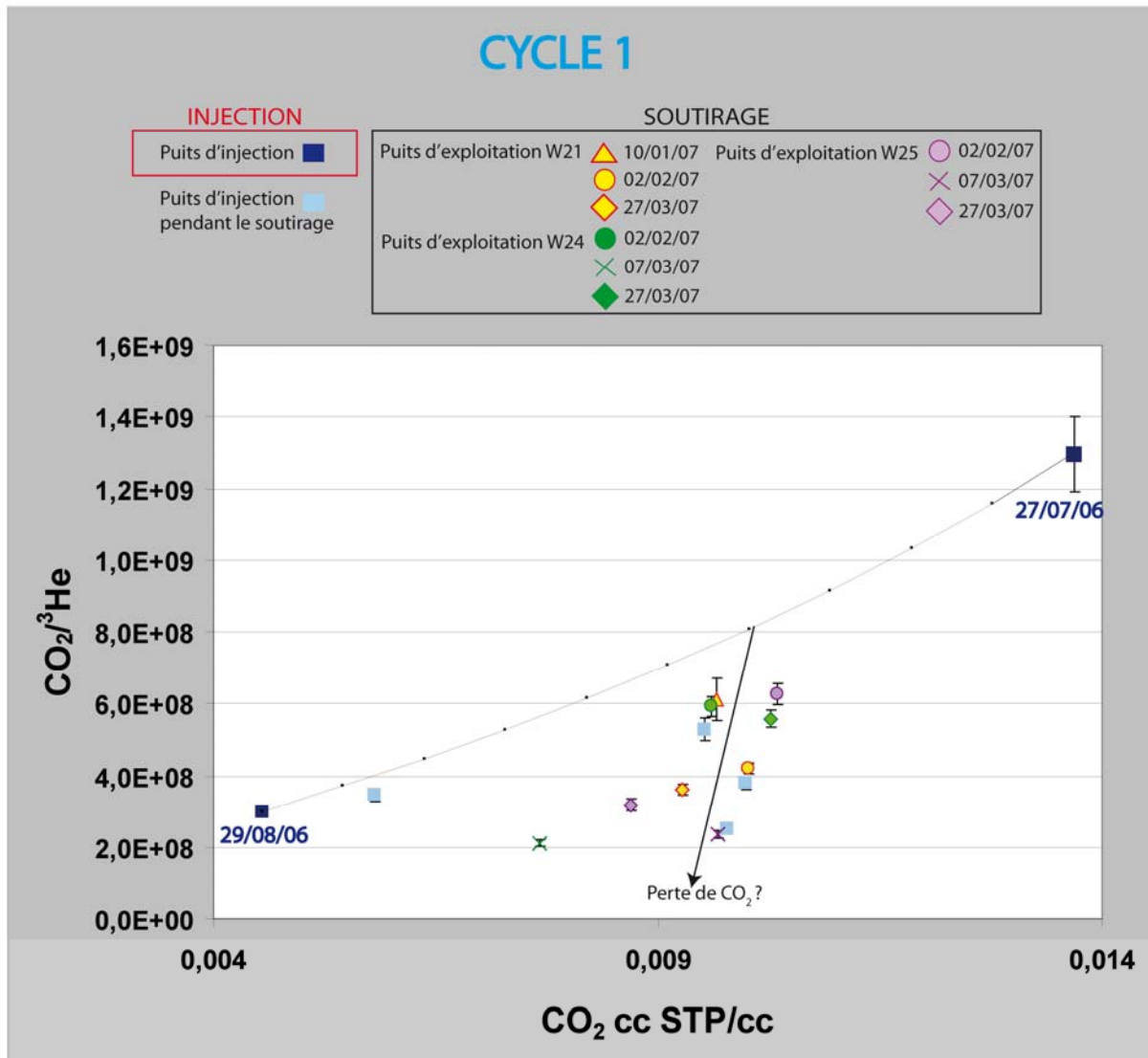
Figure 4.50: Diagramme CO_2/{}^3He versus CO_2 (cycle 1)
