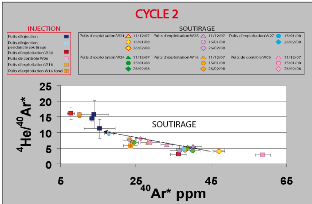
Figure 4.41: ^4\text{He}/^{40}\text{Ar}^* versus ^{40}\text{Ar}^* (cycle 2).
