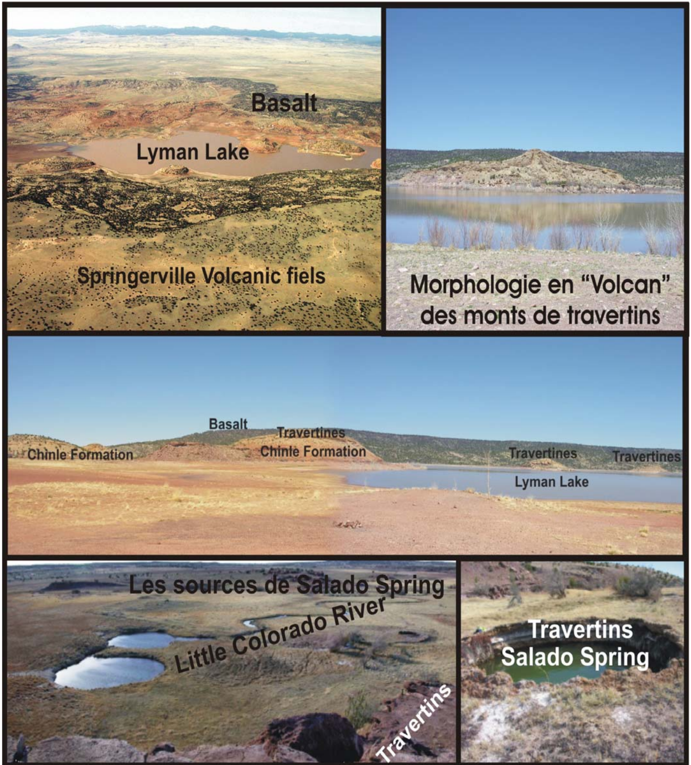
Figure 3.62: Lyman Lake et Salado Spring.
