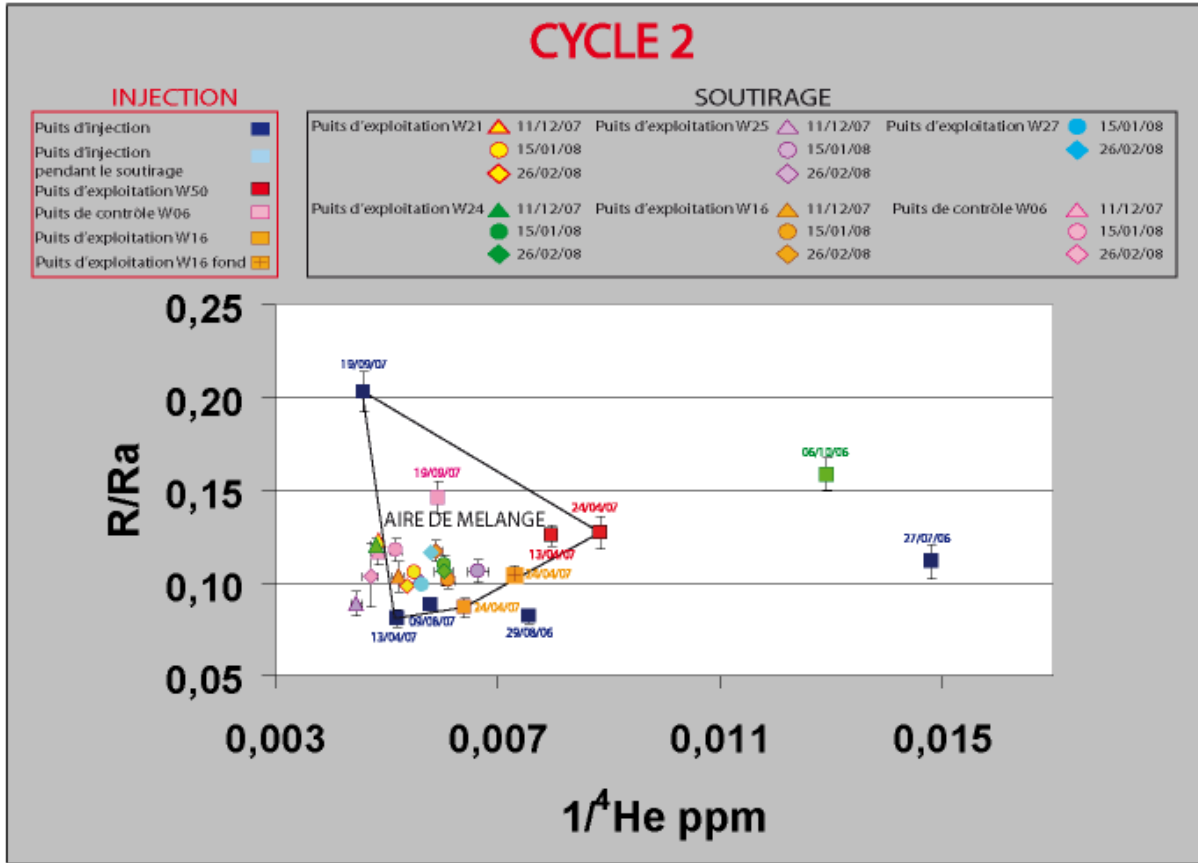
Figure 4.35: R/Ra versus 1/4He (ppm) (cycle 2)
