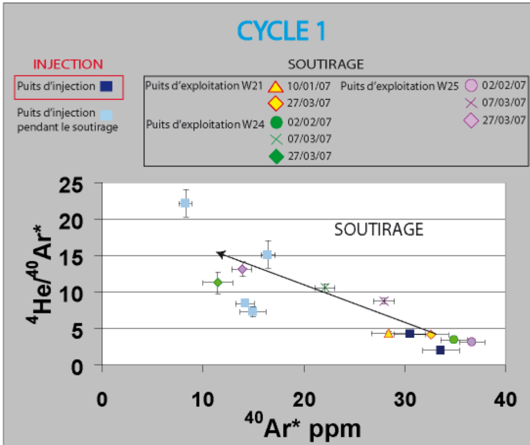
Figure 4.40: ^4\text{He}/^{40}\text{Ar}^* versus ^{40}\text{Ar}^* (cycle 1).
