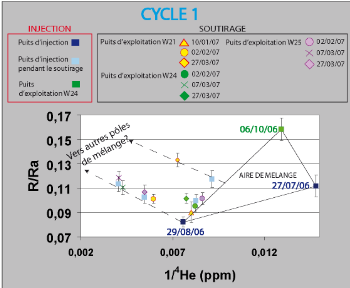
Figure 4.34: R/Ra versus 1/{}^4He (ppm) (cycle 1)
