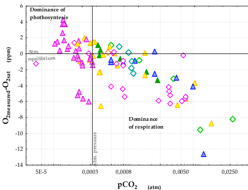
Figure 4.2.2.5 Differences between the measured oxygen partial pressure and oxygen atmospheric value is reported against p\text{CO}_2 values. For legend see Figure. 4.2.2.2
