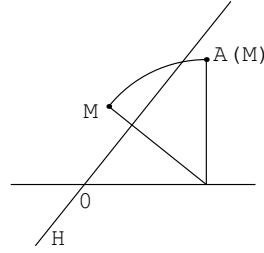
Figure 2.1: The linear transformation A
