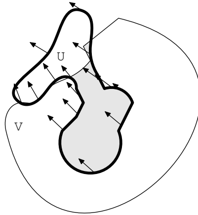
Figure 1.1: Evolution of the area between two Lipschitz curves. (The arrows represent the value of X on the boundary of U )
