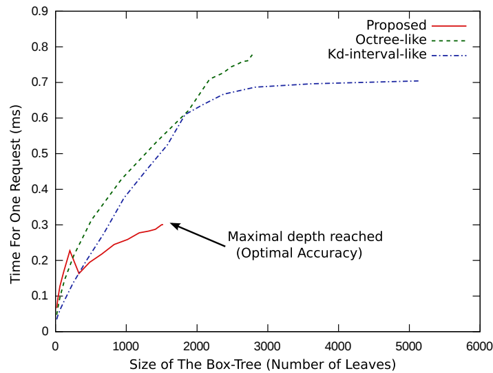
Figure 4.7 – Experimental results comparing the time spent for the viewpoint request with regard to the size of the data-structure ( lower is better ).
