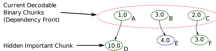
Figure 2.19 – The Counter-Example of non-optimality of the basic ordering policy. The ordering method (or the FIFO packetization strategy in the next chapter) will give the following order to the binary chunks: {B, E, C, F, A, D} but the total quality would have been improved faster with, for example, the order {A, D, B, E, C, F}
