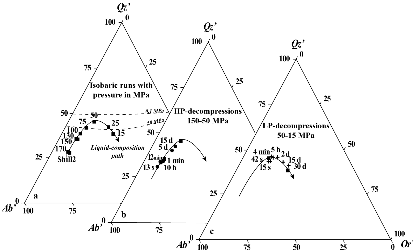
Fig. 11a–c Projection of the melt compositions in the haplogranite system corrected for An-bearing melts (Qz'–Ab'–Or'; Blundy and Cashman 2001, adapted from Tuttle and Bowen 1958). a Isobaric runs and starting composition (SHILL2); Qz'–feldspar cotectics for the Qz'–Ab'–Or' (An-free) system at 50 and 0.1 MPa after Tuttle and Bowen (1958). b HP decompressions from 150 to 50 MPa. c LP decompressions from 50 to 15 MPa (for b and c , point labels are the decomposition duration, and the squares denote the melt compositions of the isobaric run at initial and final pressure). Errors on Qz', Ab', and Or' components are up to 2 wt% (Blundy and Cashman 2001)
