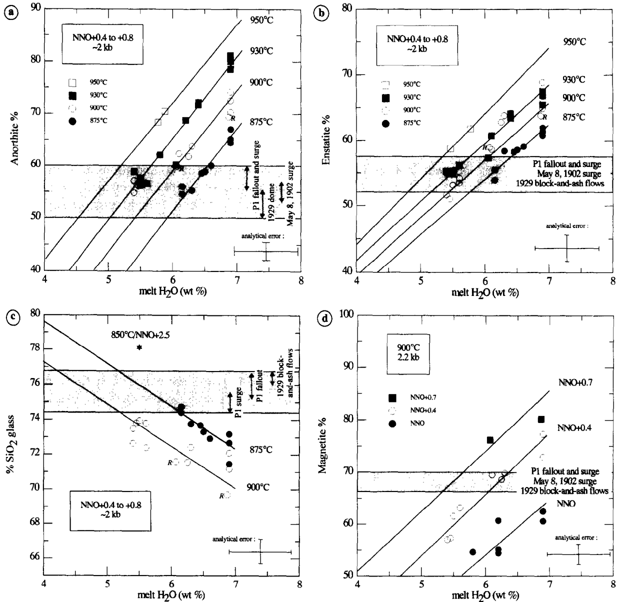
Fig. 2. Compositions of experimental plagioclase (a), orthopyroxene (b), glass (c) and magnetite (d) as a function of the H 2 O content of the glass, and comparison with natural compositions from recent eruptions. Each point represents either one analysis or the average of multiple analyses for a given phase in a given charge, with standard deviations ( 1\sigma ) equal or lower than analytical error. The data points are labelled as a function of experimental conditions, charges from different starting samples being represented under the same symbol. R denotes data from rapid-quench experiments. For plagioclase, only rim compositions are compared and, for glasses, only matrix glasses are used in the comparison (see text).
