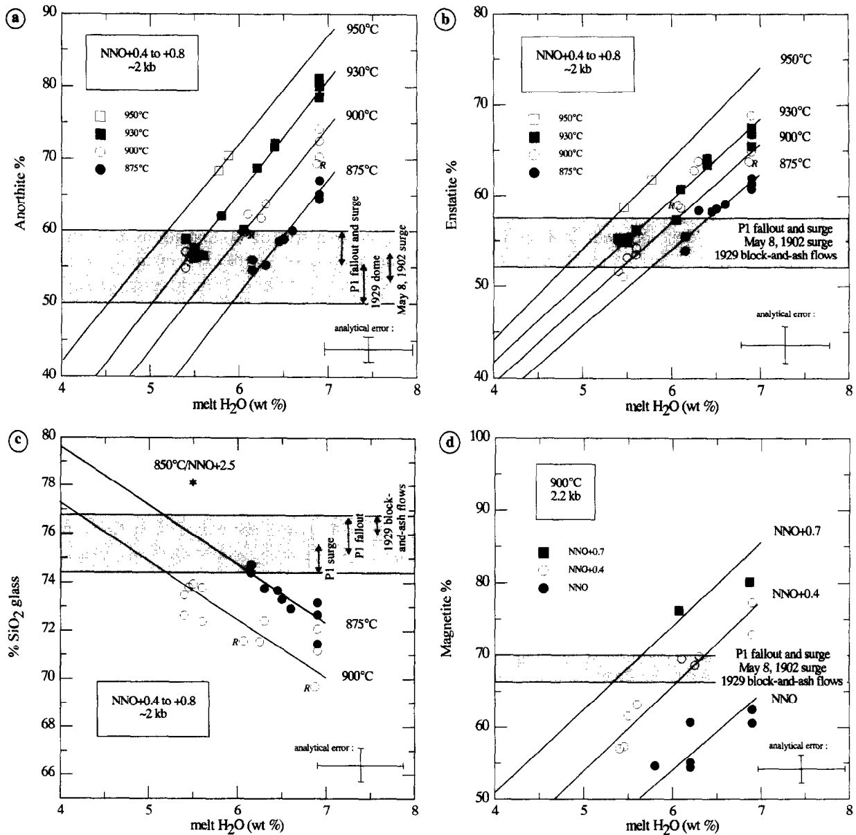
Fig. 2. Compositions of experimental plagioclase (a), orthopyroxene (b), glass (c) and magnetite (d) as a function of the H_2O content of the glass, and comparison with natural compositions from recent eruptions. Each point represents either one analysis or the average of multiple analyses for a given phase in a given charge, with standard deviations ( 1\sigma ) equal or lower than analytical error. The data points are labelled as a function of experimental conditions, charges from different starting samples being represented under the same symbol. R denotes data from rapid-quench experiments. For plagioclase, only rim compositions are compared and, for glasses, only matrix glasses are used in the comparison (see text).
