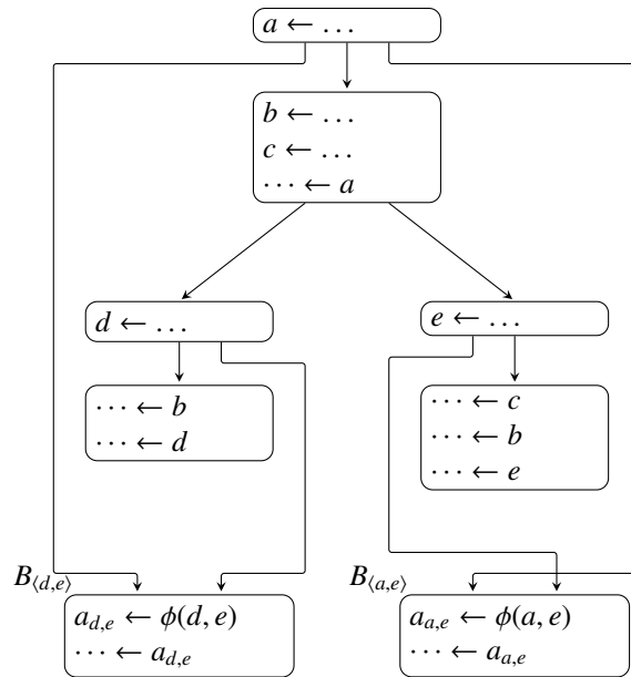
Figure 5.2: Chordal reduction with affinities: for any chordal graph and set of affinities there exists an SSA program.
