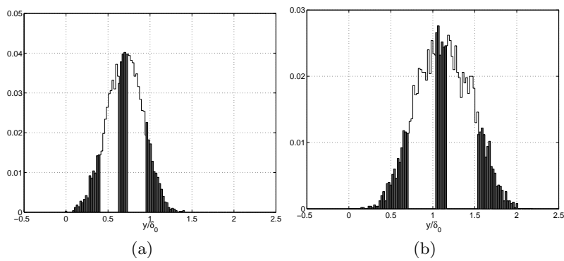
FIGURE 6. PDF of the instantaneous maximal elevation of the dividing stream line in the recirculating bubble, (a) \theta = 8^\circ , (b) \theta = 9.5^\circ
