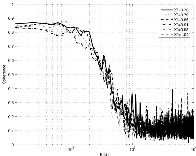
Fig. 14 Coherence function between wall pressure signals recorded in the vicinity of the reflected shock and near the reattachment region, \theta = 9, 5 deg, from [6,11].
