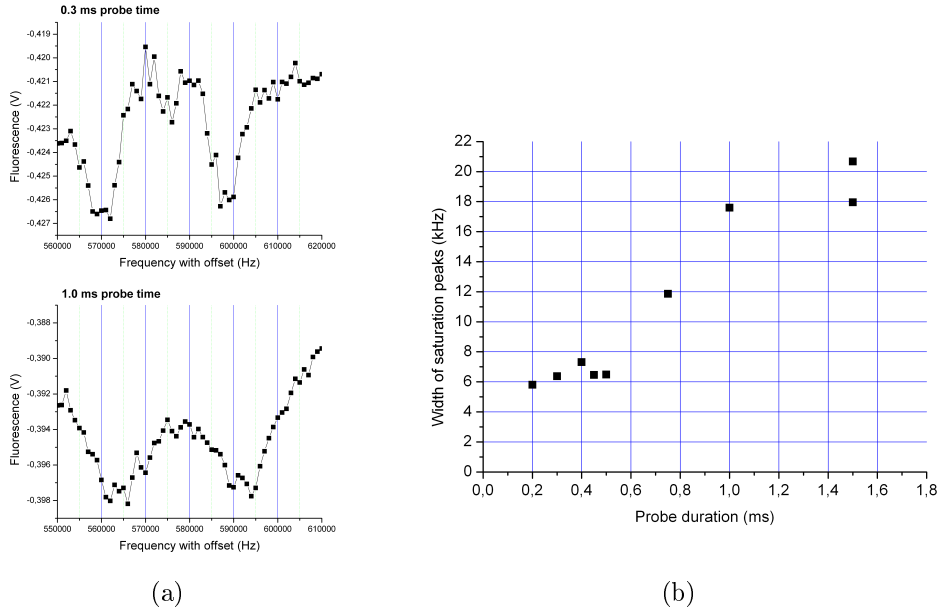
Figure 6.9: (a) The recoil doublets with respectively 0.3 ms and 1.0 ms of probe time. (b) The 1/e^2 width of the recoil peaks for different probe durations.
