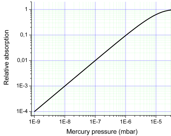
Figure 4.6: Calculated relative absorption of a (weak) beam of light at the ^{202}\text{Hg} cooling transition resonance as a function of the total mercury pressure.
