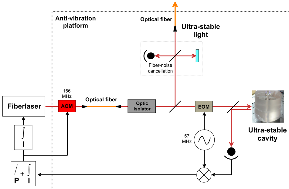
Figure 5.10: The Pound-Drever-Hall servo-loop used for locking the fiber laser to the ultra-stable cavity. Everything shown within the dotted border was placed on the anti-vibration platform.
