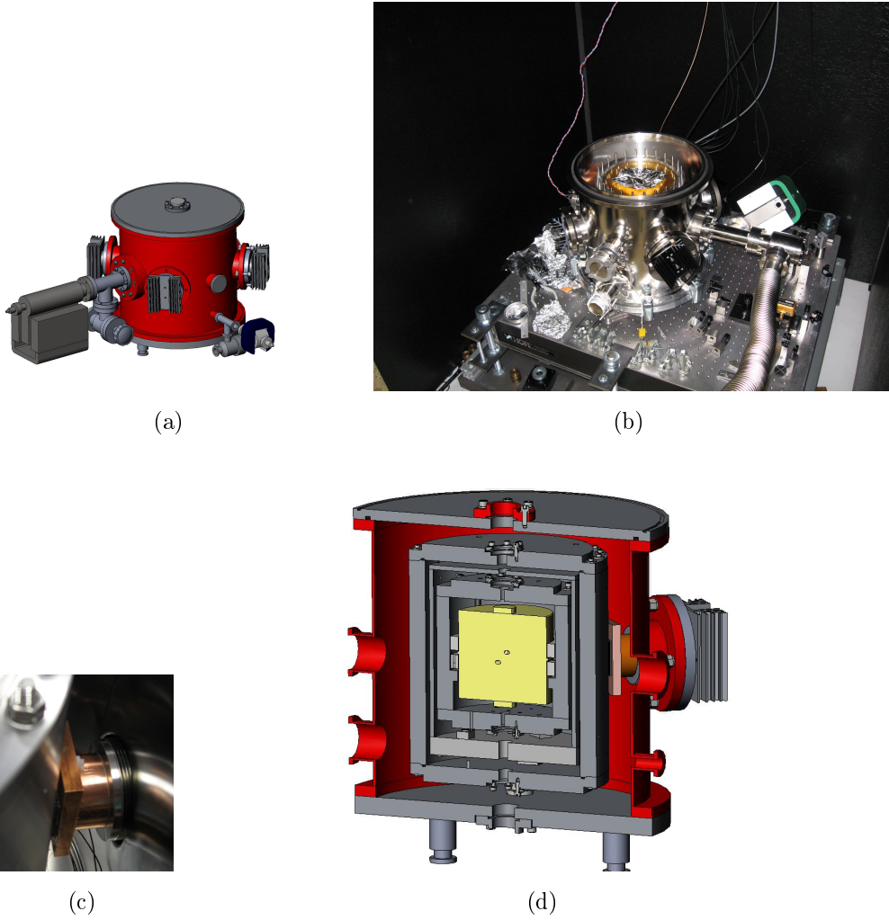
Figure 5.7: The thermo-mechanical setup around the ultra-stable cavity. (a) Diagram showing the exterior and the ion pumps. (b) Photo of the setup on the anti-vibration platform with the two top lids off. (c) Photo of the Peltier element and the heat tube used for temperature control of the inner vacuum chamber. (d) Cross section showing the interior of the vacuum chambers. The cavity is the yellow part.
