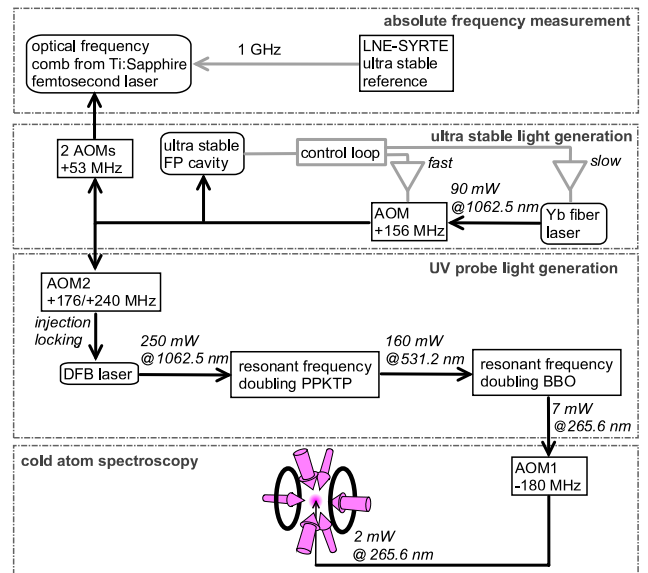
FIG. 2 (color online). Generation of the probe light at 265.6 \text{ nm} and referencing to the primary frequency reference. AOM2 frequency depends on the isotope.
