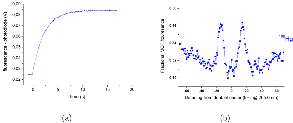
Figure 7.1: The major results presented in this thesis:(a) The loading of a ^{202}\text{Hg} MOT demonstrating the assembling of a neutral mercury MOT and (b) the ^{199}\text{Hg} recoil doublet of mercury in free fall, which allowed for the Doppler-free spectroscopy of the neutral mercury fermions.
