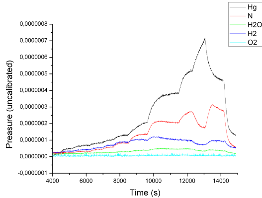
Figure 4.4: A mass spectrum analyzers measurement during a test of the mercury source in a smaller test chamber. These graphs shows the abundance of single isotopes. Due to the many mercury isotopes and the lesser efficiency of the measurements of heavier isotopes it is assumed that mercury is by far the most dominant atomic species. Near the peak of the mercury graph the spectrum analyzer is saturated by the mercury giving rise to the dip in the apparent abundance of the other atomic species.
