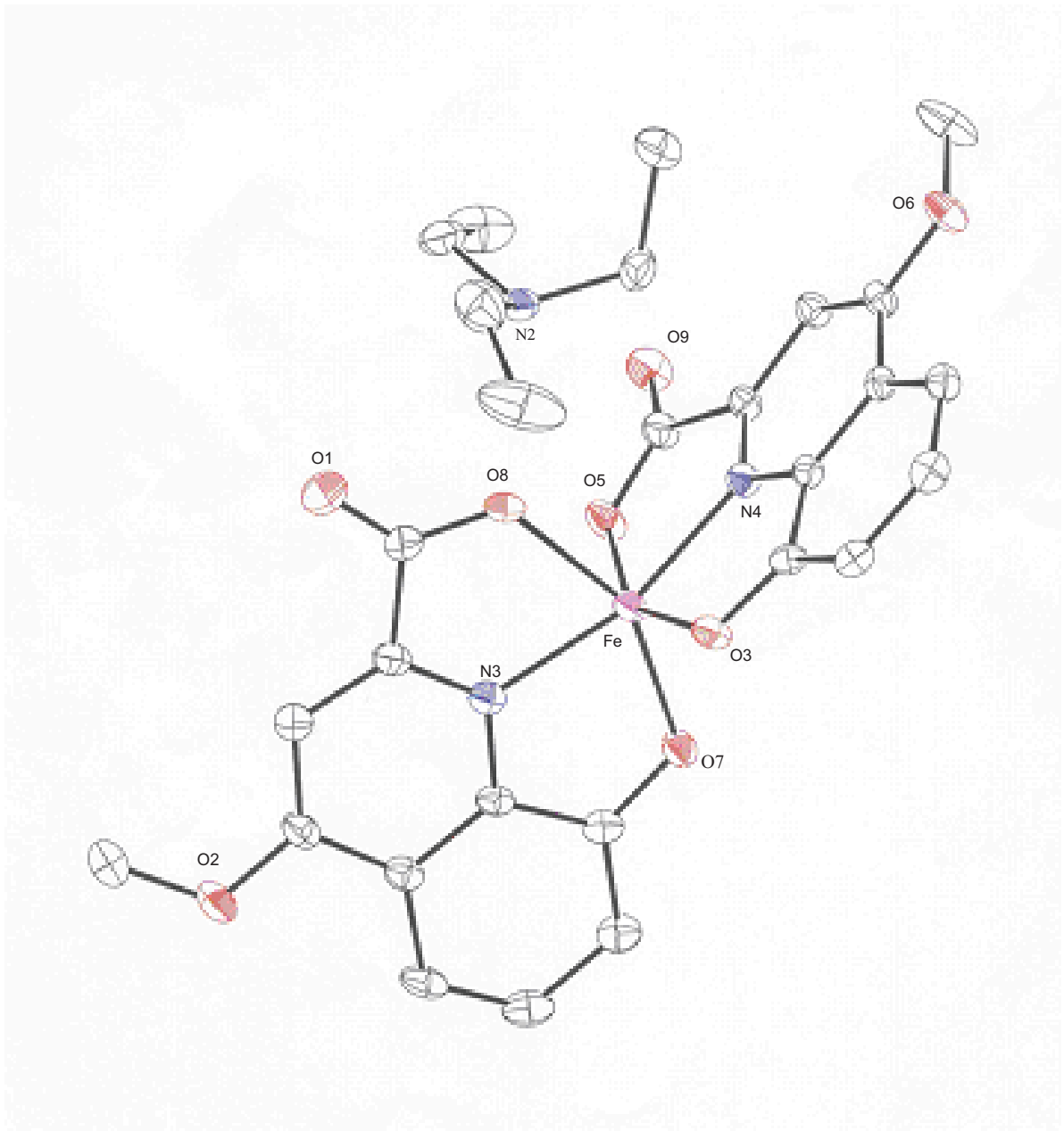
Figure 52 : RX de complexe [\text{Fe}(\text{Q})_2, \text{Et}_3\text{NH}] .
