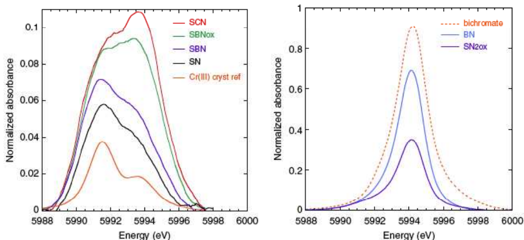
Fig. 3. (left) Extracted X-ray absorption near-edge structure pre-edge features of glasses with a very low or no Cr(VI) content, and Cr(III) crystalline reference. SBN2 is identical to SBN. (right) Extracted pre-edge features of glasses with a high Cr(VI) content. Note the difference in the relative intensity.
