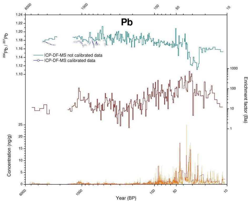
Figure 9.1 Pb concentration, enrichment factor and ^{206}\text{Pb}/^{207}\text{Pb} isotopic ratio profiles in Colle Gnifetti firn/ice samples.
