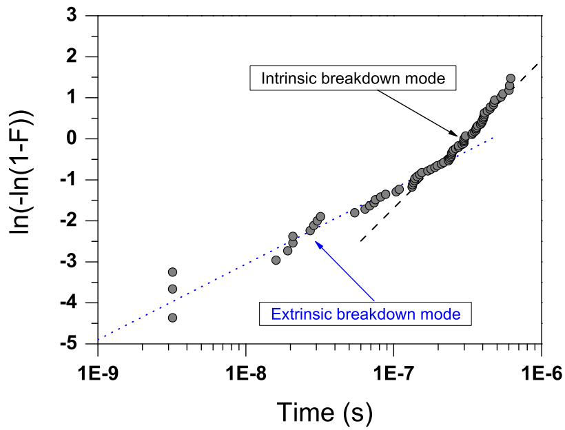
Figure 1.26: Bimodal cumulative failure distribution of an oxide stressed under CVS.
