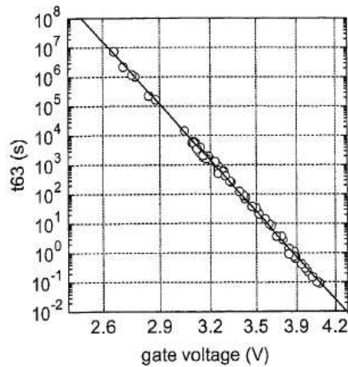
Figure 1.35: TDDB data plotted accordingly to the power law model after Pompl et al. [120].
