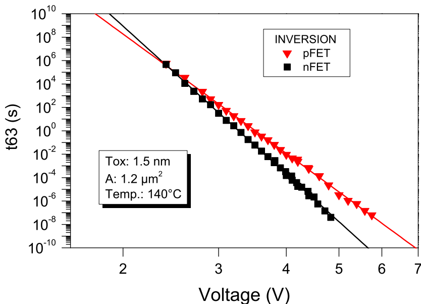
Figure 6.19: Voltage acceleration of 1.5 nm nFET and pFET stressed in inversion at 140 °C.
