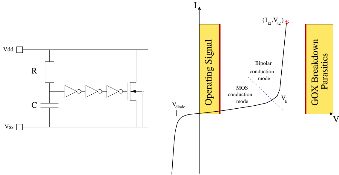
Figure 2.19: Left: protection concept based on a bigFET driver. Right: RC triggered nFET I-V characteristic showing first, the MOS current driving mode and then, the bipolar current regime after (V_{t1}-I_{t1}) .
