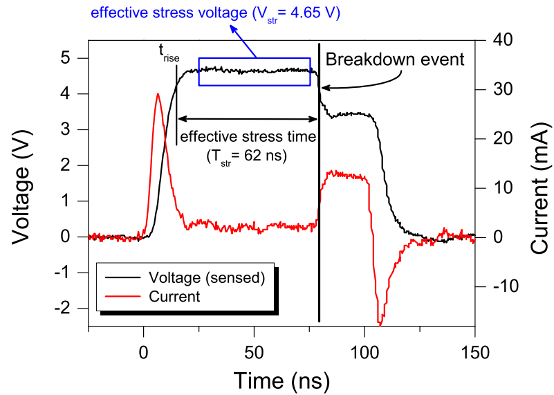
Figure 3.5: Pulse waveform for a 4.65 V stress, sensed at the gate. The detection of the breakdown event during the pulse is exposed for the determination of the effective time-to-breakdown ( T_{BD,eff} = 62 ns). The current spikes at the beginning and at the end of the pulse are artifacts due to reflections.
