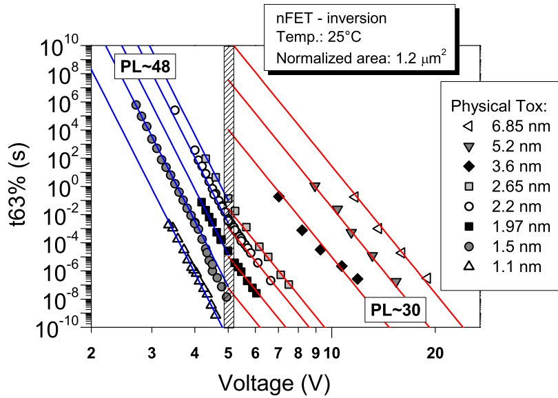
Figure 4.23: Voltage acceleration for nFET stressed in inversion regime at 25 °C normalized to the area of 1.2 μm 2 [51].
