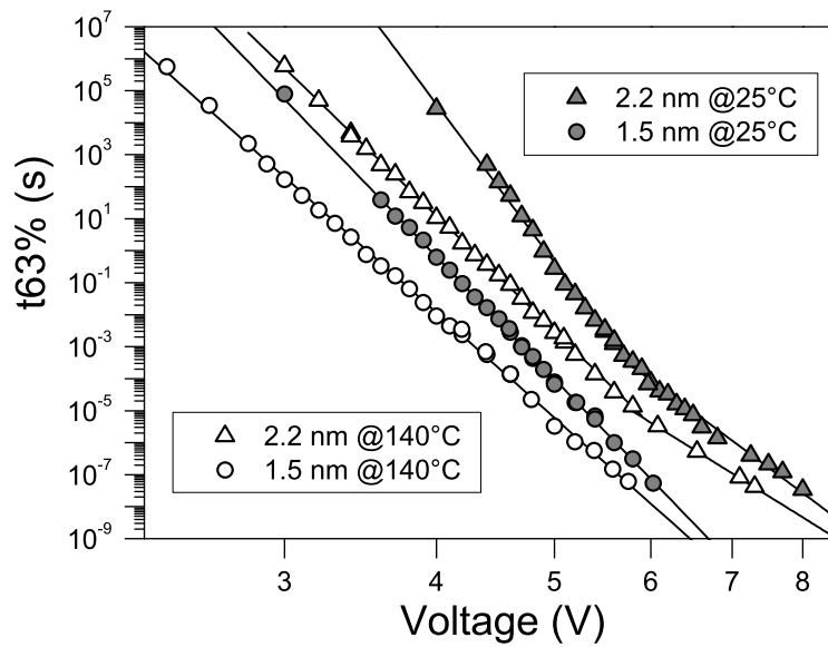
Figure 4.38: Voltage acceleration for the 1.5 nm, 2.2 nm pFET at 25^\circ\text{C} and 140^\circ\text{C} .
