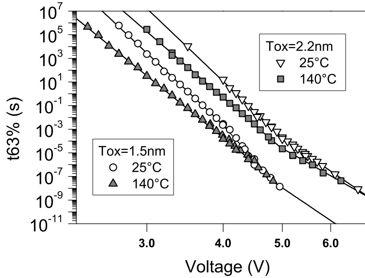
Figure 4.37: Voltage acceleration for the 1.5 nm, 2.2 nm nFET at 25^\circ\text{C} and 140^\circ\text{C} [23].
