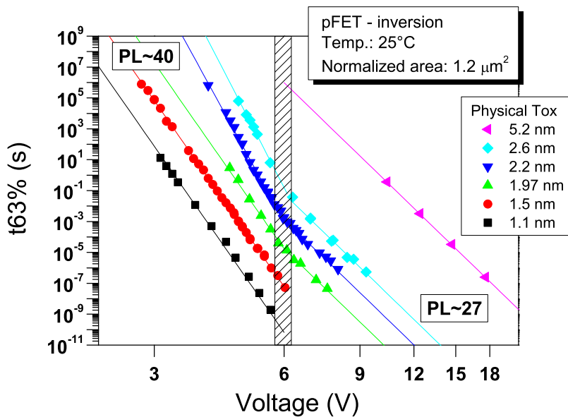
Figure 4.24: Voltage acceleration for pFET stressed in inversion regime at 25 °C normalized to the area of 1.2 μm 2 .
