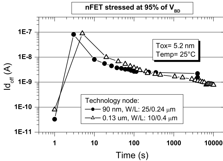
Figure 5.10: Characteristic recovery effect in time at room temperature from stressed devices by a 100 ns pulse stress [39].
