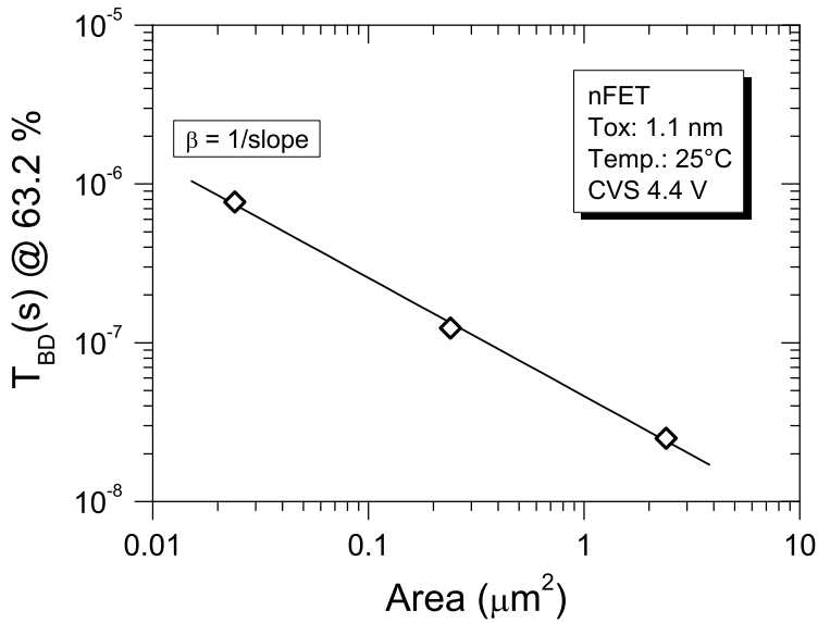
Figure 4.11: The extracted T_{63\%} obtained from the 4.4 V CVS (Figure 4.10) are plotted as a function of the GOX area.
