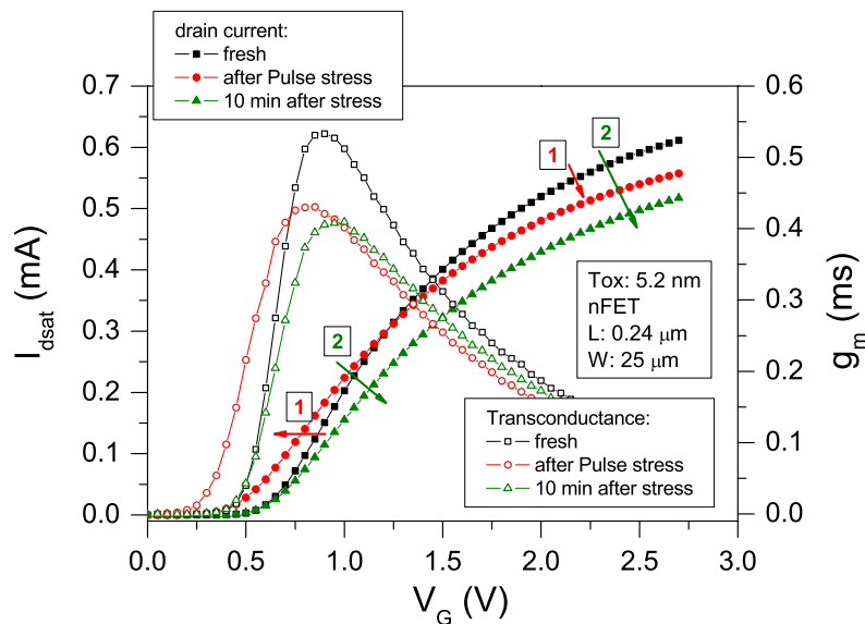
Figure 5.7: Saturated drain current from an 5.2 nm nFET after an 100 ns pulse stress at 90 % of the breakdown voltage. In a first step (1), a threshold voltage ( V_{th} ) reduction due to unstable positive charges occurs, then in a second phase (2) the degraded characteristic is dominated by a net negative trapping (increased V_{th} and I_{on} reduction) [39].
