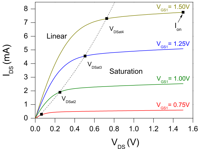
Figure 1.11: The MOS drain current versus the drain voltage is exposed for different gate biasing for an 2.2 nm nFET with L_g = 0.18 \mu\text{m} and W_g = 20\mu\text{m} .
