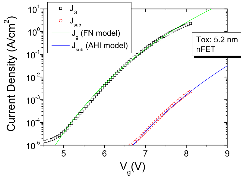
Figure 1.19: Gate and substrate leakage of an 5.2 nm nFET. Gate current is modeled with the Fowler-Nordheim Tunneling equation and the substrate current accordingly to the AHI model.
