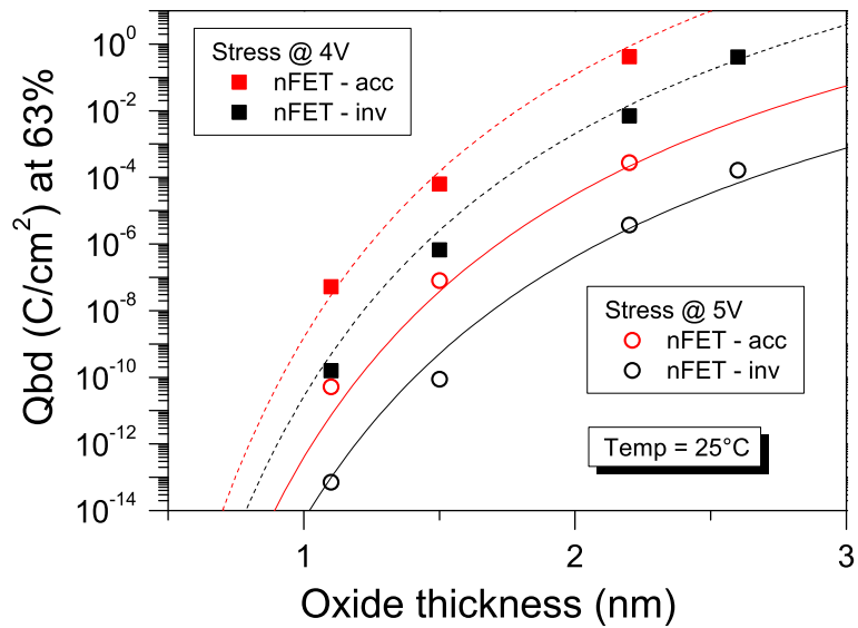
Figure 4.55: Charge to breakdown ( Q_{BD} ) of nFET devices as a function of the oxide thickness for two selected voltages under the TDDB acceleration voltage kink.
