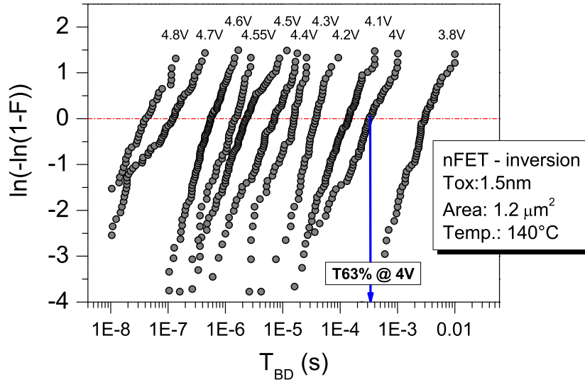
Figure 4.18: Gate oxide time to breakdown distribution of 1.5 nm nFET devices at 140^\circ\text{C} for CVS measurements from 3.8 V to 4.8 V using the set-up exposed in Section 3.2.3 [23].
