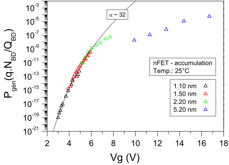
Figure 4.54: Gate voltage dependence of the defect generation probability ( P_g ) for nFET stressed in accumulation at room temperature and based on a_0 = 1.83 nm and T_{int} = 0.37 nm.
