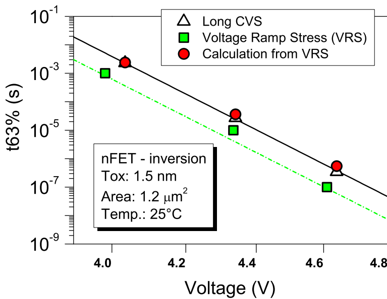
Figure 4.16: TDDB data at 25 °C obtained by long CVS and VRS. The T_{63\%} from the transformed VRS distributions are also plotted (circles) [23].
