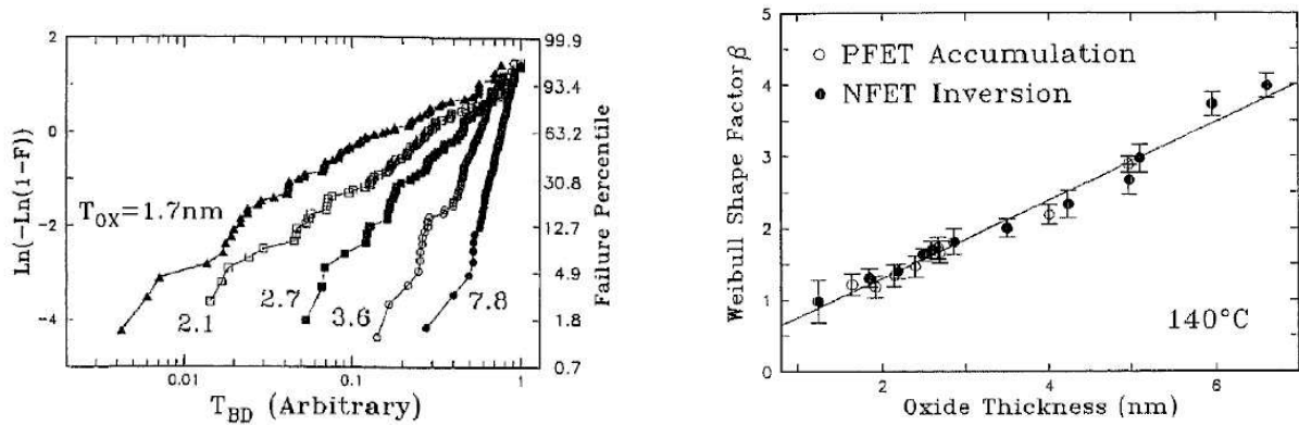
Figure 1.27: Weibull slope dependence with the oxide thickness after Wu et al. [86], data at 140 °C.
