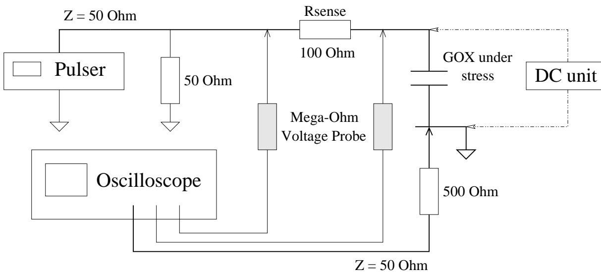
Figure 3.1: Set-up configuration used for the gate oxide time dependent dielectric breakdown experiments
