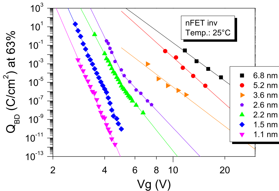
Figure 4.48: Charge to breakdown of nFET devices stressed in inversion at room temperature.
