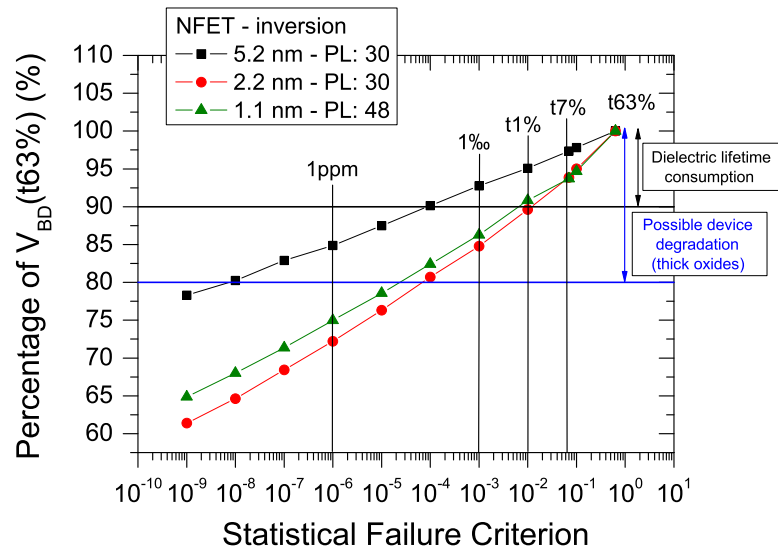
Figure 6.12: Correlation between the statistical failure criteria and the percentage of the breakdown voltage ( V_{bd} ) for nFET stressed in inversion. Three oxide thicknesses are considered (1.1 nm, 2.2 nm, 5.2 nm) [9].
