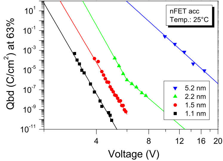
Figure 4.49: Charge to breakdown of nFET devices stressed in accumulation at room temperature.
