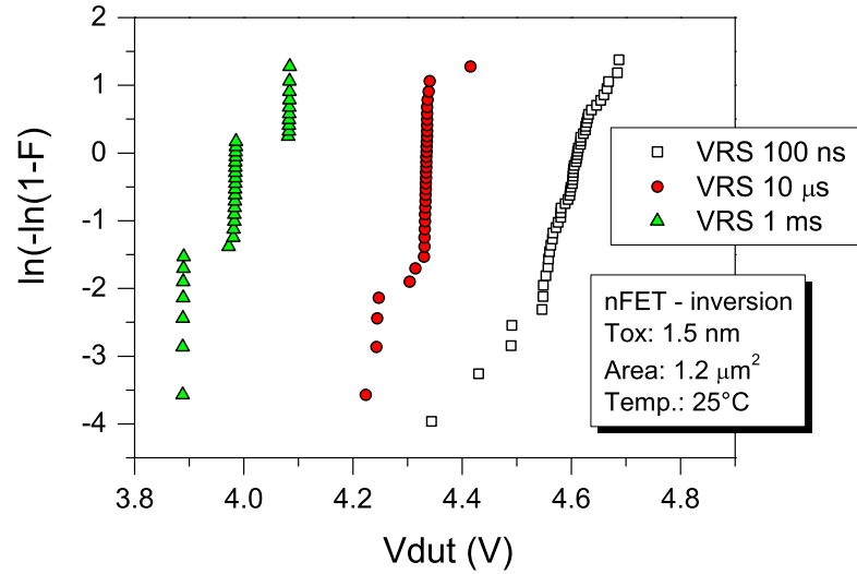
Figure 4.14: Breakdown voltage distributions of 1.5 nm nFET obtained from VRS for three different pulse-width, 100 ns, 10 μs and 1 ms
