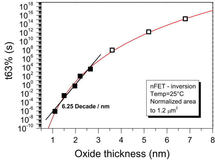
Figure 4.35: TDDB cross section from Figure 4.23 at 4 V showing the acceleration factor from the GOX time to fail as a function of the oxide thickness [51].
