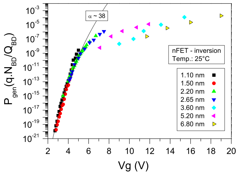
Figure 4.53: Gate voltage dependence of the defect generation probability ( P_g ) for nFET stressed in inversion at room temperature and based on a_0 = 1.83 nm and T_{int} = 0.37 nm.
