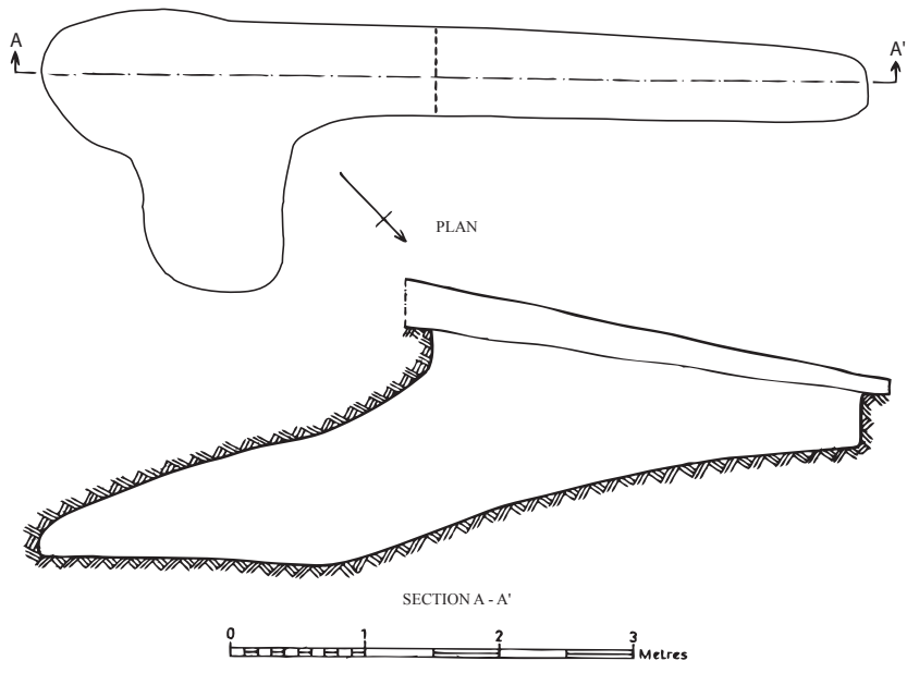
GASTRIA : "Alaas" TOMB 11
