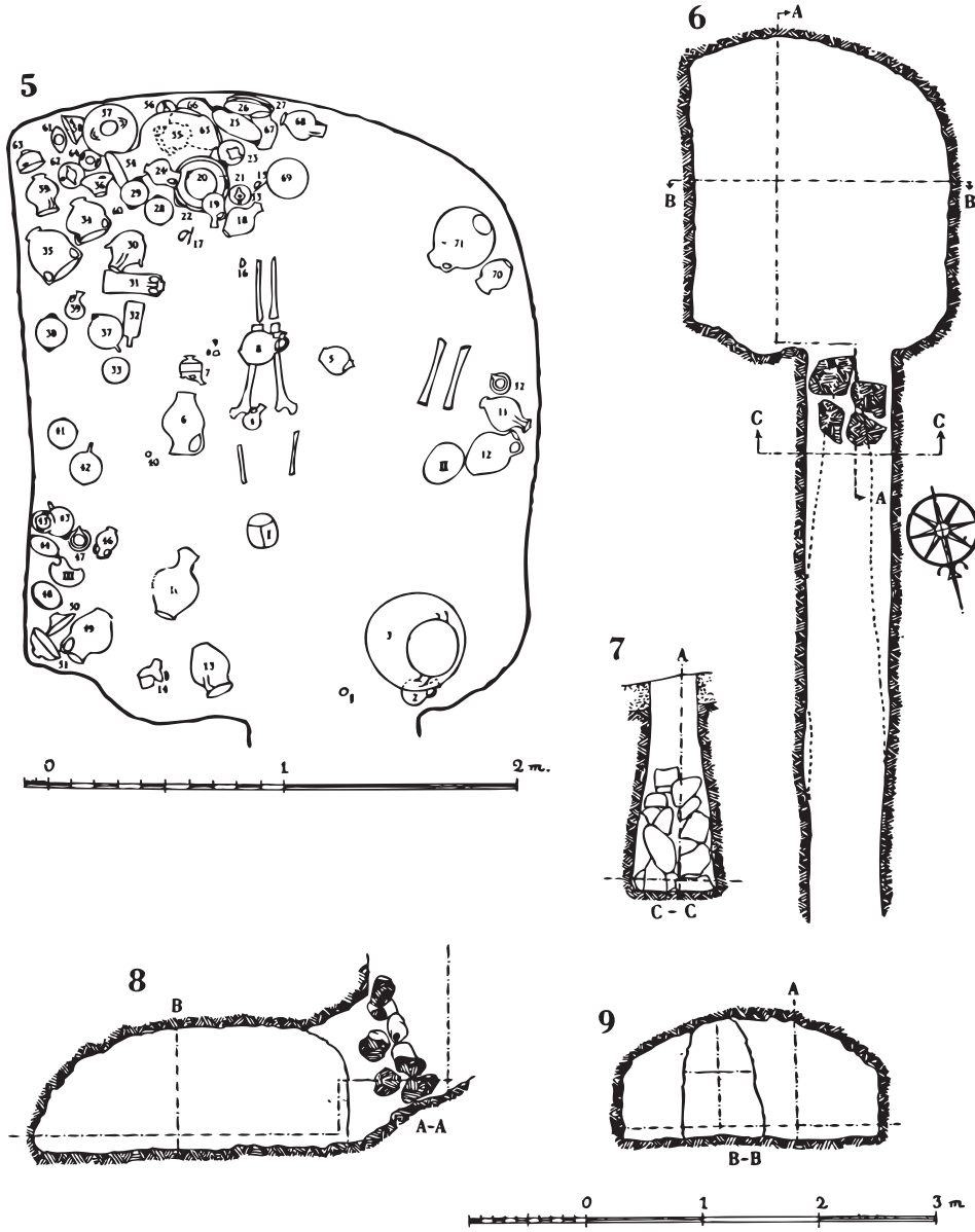
Fig. 72. Lapithos. Tombs 404 - 405, Plan (I); Sections A-A and B-B (2-3); Finds in situ (4). Tomb 4c6, Finds in situ (5); Plan (6); Sections C-C, A-A, B-B (7-9)
