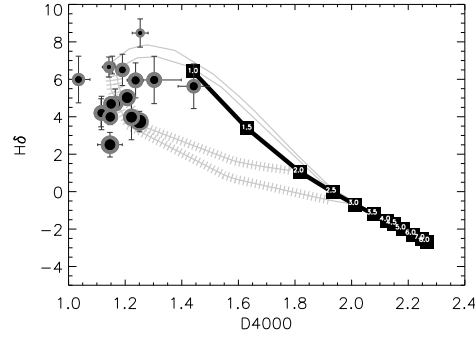
Fig. 13. The lines are the same as in Fig. 7 and in Fig. 8. The black circles are proportional to t_{20} defined before, while the grey one to t_{50} .
