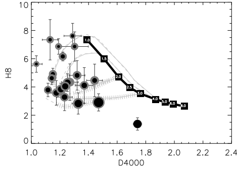
Fig. 12. The lines are the same as in Fig. 7 and in Fig. 8. The black circles are proportional to t_{20} defined before, while the grey one to t_{50} .
