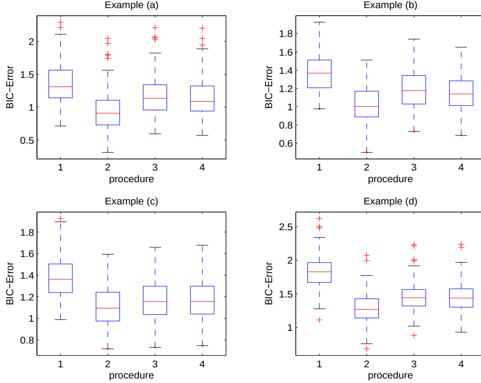
Figure 3.1: BIC error in each example. For each plot, we construct the boxplot for the procedure 1 = Lasso; 2 = Elastic-Net; 3 = NS-Lasso; 4 = HS-Lasso
