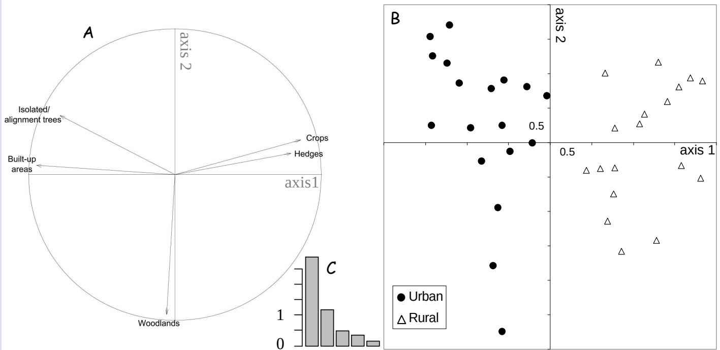
Figure 2: Results of the principal components analysis on the environmental matrix R. A: Scatter diagram of the correlation circle. B: position of sites on first factorial map with the distinction on the first axis of sites which will be considered as urban (black dots) and rural (white triangles). The eigenvalue barplot is provided at the lower left-hand corner
