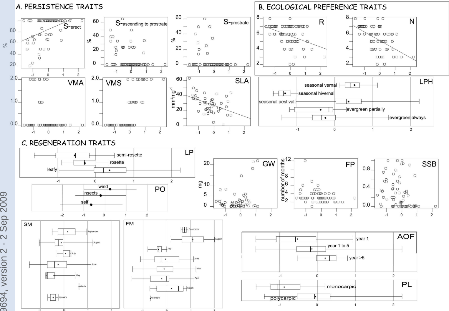
Figure 8: Synthesis of biological traits which are significantly associated with the first ordination axis of the RLQ analysis. For each graph, the left part of the abscise axis were associated with the urban woodlands, the right with the rural woodlands. For quantitative and ordinal variables, we displayed a graph of the correlation between the score of the species along the first axis of the RLQ and the values of the biological traits for each species. For circular, nominal and multichoice variables, we displayed a boxplot of the scores of the species along the first axis of the RLQ analysis belonging to each group. The box indicates the boundaries of the first (left) and third (right) quartiles; the line in the box indicate median position and the dot position of the mean. The whiskers indicate min value (left) and max values (right). For fuzzy variables, we displayed the mean (dot) and the standard deviations (whisker) of each modality of the variable. See Table I for codes of traits.
