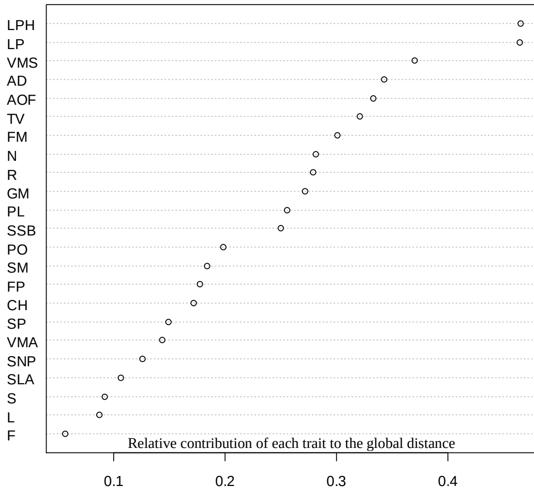
Figure 3: Contribution of each variable to the global distance obtained by Eq. 1 and displayed by a Cleveland's (1994) dot plot. Abbreviates of plant traits are given in Table I.
