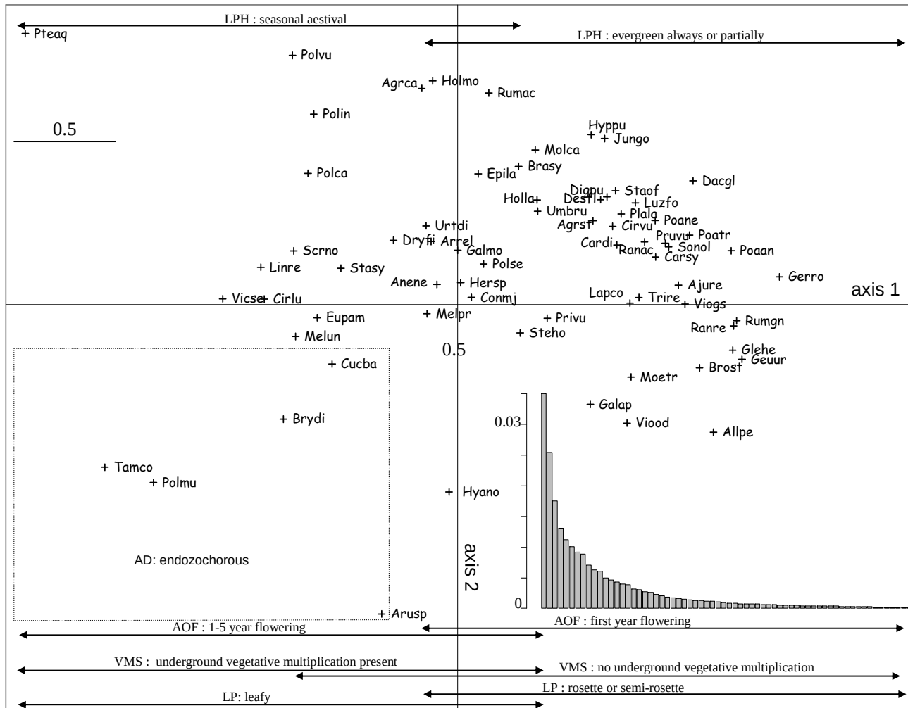
Figure 5: Principal coordinate analysis (PCoA) applied to the global distances among species. Axis 1 (horizontal) expresses 16% of the variation and axis 2 (vertical) expresses 12% of the variation. The eigenvalue barplot is provided at the lower right-hand corner of the factorial map. The labels of the species are given by codes; full Latin names are given in Appendix 2. Some of the variables or levels of variables have been added to the graph to help the interpretation. The variables are associated with arrows indicating tendencies of separations of the species according to the first or second axis. The dashed indicate the distinction between endozoochorous and other species. The scale is given in the top left-hand corner of the map.
