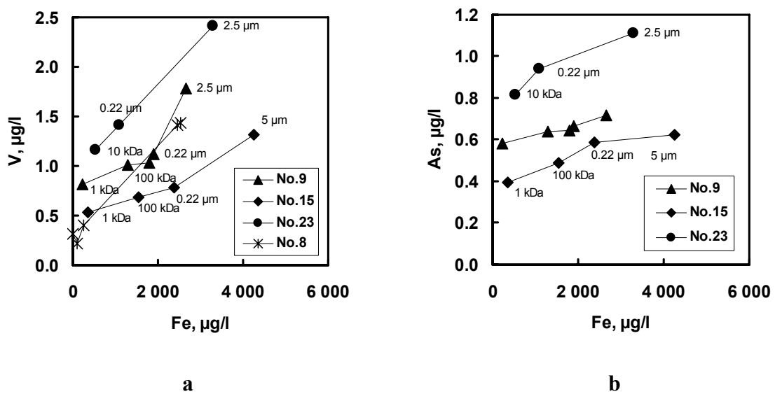
Fig. 3.17. V (a) and As (b) concentration as a function of Fe concentration in successive filtrates from 5 \mu\text{m} to 1-10 kDa.
