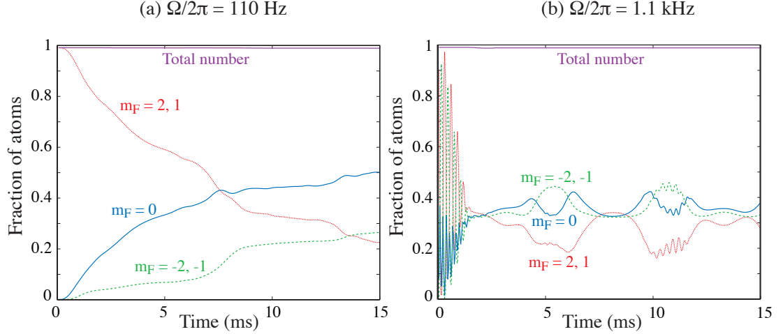
Figure 5.5: Comparison of the population dynamics in the five-state system for (a) weak and (b) strong coupling. Parameters are N = 5 \times 10^4 atoms, \omega_z = 2\pi \times \frac{260}{\sqrt{2}} \text{ Hz} , U = 6.6 \times 10^{-4} , G = 9.24 , and \Delta = 10.7 .
