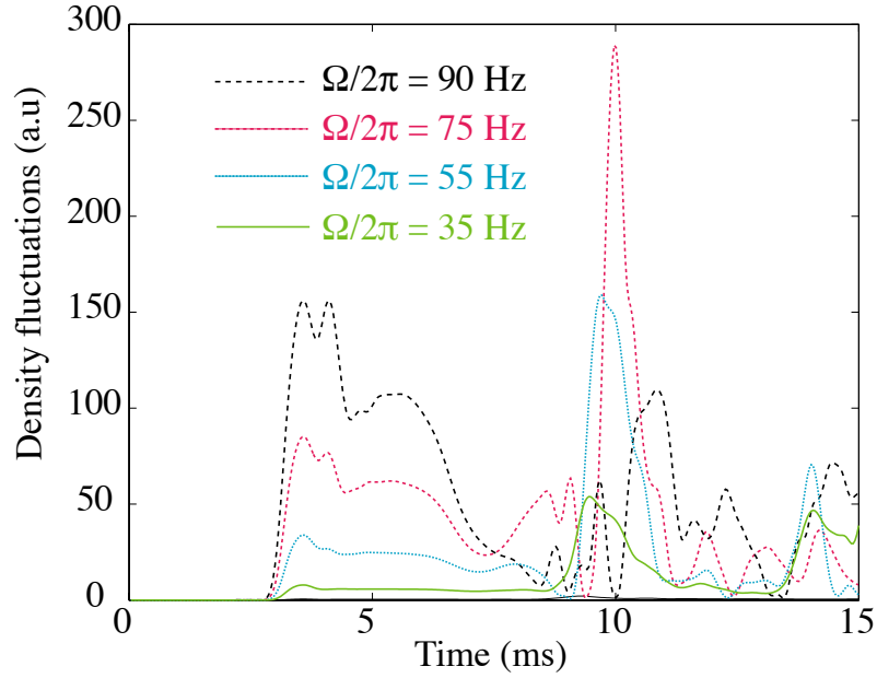
Figure 5.11: Density fluctuations in the m_F = 0 state of a five-state system at a single point in the beam as a function of time. The fluctuations due to the sloshing of the m_F = 1 are increasingly severe as the coupling strength is increased. Parameters are N = 5 \times 10^4 atoms, \omega_z = 2\pi \times \frac{260}{\sqrt{2}} Hz, U = 6.6 \times 10^{-4} , G = 9.24 , and \Delta = 10.7 .
