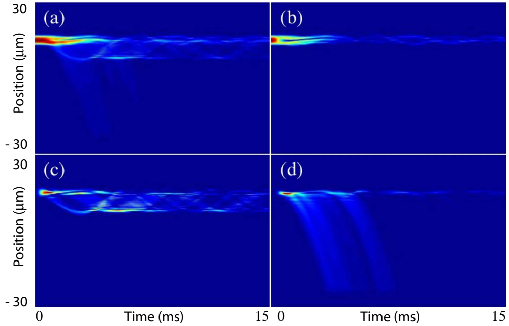
Figure 5.8: Spatial profiles of the five-state system after 15 ms of weak ( \Omega/2\pi = 200 Hz) output coupling. Each plot shows the atomic density of atoms with the complete spatial grid in the vertical direction and the temporal grid in the horizontal direction. (a) Represents the total density, i.e. the sum of the densities in all five Zeeman states, as a function of time. (b) Is the density of the m_F = 2 state, (c) m_F = 1 and (d) m_F = 0 . The color axes are adjusted to give the best contrast for each of the Zeeman states. N = 5 \times 10^4 atoms, \omega_z = 2\pi \times \frac{260}{\sqrt{2}} Hz, U = 6.6 \times 10^{-4} , G = 9.24 , and \Delta = 10.7 .
