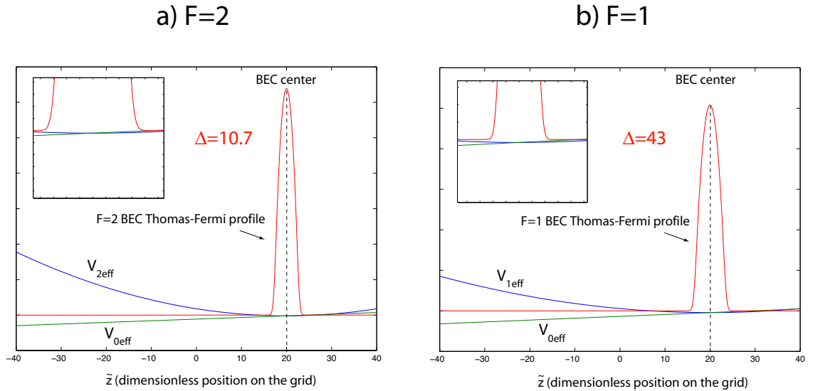
Figure 5.1: Thomas-Fermi profile of the BEC and effective potentials experienced by the atoms for the F = 2 state (a) and F = 1 state (b) where the detunings have been set to 10.7 and 43 respectively in order for the out-coupling resonance to be at the center of the BEC. N = 5 \times 10^4 atoms.
