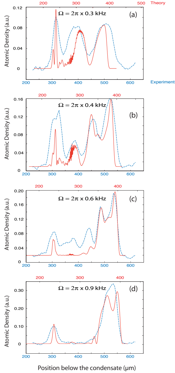
Figure 5.3: Comparison of theoretical (solid lines) and experimental (dashed lines) results showing the spatial structure of an atom laser (atoms in the m_F = 0 state) for various Rabi frequencies. The theoretical simulations were performed with 2.6 ms of RF out-coupling followed by a 6 ms free fall. The experimental data were obtained after 3 ms of RF out-coupling and again a free evolution of 6 ms. Important parameters are : N = 5 \times 10^4 atoms, \omega_z = 2\pi \times \frac{260}{\sqrt{2}} \text{ Hz} , \omega_y = 2\pi \times \frac{20}{\sqrt{2}} \text{ Hz} , \Delta = 10.7 and U = 6.6 \times 10^{-4} .
