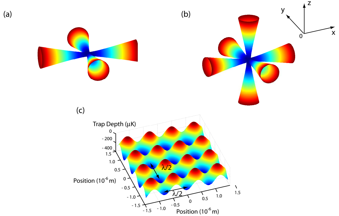
Figure 8.2: a) Shows two orthogonal pairs of retro-reflected Gaussian beams which create the 2 dimensional standing wave represented in c). b) Shows a third orthogonal pair of retro-reflected laser beams. In this case, the resulting 3D confinement has a cubic geometry and is analogous to electrons in a crystal lattice.
