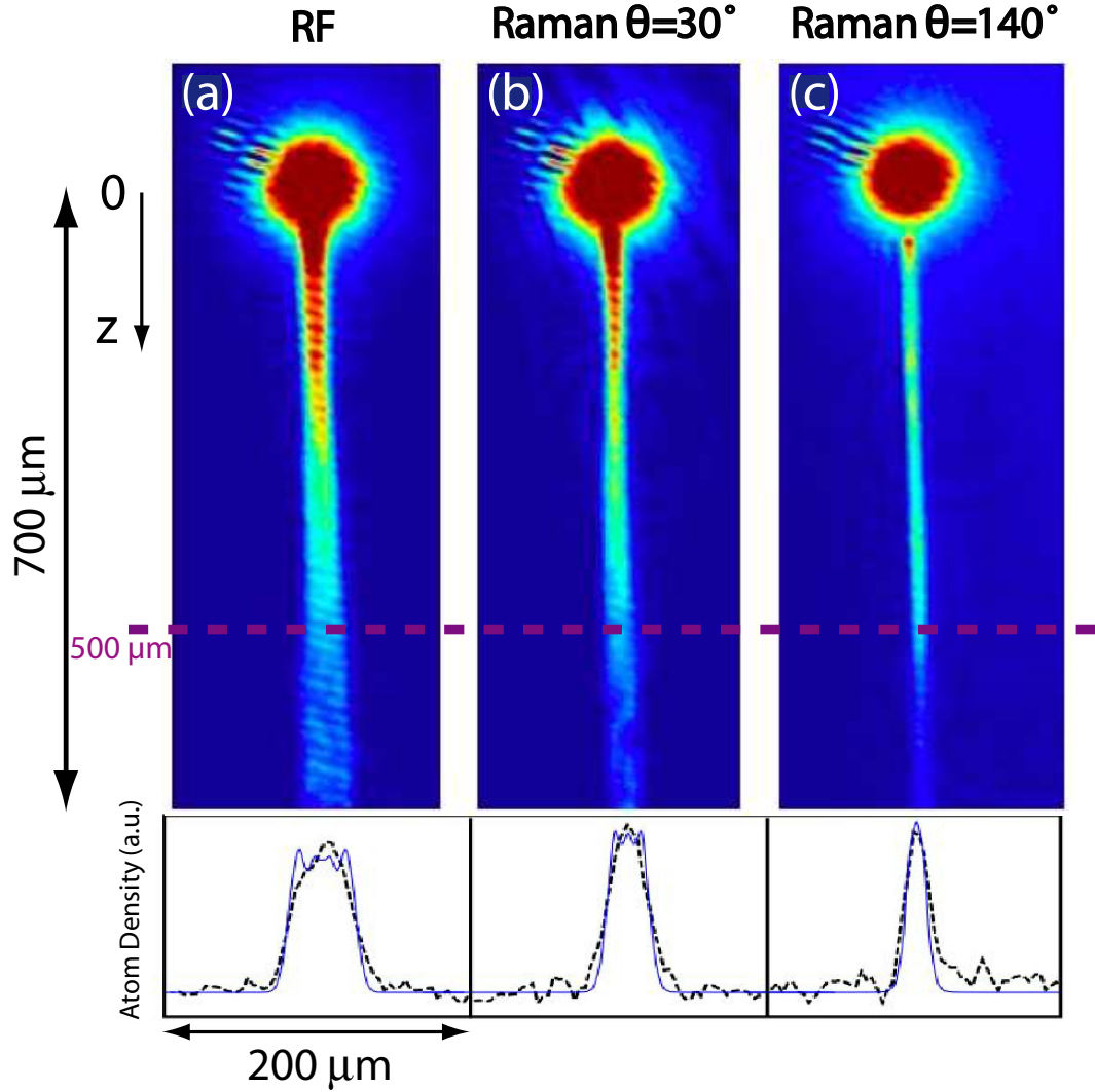
Figure 3.2: The top images show a sequence of atom laser beams produced using RF (a) and Raman (b and c) transitions with the out-coupling cut set at the center of the BEC and imaged after a 3 ms time-of-flight. The angle between the Raman beams was \theta = 30^\circ in (b) and \theta = 140^\circ in (c), corresponding to momentum kicks of 0.5 \hbar k ( 0.3 \text{ cm.s}^{-1} ) and 1.9 \hbar k ( 1.1 \text{ cm.s}^{-1} ) respectively. The out-coupling rate differs between each atom laser and the time-off-flight was set to approximately 3 ms. One can see the improved beam profile of a Raman atom laser. Note that the fringes that can be observed in the condensates are an imaging artifact due to interferences on the CCD cover plate. The bottom plots show a comparison of experimental (dashed) and theoretical (solid) beam profiles at a distance 500 \mu\text{m} below the BEC (indicated by the horizontal dashed line). The heights have been normalized and each theoretical curve has been scaled to match the experimental data.
