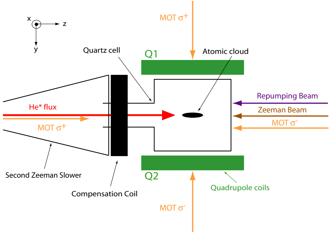
Figure 6.11: Schematics of the MOT. The 6 optical MOT beams (only 4 are visible in the plane of the figure) intersect at the center of the quartz cell. The Zeeman and repumping beams are also shown. The quadrupolar magnetic field is created by the two coils Q_1 and Q_2 .
