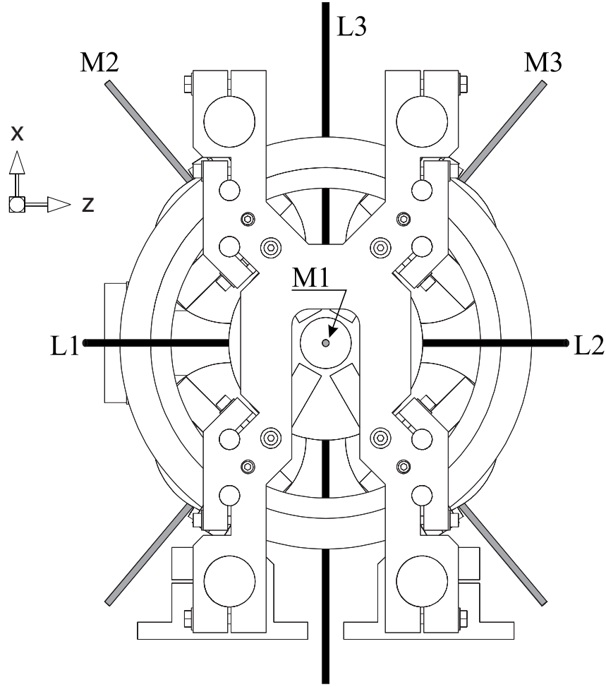
Figure 8.5: View of the mechanical support structure from the positive Y -direction. The 4 support rods are spaced by 270 mm in the X -direction, and 113 mm in the Z -direction.
