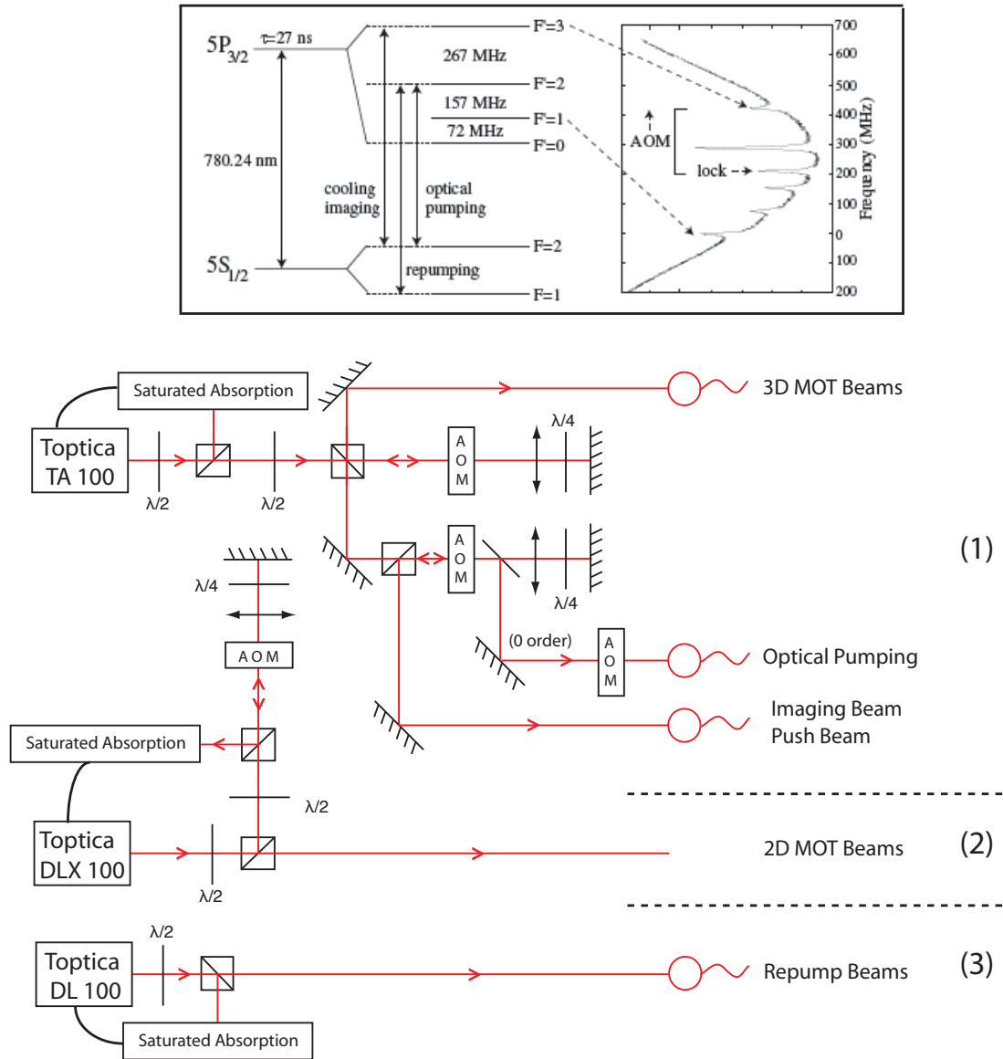
Figure 2.4: Laser system. The top pictures show the spectroscopy relevant to the experiment, together with a theoretical plot of the saturated absorption spectrum which is used to lock the light frequency. The bottom diagram represents the optical setup used to produce the beams to cool, pump, image, and push the atoms.
