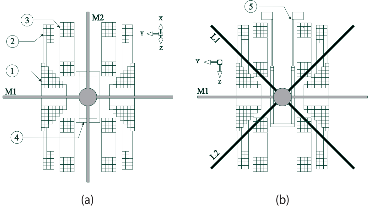
Figure 8.4: Winding configuration of the pinch coils (No. 1), compensation coils (No. 2) and cloverleaf coils (No. 3). a) is a view of a cross section in a plane resulting from a rotation of the YZ -plane by 45^\circ around the Y -axis (see figure 8.3). The grey circle (a sphere of 30 mm diameter) is the largest volume that can be occupied by an atomic cloud trapped in the MOT inside the glass cell (No. 4). b) is a similar view of a cross section in the YZ -plane where No.5 is the DN40CF-flange, connected to the UHV-glass cell by a metal-glass joint.
