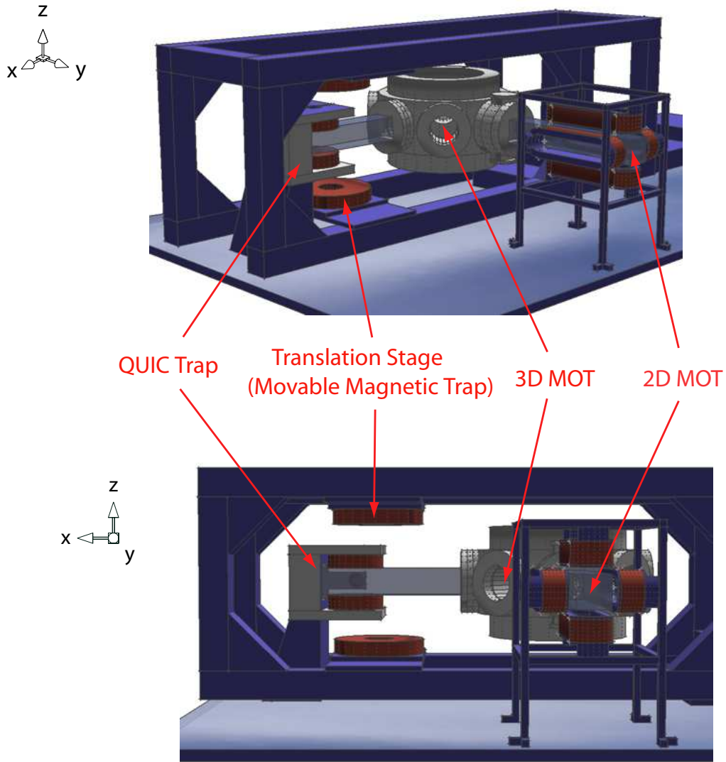
Figure 2.2: Experimental machine used to produce the Bose-Einstein condensate. Optical laser beams are not shown. The 2D MOT cools the atoms from room temperature in both transverse directions. The 3D MOT is loaded in an ultra-high vacuum from the 2D MOT by a near-resonance laser push beam. The 3D MOT coils are mounted on a translation stage. They not only provide confinement for the 3D MOT stage but they are also used to transport the atoms across to the QUIC trap where they are transferred and condensed after evaporative cooling.
