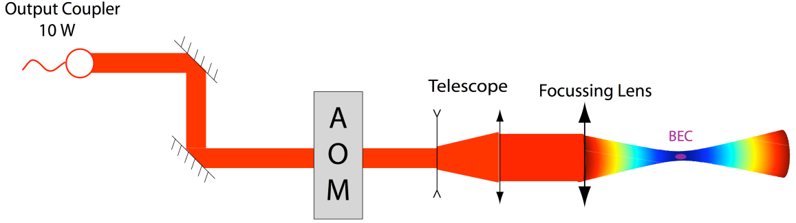
Figure 7.6: Creation of a focussed Gaussian beam. The output beam of the laser amplifier passes through an AOM which can switch the light on and off and change its central frequency. Finally, the beam is expanded before being focussed onto the BEC down to a waist of \sim 100 \mu\text{m} .
