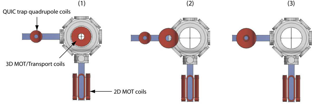
Figure 2.8: Transport of the magnetically trapped atoms by a translation stage. The quadrupole coils, initially above the Collection chamber (1), are moved across the frame (2) to the far end of the BEC chamber (3).
