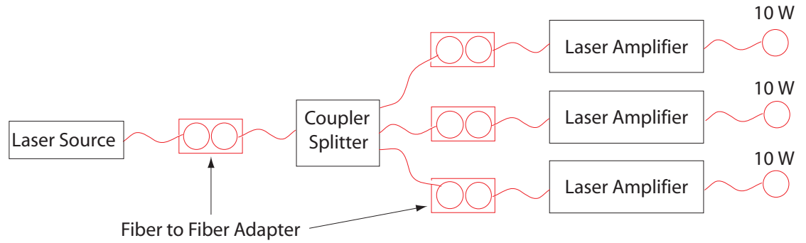
Figure 7.5: Schematic of the experimental layout of the laser system used to produce 1-, 2- or 3-D lattice traps. The laser source is split into three outputs. Each laser amplifier provides a total power of 10 W at 1560 nm.
