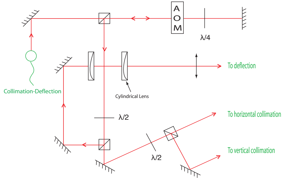
Figure 6.7: Schematic of the optical setup used to create the laser beams for collimation and deflection. These beams are on resonance with the 2^3S_1 \rightarrow 2^3P_2 atomic transition.
