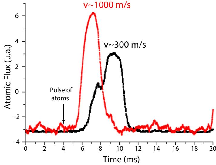
Figure 6.10: Effect of the first Zeeman slower on the atoms, measured using the channeltron. In red is the atomic signal without Zeeman slowing whereas the black curve corresponds to an atomic jet which has experienced longitudinal cooling. The shoulder of the black curve represents a fraction of atoms which do not experience the slowing effect and cannot be trapped in the MOT.
