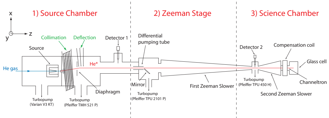
Figure 6.2: Experimental setup. The vacuum system is segmented into 3 parts: 1) the Source Chamber, 2) the Zeeman slower Stage and 3) the Science Chamber. The metastable helium beam is successively collimated, deflected, decelerated and trapped, in the Science Chamber, a 5\text{cm} \times 5\text{cm} \times 4\text{cm} quartz cell.
