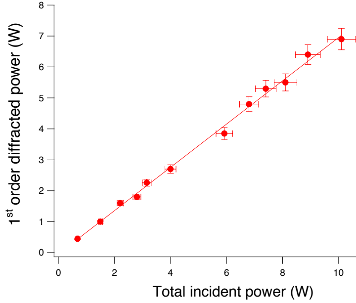
Figure 7.8: First order efficiency of the acousto-optic modulators. The input power is increased from minimum to maximum value and compared to the output power diffracted in the first order. 10% error bars are considered to account for experimental uncertainties.
