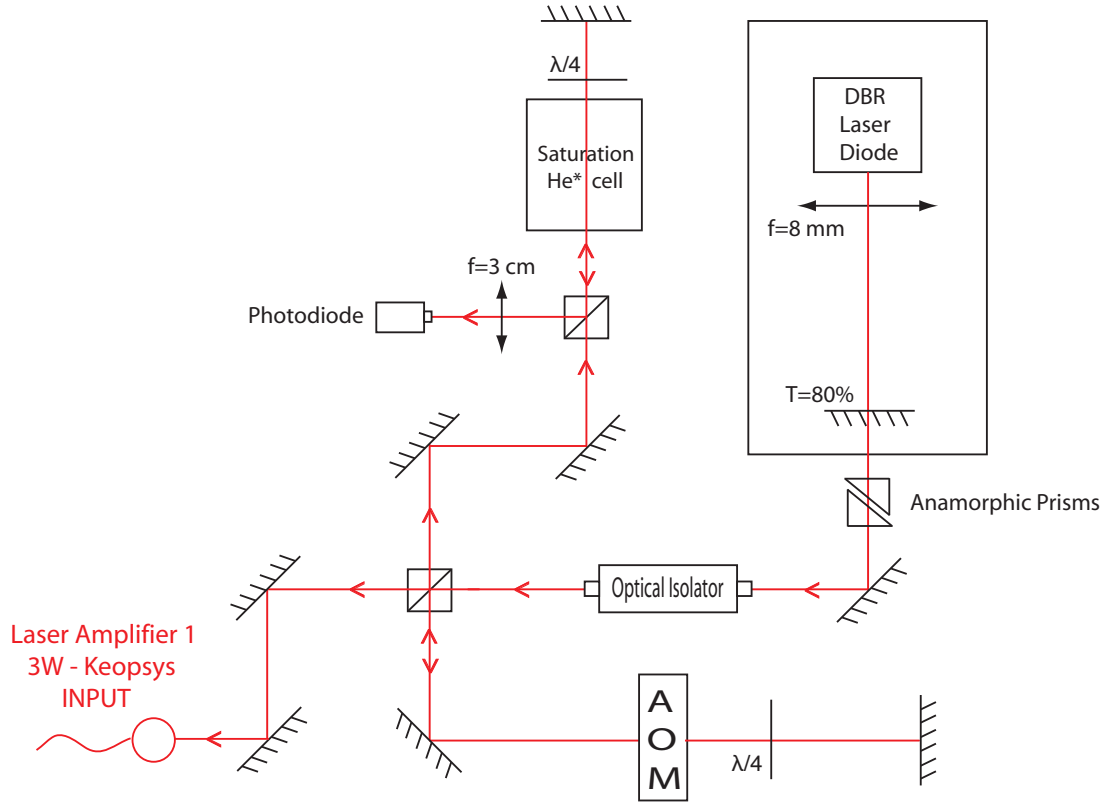
Figure 6.3: Schematic of the laser diode setup. The beam frequency is locked -240 MHz away from the 2^3S_1 \rightarrow 2^3P_2 atomic transition by saturated absorption and is used as a seed to be amplified by a 3 W laser-amplifier.
