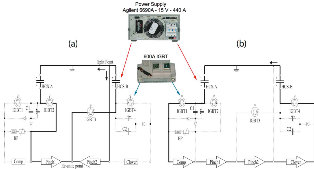
Figure 8.7: Schematics of the coil wiring circuit. HCS-A and HCS-B are two high current power supplies that can be programmed independently. The thick lines indicate the path followed by the current in either the MOT configuration a) or the magnetic trap configuration b). The current route is controlled by adjusting the control voltage of four IGBTs. Capacitors C1 and C2 can absorb the magnetic field energy thus reducing the voltage spikes during the switching off. The bypass circuit BP allows for a controllable drain of current from the compensation coils in order to adjust the level of the bias field B_0 .
