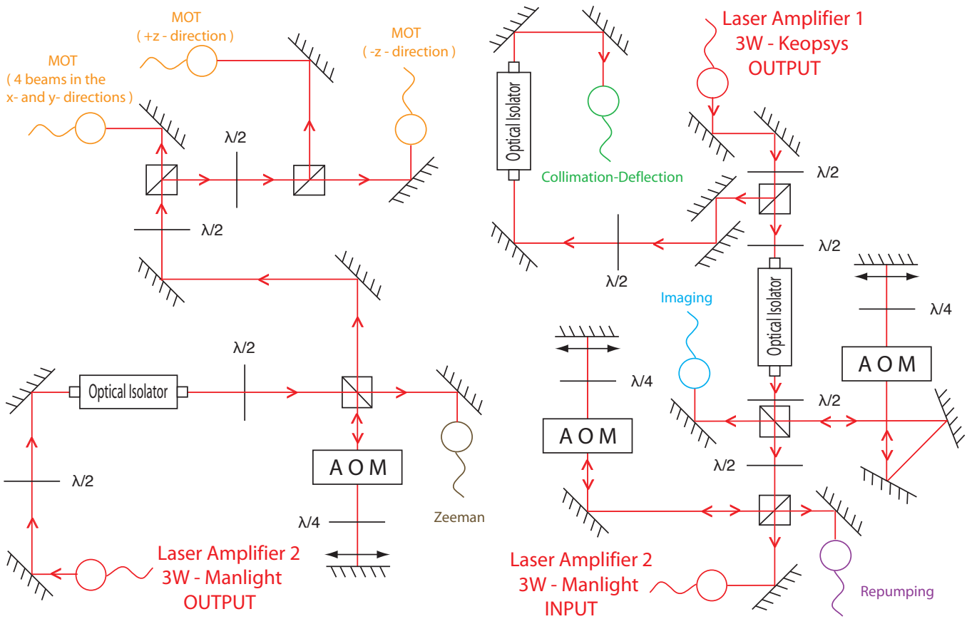
Figure 6.4: Main optical setup used to create all required optical beams. The output of amplifier 1 provides 3 W of light which is used for collimation, deflection, imaging as well as for injecting a second laser amplifier (amplifier 2 input). This second amplifier provides enough power for both the Zeeman and MOT beams.
