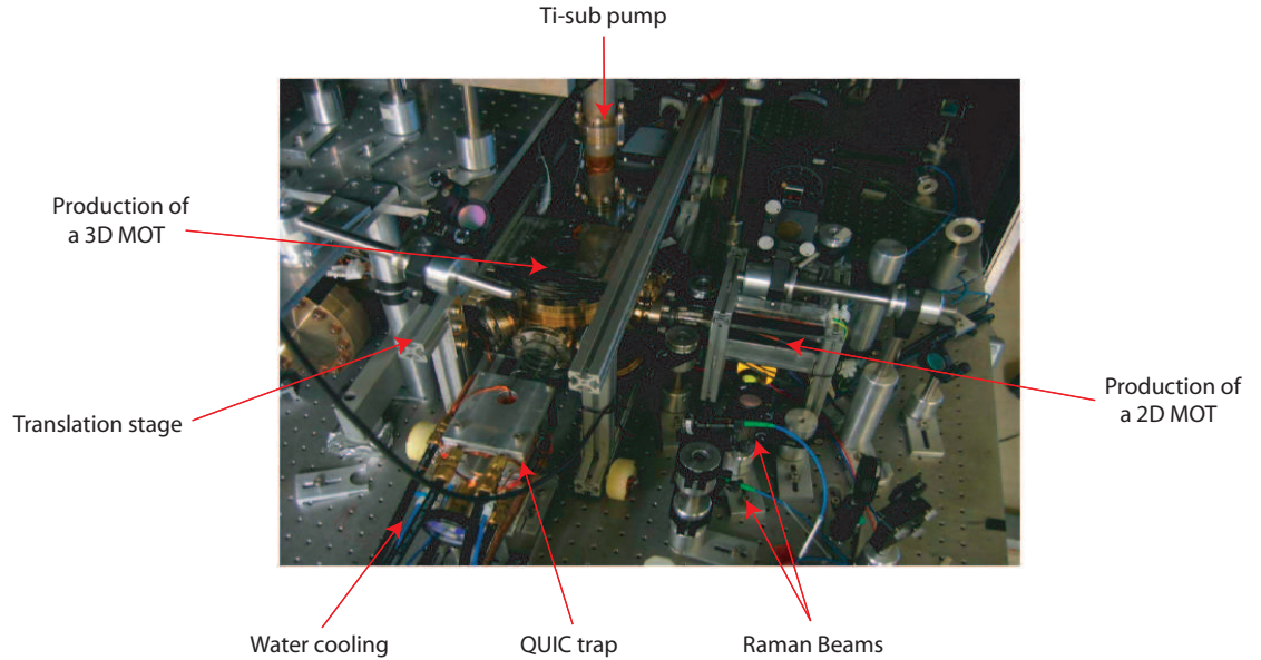
Figure 2.1: Picture of the BEC machine. One can see the location of the 2D and 3D MOT as well as the translation stage used to transport the atoms from the 3D MOT to the QUIC trap. The output of the optical fibers used for the Raman beams can also be seen.
