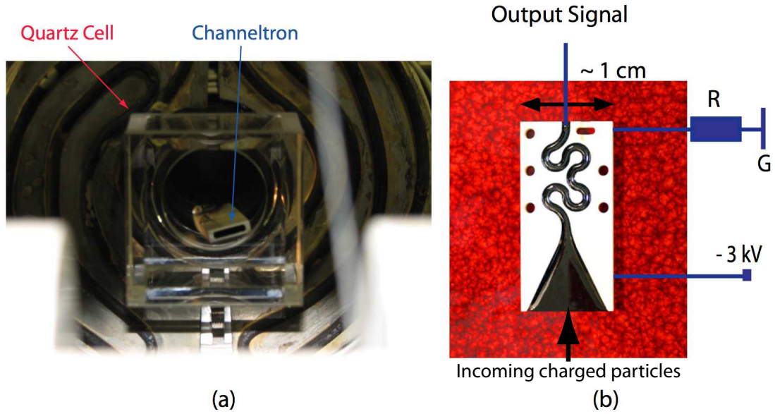
Figure 6.9: a) Picture of the channeltron, located just before the quartz cell where the atoms are trapped. b) Cut view of the channeltron, showing the external ceramic structure and the lead glass channel where the electron avalanche occurs.
