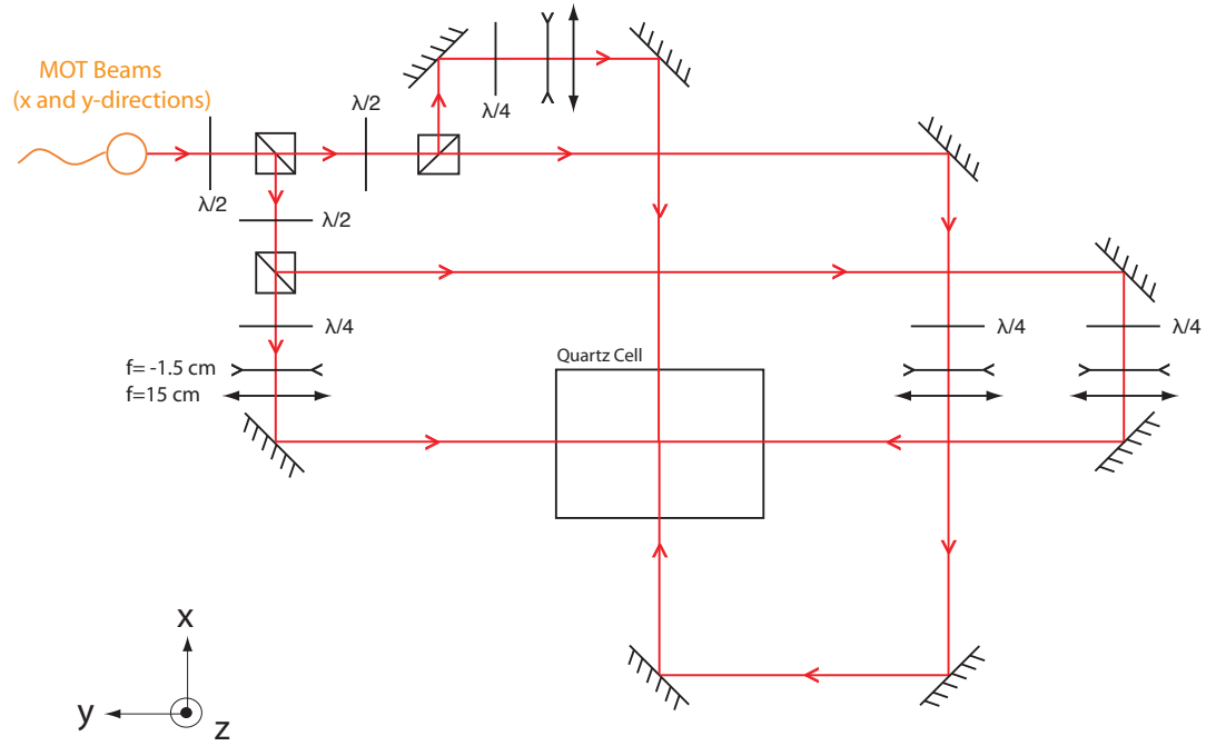
Figure 6.12: Schematic of the MOT beams in the vertical xy -plane. The third pair of beams along the z -direction is not represented. The power balance can be adjusted using half wave-plates and polarizing beam-splitters. Each MOT beam is expanded 10 times in a telescope.
