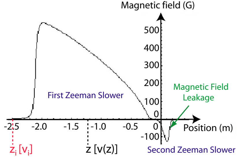
Figure 6.8: Magnetic field configuration in both Zeeman slowers, calculated from the Biot-Savart law [130].
