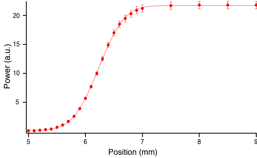
Figure 7.7: Measured laser power (dots) as a function of the position of the razor blade. 10% error bars are considered to account for experimental uncertainties. The solid line is a fit to an Error function. A beam waist of w = 0.72 \pm 0.02 mm is determined from the fit.
