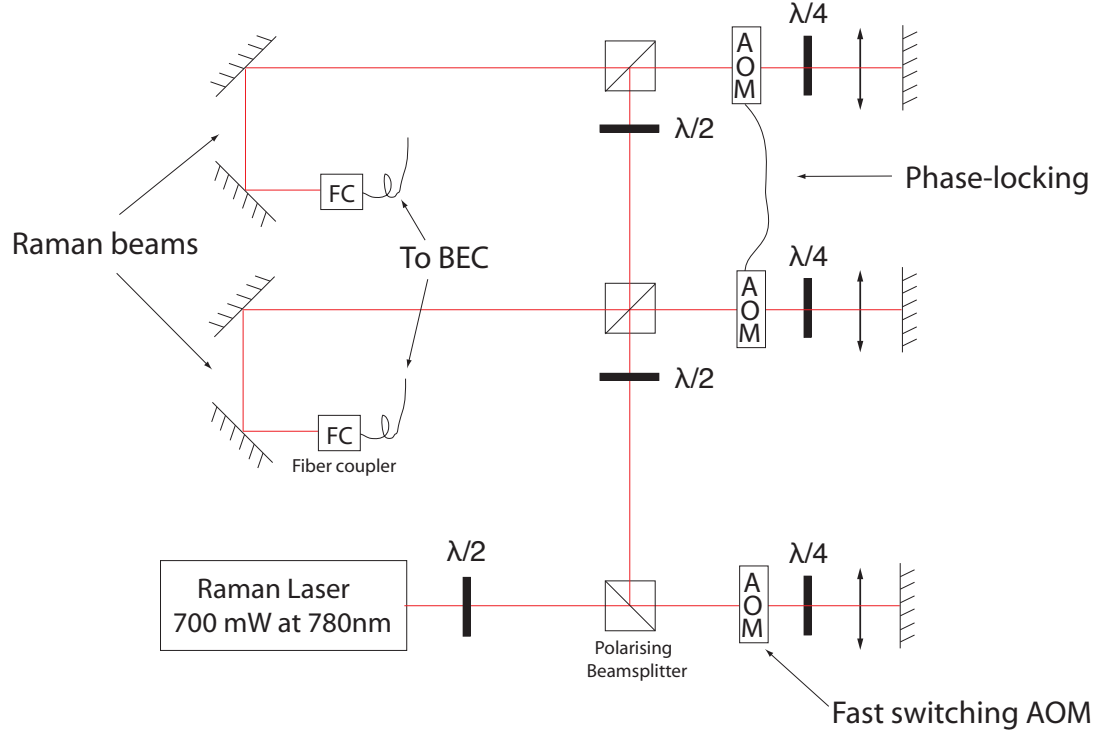
Figure 2.10: Optical setup used to prepare the laser beams for Raman outcoupling. A fast AOM can switch the Raman beams in less than 200 ns with an extinction ratio greater than 60 db. The frequency difference between the two Raman beams is tuned using two distinct AOMs. The light is fiber-coupled and sent to the BEC machine where the polarization of each beam is adjusted (figure 2.11).
