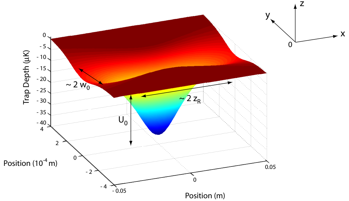
Figure 7.2: Dipolar potential experienced by the atoms in the case of a single dipole trap. The trap depth is characterized by U_0 whereas characteristic lengths are given by w_0 and z_R along the transverse y -direction and the x -direction of propagation respectively.
