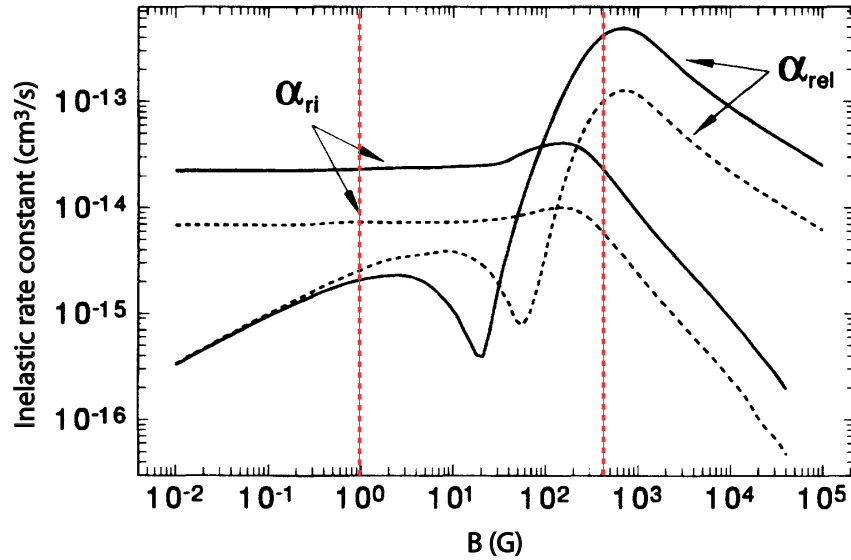
Figure 7.11: Theoretical results obtained in [128]. The rate constants at T = 0 K for spin relaxation ( \alpha^{rel} ) and relaxation-induced Penning ionization ( \alpha^{ri} ) are given as a function of the external magnetic field. Solid curves correspond to the final potential U_2(R) calculated in [156] and dashed curves to the same potential multiplied by 1.01. The vertical dashed lines represent the range of magnetic field values which we plan to sweep experimentally.
