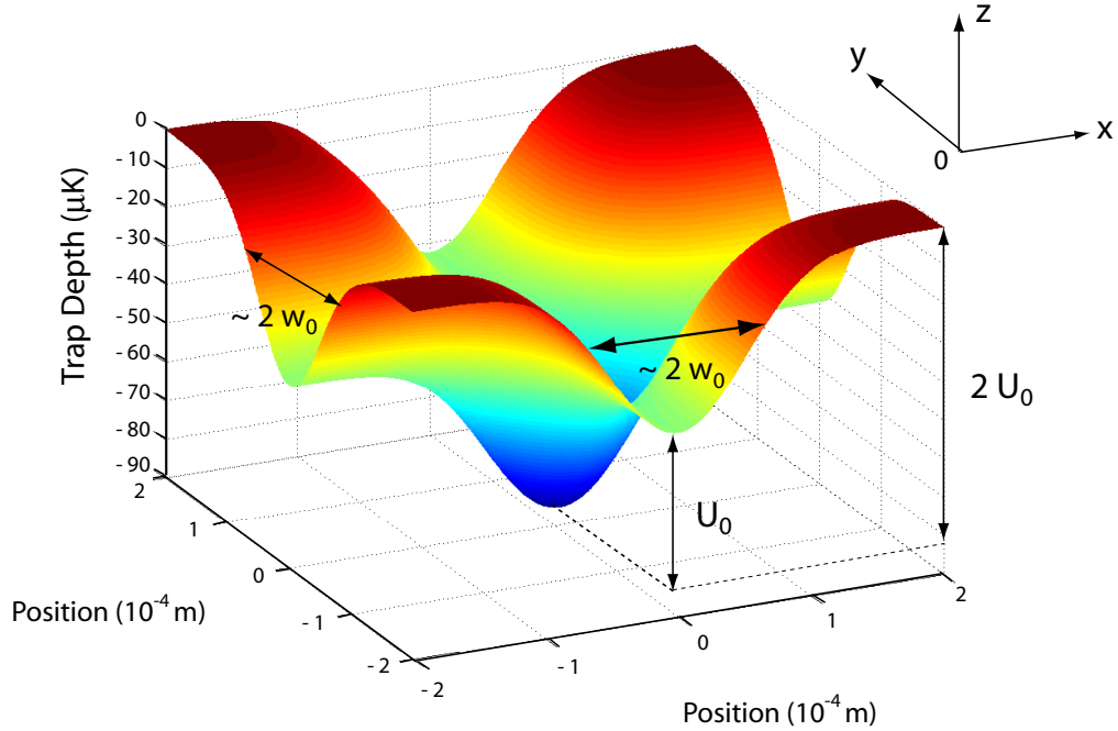
Figure 7.4: Quasi-isotropic dipolar potential experienced by the atoms in a crossed-beam configuration. The effective trap depth is only U_0 because atoms with a higher energy can leave the trapping region along one of the arms (x- or y-directions) of the laser beams.
