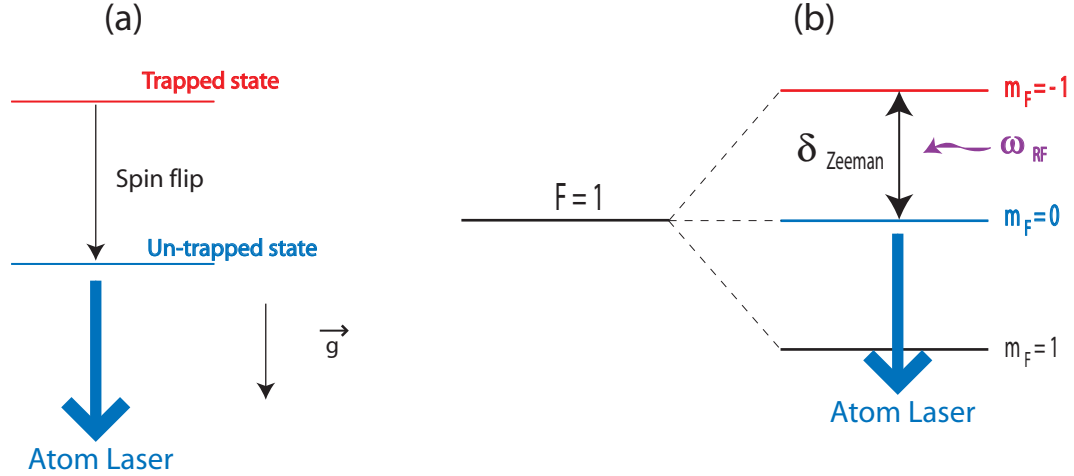
Figure 1.5: The scheme (a) shows the basic principle of RF out-coupling which is applied to the case of the F=1 manifold (b) in our experiment.
