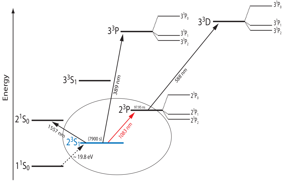
Figure 6.1: Energy levels of ^4\text{He} . In our experiment, we prepare the atoms in the 2^3S_1 metastable state which is considered as an effective ground state due to its very long lifetime. We use the 2^3S_1 \rightarrow 2^3P_2 optical transition at 1083 nm to manipulate and cool the atoms.
