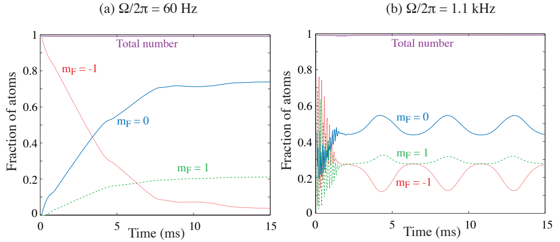
Figure 5.6: Comparison of the population dynamics in the three-state system for (a) weak and (b) strong coupling. Parameters are N = 5 \times 10^4 atoms, \omega_z = 2\pi \times \frac{260}{\sqrt{2}} \text{ Hz} , U = 6.6 \times 10^{-4} , G = 9.24 , and \Delta = 43 .
