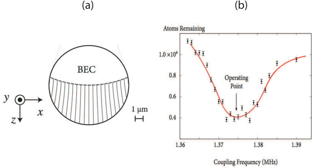
Figure 3.1: (a) Represents a cross-section of the condensate along the two directions of strong confinement. The long axis is along the y direction and the BEC has a cigar shape with an aspect ratio of about 10. The dashed line is the out-coupling cut at the center of the condensate. (b) Shows a typical RF output coupling spectroscopy of the BEC from which the operating point at the center of the condensate (designated by the arrow) is determined. The solid line is only to guide the eye. Error bars are based upon typical standard deviation.
