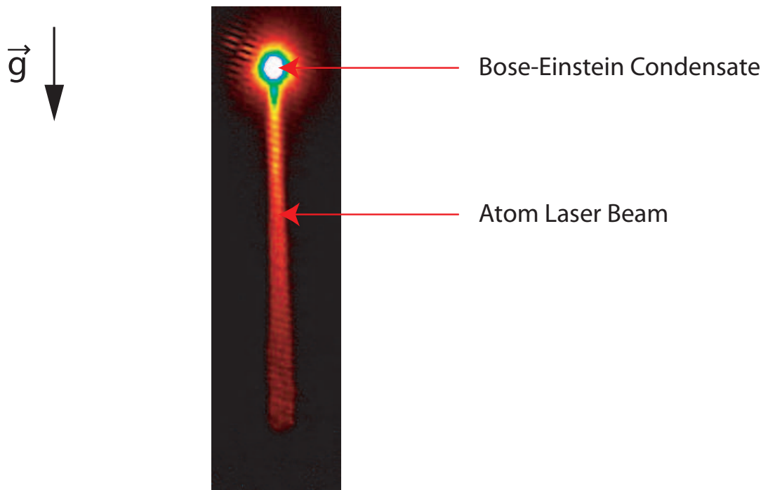
Figure 1.2: Atom laser produced in our lab after a long (10 ms) pulse of out-coupling. The atoms have fallen under gravity creating an atom laser beam 0.5 mm long. At the top of the figure is the BEC. The time of flight for imaging the system was on the order of 3 ms.
