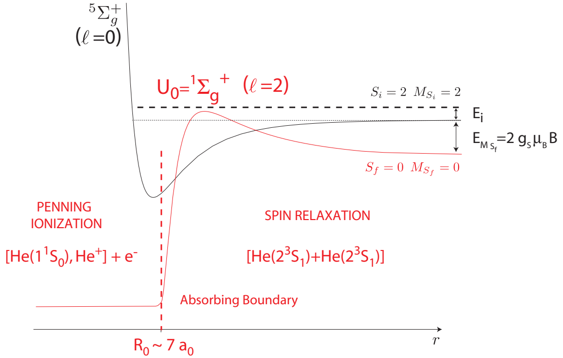
Figure 7.10: Interaction potentials of the initial |S_i = 2, M_{S_i} = 2\rangle state (black curve) and a final |S_f = 0, M_{S_f} = 0\rangle state (red curve). The two triplet and singlet potentials are coupled by the spin-dipole hamiltonian and separated by the Zeeman energy E_{M_{S_f}} = 2g_s\mu_B B . E_i is the initial energy of two colliding spin-polarized metastable helium atoms and the distance R_0 is the approximate position of the absorbing boundary at which Penning ionization occurs with a probability close to unity.
