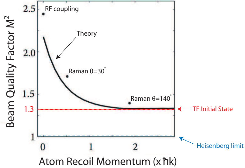
Figure 3.4: Calculated and measured quality factor M^2 of an atom laser. The solid line is the theoretical prediction whereas the three dots are the experimental measurements obtained after RF or Raman out-coupling at 2 different angles. The discrepancy between theory and experiment seems to be due to systematic errors which we attribute to the second order Zeeman effect, ignored in the model. The theoretical line does not converge towards M^2 = 1 but rather M^2 = 1.3 due to the Thomas-Fermi initial state of the condensate.
