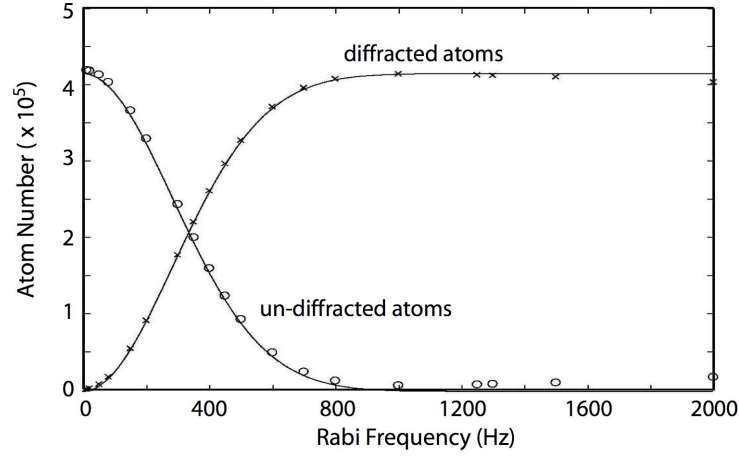
Figure 4.6: Theoretical predictions of the efficiency of the Bragg diffraction process showing the number of diffracted and un-diffracted atoms as a function of the two-photon Rabi frequency. Solid lines are the predicted Landau-Zener transition probabilities whereas the symbols are the results from a Gross-Pitaevskii simulation. The angle between the laser beam and the horizontal is \theta/2 = 15^\circ .
