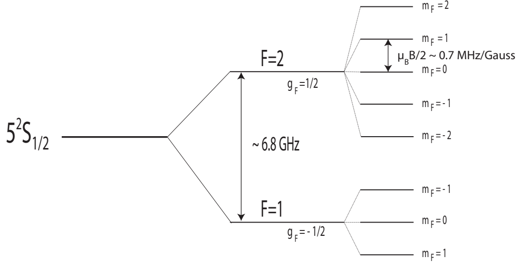
Figure 1.4: Atomic spectroscopy of the ground state of ^{87}\text{Rb} in a small bias field.
