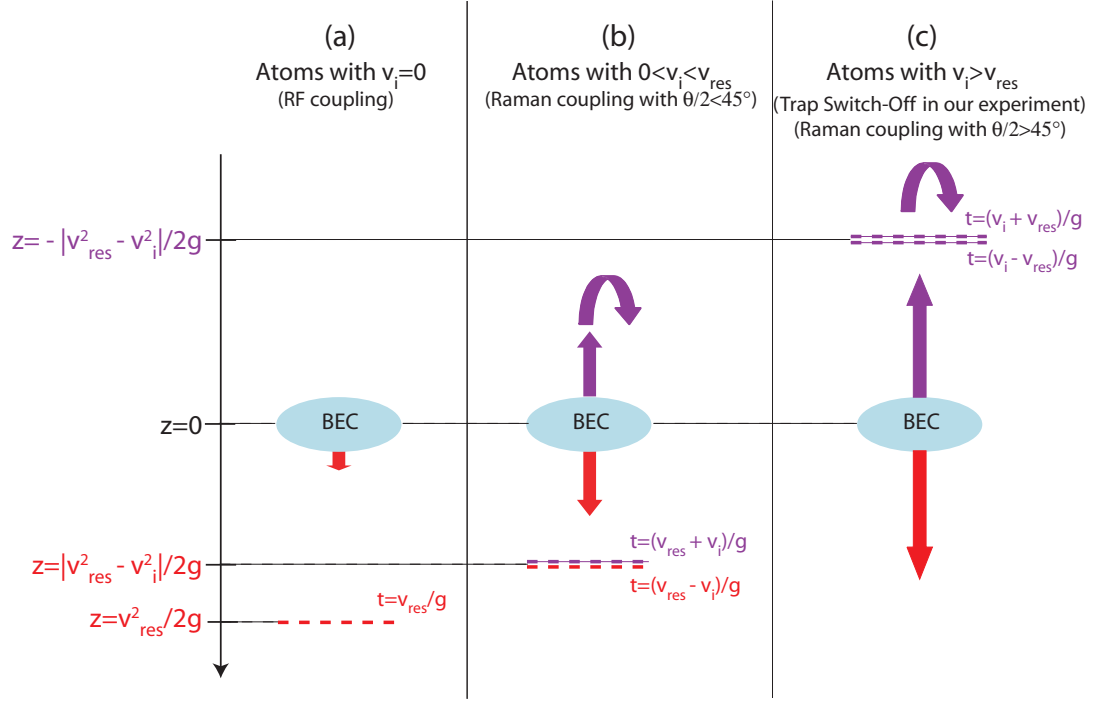
Figure 4.3: Position of the velocity resonance for Bragg diffraction after (a) RF and (b) Raman out-coupling. (c) Illustrates the case of our experimental trap switch-off (see section 4.3.2) where the atoms are initially launched upwards. Note that there are 2 velocity resonances in the latter case, first when the atoms propagate upwards, and then after they have turned back and propagate downwards.
