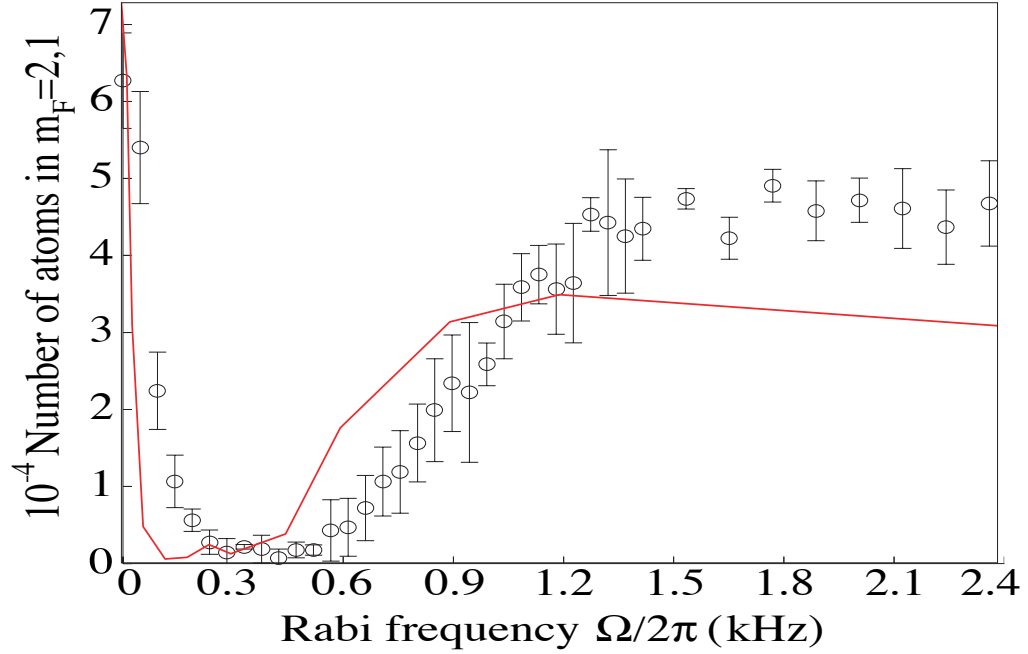
Figure 5.2: Total atomic population remaining in the magnetic trap after 100 ms of output coupling as a function of Rabi frequency for both our numerical model (solid line) and previous experimental measurements performed by our group [29] (open circles).
