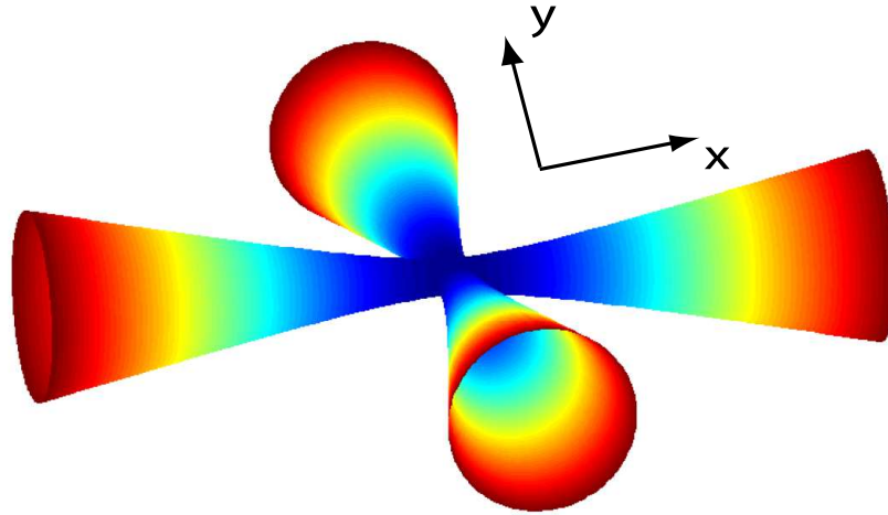
Figure 7.3: Laser beam profile of two crossed Gaussian beams intersecting at their foci.
