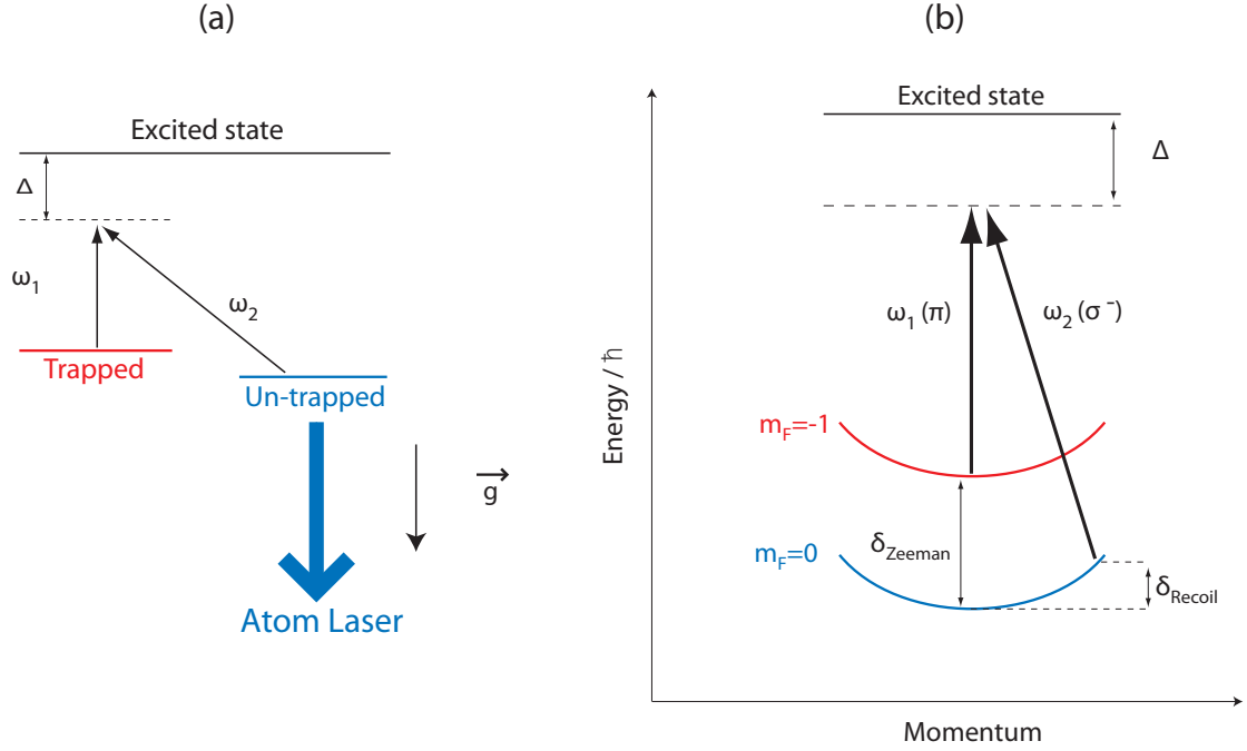
Figure 1.6: Schematic showing the basic principle of Raman out-coupling (a) as well as the restrictions of energy and momentum conservation on a two photon Raman transition in the F=1 manifold of our experiment (b). The parabolas correspond to the kinetic energy of the atoms, equal to p^2/2m .
