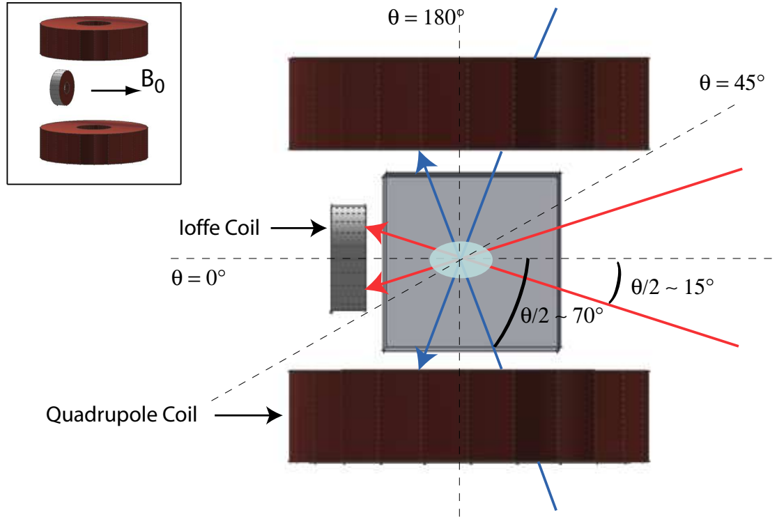
Figure 4.1: Experimental setup showing the position of the magnetic coils with respect to the glass cell. Two sets of optical Raman beams hitting the coils after they have passed through the BEC are also represented at small and larger incidence angles \theta/2 . Note that due to the magnetic field from the Ioffe coil the condensate does not sit at the center of the glass cell but is displaced towards the Ioffe coil.
