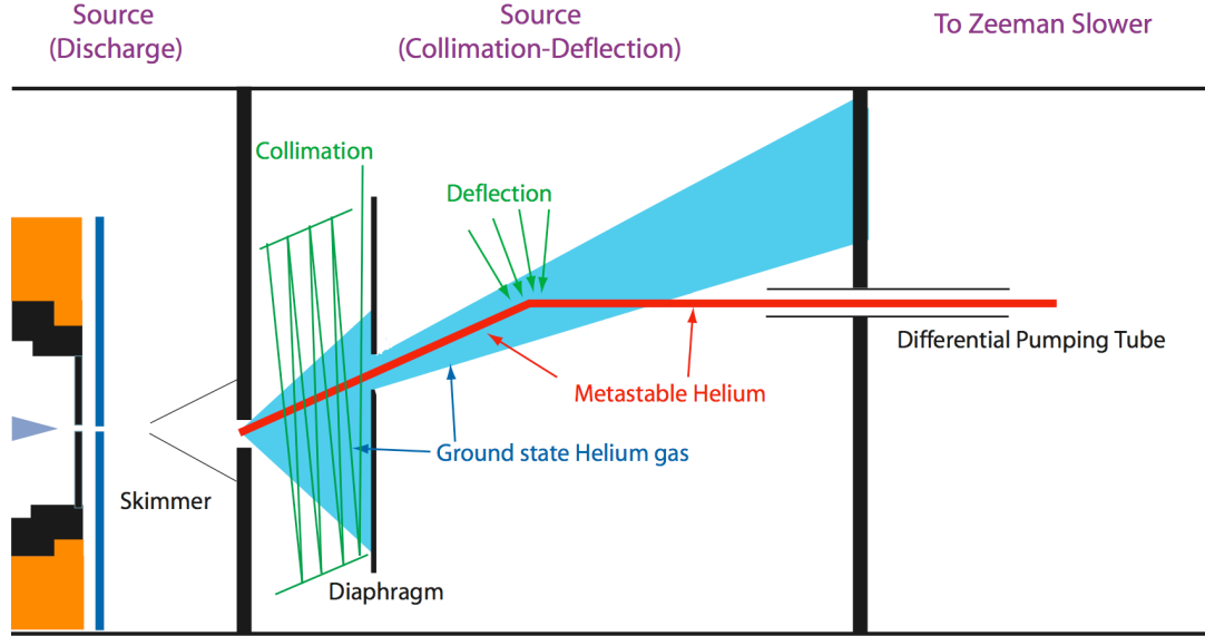
Figure 6.6: Scheme used for separating the beam of metastable atoms from atoms in the He ground-state. First, the metastable atoms are collimated to reduce the initial divergence. Second, the beam of metastable atoms is deflected to enter the differential pumping tube of the Zeeman Slower whereas atoms in the ground-state are selectively blocked and pumped out of the vacuum system.
