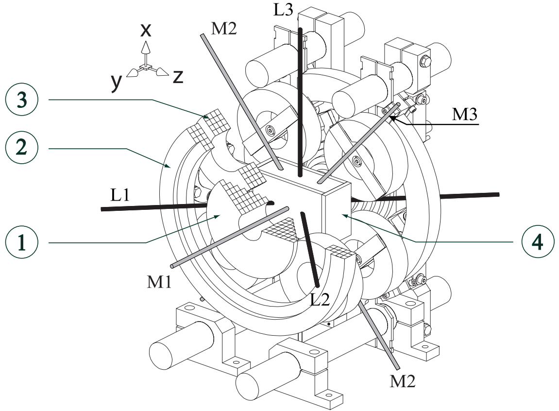
Figure 8.3: Three-dimensional view of the coil and beam geometry. Some mechanical components in the positive Y -direction are sliced open in order to expose the coil wiring. Coils no.1 are the ‘pinch coils’, coils no.2 are the ‘compensation coils’ and coils no.3 are the ‘cloverleaf coils’, spaced by 54 mm in the Y direction. Object no.4 is the 40 \times 40 \times 60 mm UHV-glass cell. M grey bars represent the MOT beams, L black bars represent the lattice beams.
