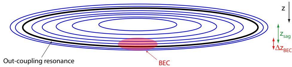
Figure 1.8: The sag of the condensate due to gravity, viewed orthogonal to the weak trapping axis. The red ellipse represents the condensate and the blue contour lines show the magnetic field magnitude, increasing away from the central minimum. An out-coupling frequency resonance is depicted by the thick, black line.
