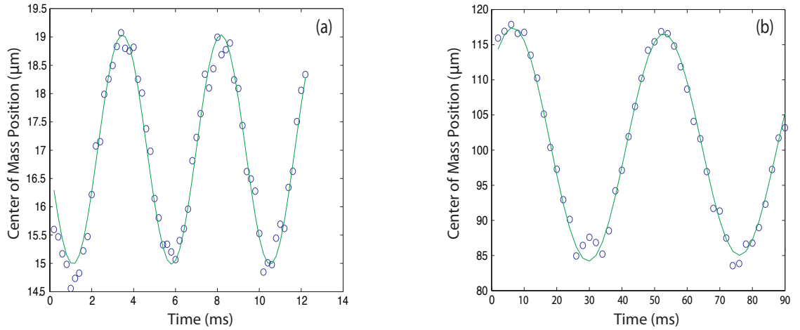
Figure 2.9: Trap oscillations of the cloud center-of-mass. The measurements (circles) are fitted to an exponentially damped sinusoidal function (solid lines). For atoms in the F = 2, m_F = 2 state, a radial frequency of \omega_p = 2\pi \times 204.6 Hz (a) and an axial frequency of \omega_y = 2\pi \times 20.4 Hz (b) are measured.
