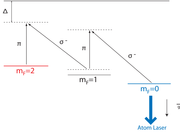
Figure 1.7: The four photon Raman outcoupling scheme in the F = 2 manifold
