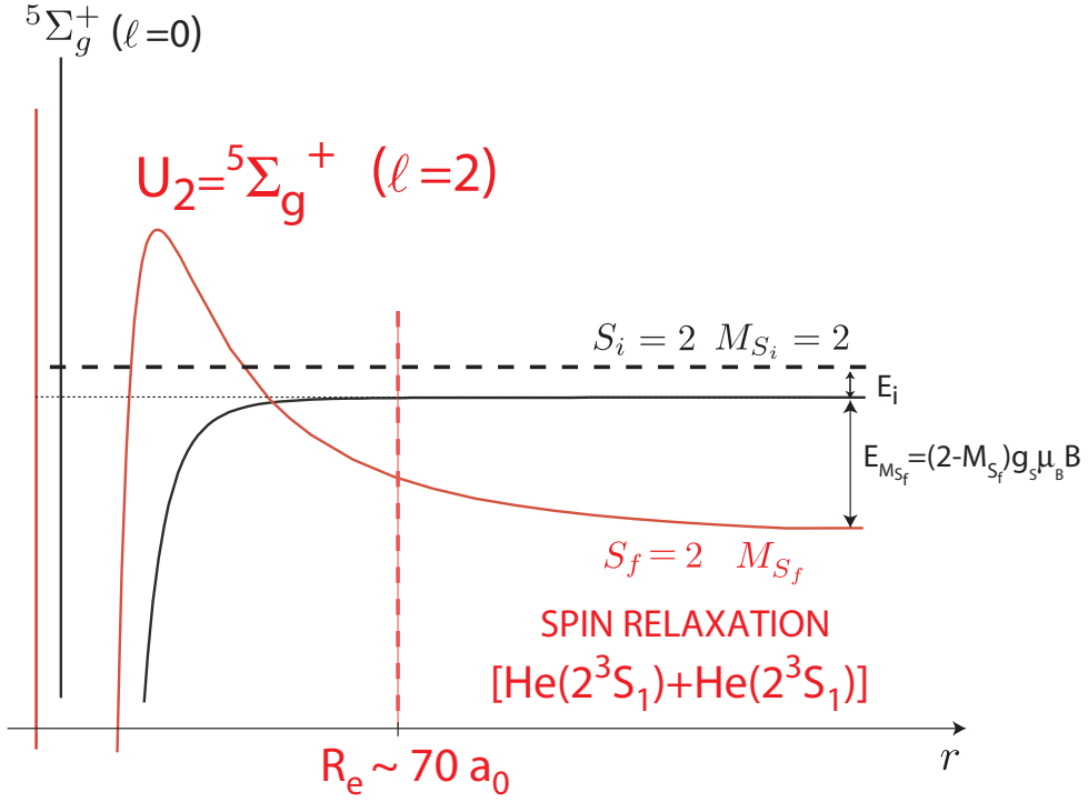
Figure 7.9: Interaction potentials of the initial |S_i = 2, M_{S_i} = 2\rangle state (black curve) and a final |S_f = 2, M_{S_f} = 0, 1\rangle state (red curve). The two triplet potentials are coupled by the spin-dipole hamiltonian and separated by the Zeeman energy E_{M_{S_f}} = g_s \mu_B B (2 - M_{S_f}) . E_i is the initial energy of two colliding spin-polarized metastable helium atoms and the distance R_e is the characteristic radius of interaction.
