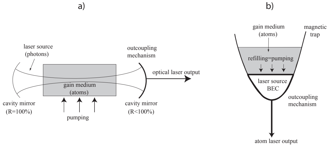
Figure 1.3: Physical elements constituting an optical laser (a) and an atom laser (b). In both cases, the lasing mode has a macroscopic population of bosons. In an optical laser, the lasing mode is multiple wavelengths long. In an atom laser, the lasing mode is the ground state of the trap. Both lasers rely on an irreversible stimulated process to populate the lasing mode.
