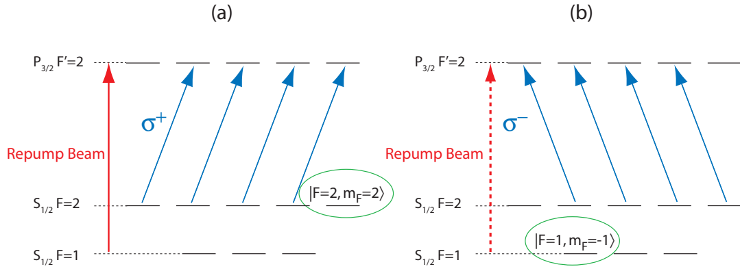
Figure 2.7: Schematics of optical pumping cycles to polarize the atoms in a) the |F = 2, m_F = 2\rangle state or b) the |F = 1, m_F = -1\rangle state using \sigma^+ or \sigma^- light respectively. In (b), the dashed line for the repump illustrates that it is a short pulse which is switched off before the end of the optical pumping sequence.
