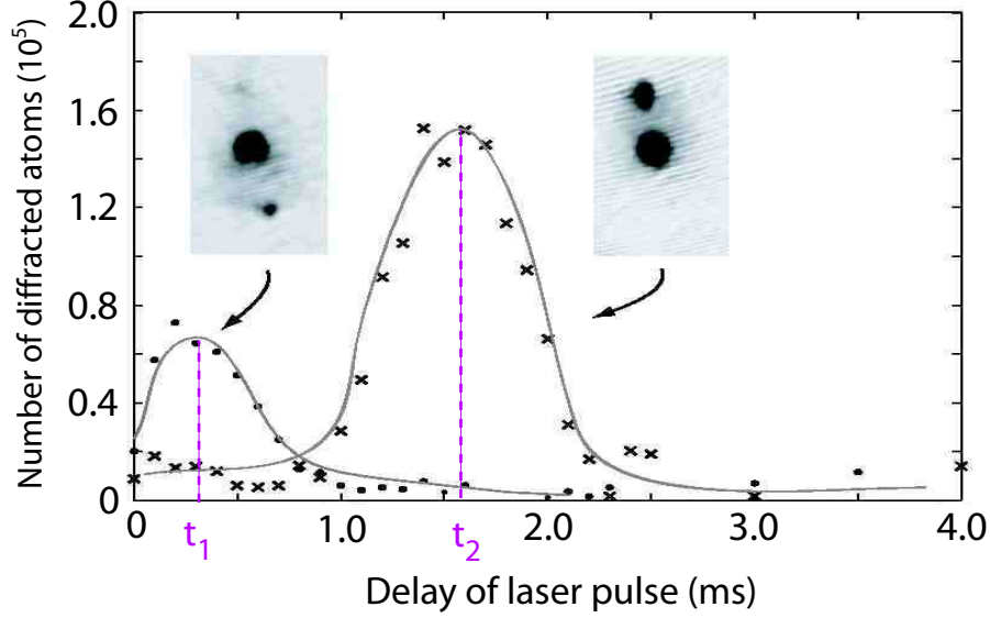
Figure 4.4: Number of diffracted atoms as a function of pulse delay relative to trap switch-off. Upon trap switch-off, the entire BEC was released with an initial velocity in the upward direction due to remnant magnetic fields (see figure 4.3c)). Shown are the two possible velocity resonances for the atoms traveling upwards (circles) and then traveling downwards (crosses). Pulse duration is 300 \mu\text{s} (the delay is given from the start of the pulse) and \theta/2 = 70^\circ . The insets show the corresponding images, each 480 \times 890 \mu\text{m}^2 . The lines are interpolations to guide the eye.
