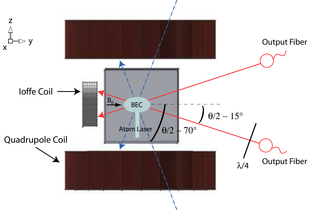
Figure 2.11: Optical layout used to illuminate the BEC with the two Raman beams of appropriate polarization. In our setup two configurations are used with the angle between the beams being set to 30^\circ or 140^\circ .
