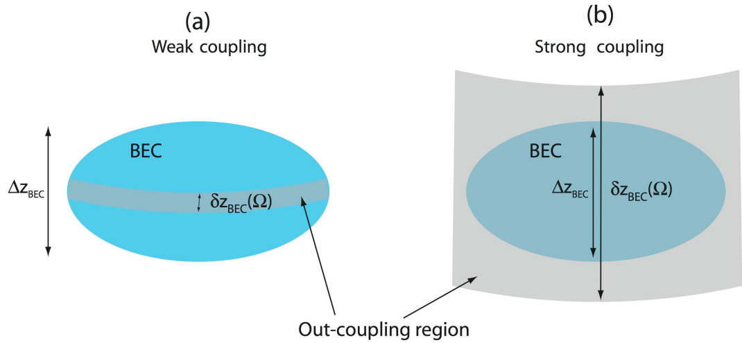
Figure 1.9: Schematics of the model for weak (a) and strong (b) out-coupling regimes.
