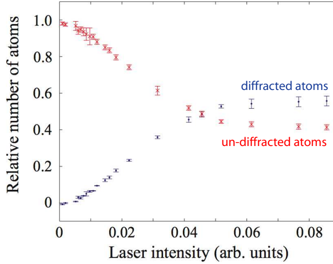
Figure 4.5: Diffraction efficiency as a function of laser intensity for a fixed pulsed duration of 2 ms. The laser beam is at an angle of \theta/2 = 15^\circ to the horizontal. The entire BEC is released after trap switch-off and the laser pulse is applied after 3.4 ms. The relative number of diffracted and un-diffracted atoms is measured after absorption imaging and is represented by the blue dots and red crosses respectively.
