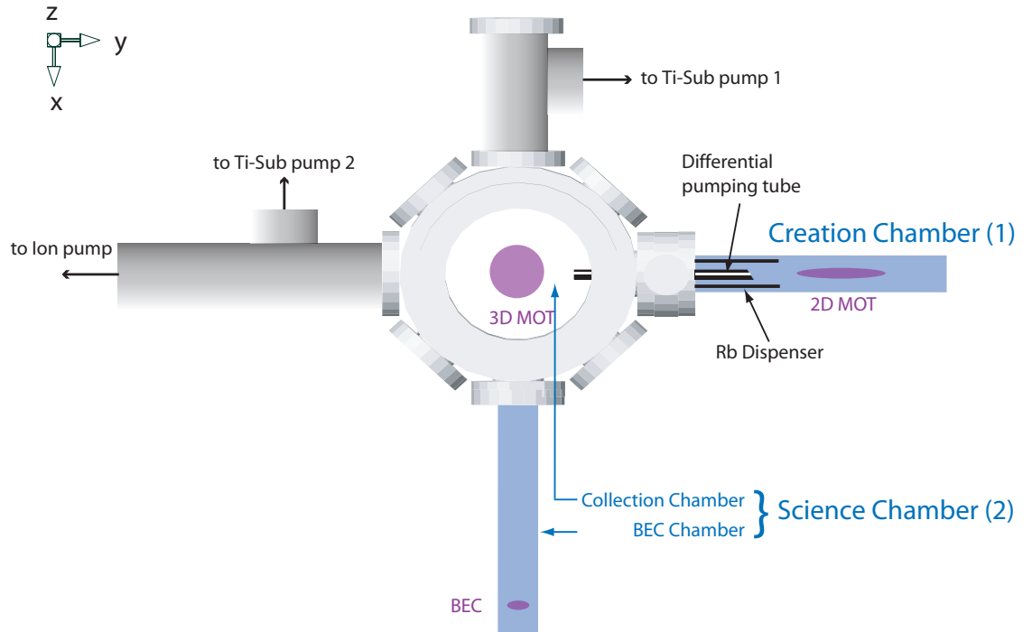
Figure 2.5: Schematic of the vacuum system. The Collection chamber is pumped by a 40 \text{ l.s}^{-1} ion pump running continuously. Two titanium-sublimation pumps were also used a few times in order to improve the ultra-high vacuum in the BEC Chamber. The Creation chamber is pumped through a differential pumping tube and holds a vapor pressure of Rb atoms which are produced by two dispensers.
