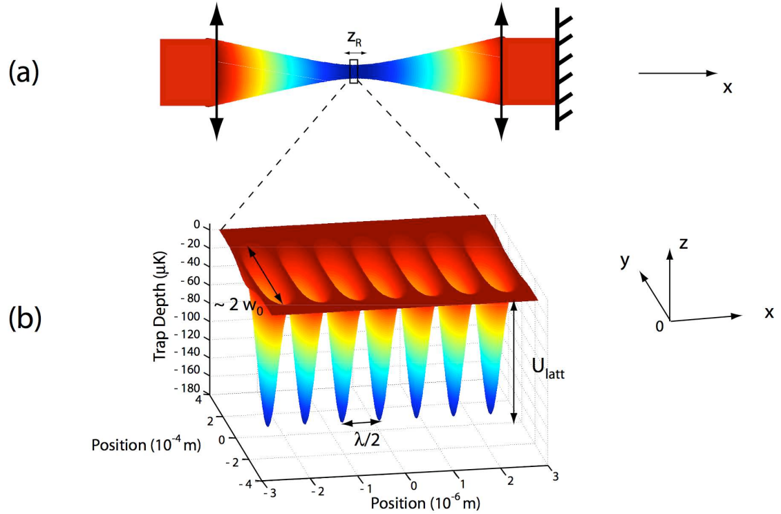
Figure 8.1: (a) Retro-reflected Gaussian laser beam propagating along the x -direction. (b) One-dimensional standing-wave laser field created in the Rayleigh range of the retro-reflected Gaussian laser beam of (a).
