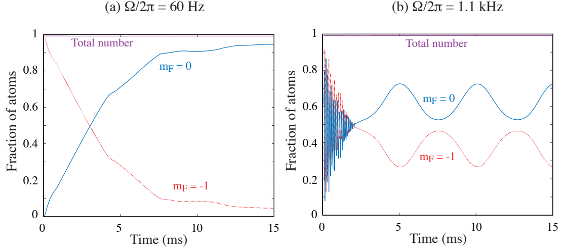
Figure 5.7: Comparison of the population dynamics in the two-state system for (a) weak and (b) strong coupling. Parameters are N = 5 \times 10^4 atoms, \omega_z = 2\pi \times \frac{260}{\sqrt{2}} \text{ Hz} , U = 6.6 \times 10^{-4} , G = 9.24 , and \Delta = 43 .
