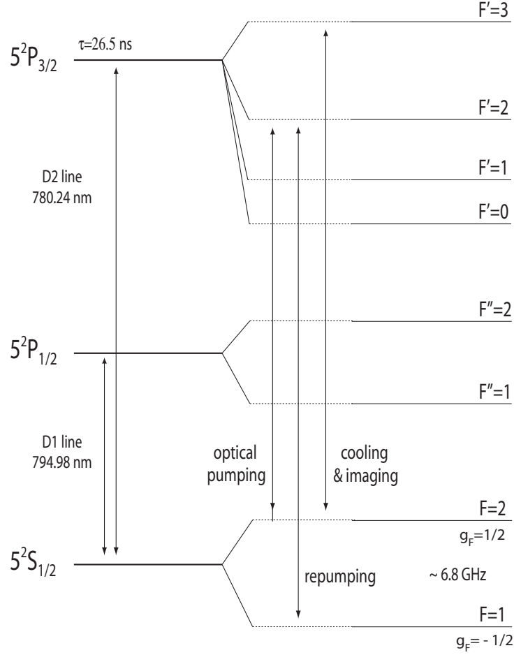
Figure 2.3: Atomic structure of ^{87}\text{Rb} . Several hyperfine levels of the D2 optical transition are used to cool and image the atoms.
