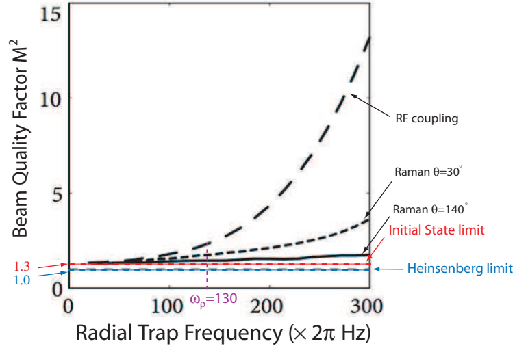
Figure 3.5: Comparison of the calculated beam quality factor M^2 as a function of the trapping frequency for RF and Raman out-coupling. The simulation always assumes out-coupling from the centre of the condensate. Whereas both techniques are comparable for small trapping frequencies, one can see the large improvement of using Raman out-coupling over RF in the case of large trapping frequencies.
