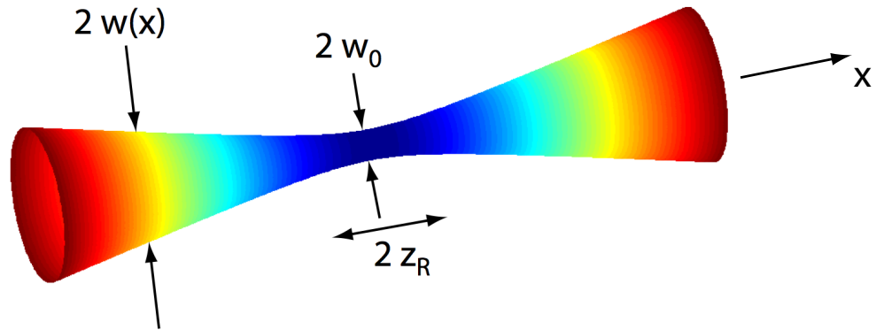
Figure 7.1: Laser beam profile of a single Gaussian beam of waist w_0 and Rayleigh length z_R .
