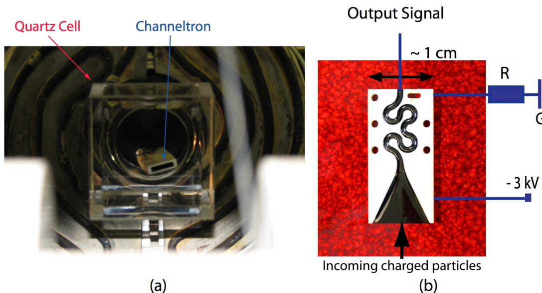
Figure 6.9: a) Picture of the channeltron, located just before the quartz cell where the atoms are trapped. b) Cut view of the channeltron, showing the external ceramic structure and the lead glass channel where the electron avalanche occurs.
