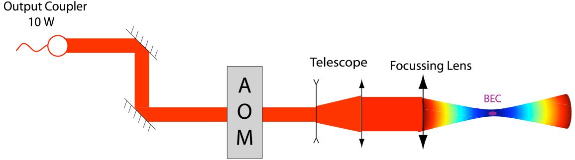
Figure 7.6: Creation of a focussed Gaussian beam. The output beam of the laser amplifier passes through an AOM which can switch the light on and off and change its central frequency. Finally, the beam is expanded before being focussed onto the BEC down to a waist of \sim 100 \mu\text{m} .
