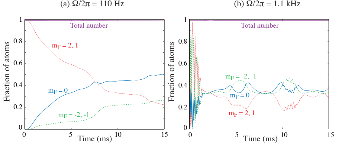
Figure 5.5: Comparison of the population dynamics in the five-state system for (a) weak and (b) strong coupling. Parameters are N = 5 \times 10^4 atoms, \omega_z = 2\pi \times \frac{260}{\sqrt{2}} Hz, U = 6.6 \times 10^{-4} , G = 9.24 , and \Delta = 10.7 .
