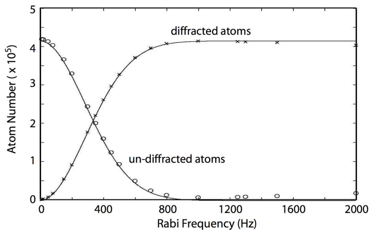
Figure 4.6: Theoretical predictions of the efficiency of the Bragg diffraction process showing the number of diffracted and un-diffracted atoms as a function of the two-photon Rabi frequency. Solid lines are the predicted Landau-Zener transition probabilities whereas the symbols are the results from a Gross-Pitaevskii simulation. The angle between the laser beam and the horizontal is \theta/2 = 15^\circ .
