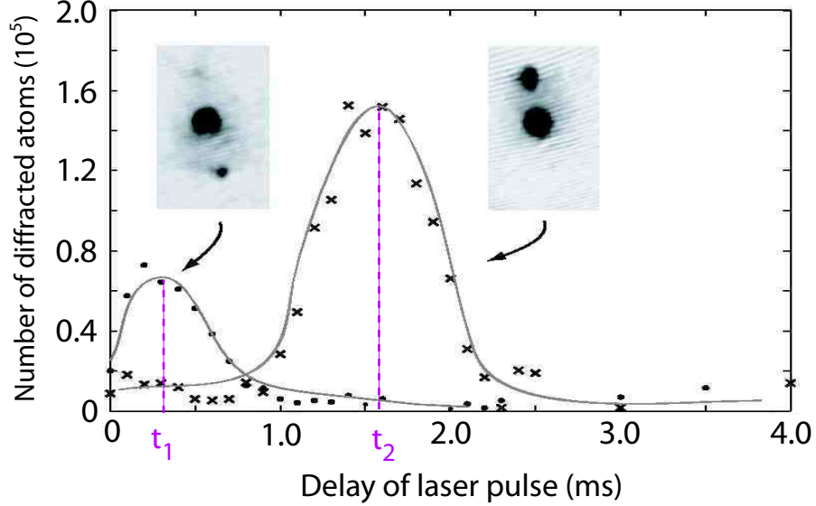
Figure 4.4: Number of diffracted atoms as a function of pulse delay relative to trap switch-off. Upon trap switch-off, the entire BEC was released with an initial velocity in the upward direction due to remnant magnetic fields (see figure 4.3c)). Shown are the two possible velocity resonances for the atoms traveling upwards (circles) and then traveling downwards (crosses). Pulse duration is 300 \mu\text{s} (the delay is given from the start of the pulse) and \theta/2 = 70^\circ . The insets show the corresponding images, each 480 \times 890 \mu\text{m}^2 . The lines are interpolations to guide the eye.
