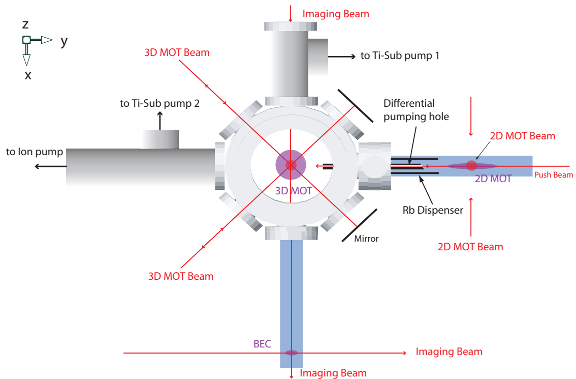
Figure 2.6: Arrangement of the optical beams onto the atoms. The imaging beam, the push beam, two pairs of 3D MOT beams as well as a pair of 2D MOT beams are represented by the red lines in the xy -plane. The red dots on the 2D and 3D MOT clouds represent the additional pair of 2D and 3D MOT beams respectively, along the vertical z -direction.
