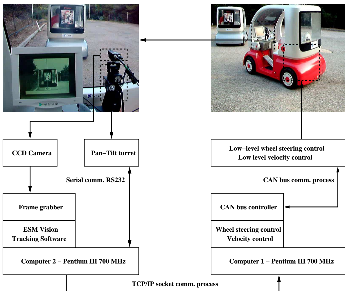
FIG. 4.3 – Overview of the complete system.
