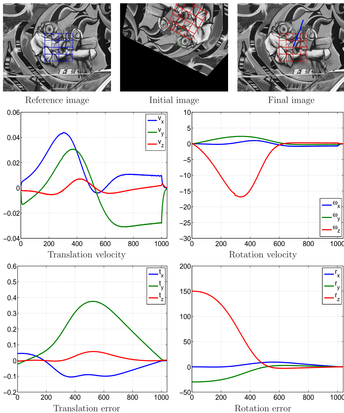
FIG. 4.7 – Direct visual servoing with respect to a planar target using the generic control law.
