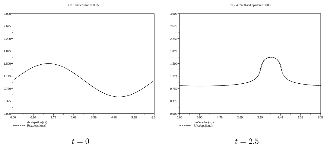
FIGURE 2.4 – Comparaison de \rho_h^\epsilon(\cdot, t) et R_h(\cdot, \frac{t}{\epsilon}, t) .
