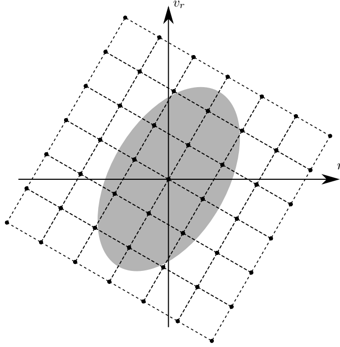
FIGURE 3.4 – Maillage M(\Omega(\frac{\pi}{3})) et support de (r, v_r) \mapsto f_0 \circ \gamma(r, v_r, \frac{\pi}{3}) .
