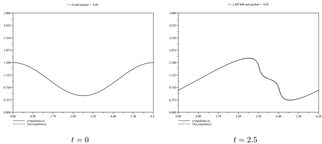
FIGURE 2.3 – Comparaison de u_h^\epsilon(\cdot, t) et U_h(\cdot, \frac{t}{\epsilon}, t) .
