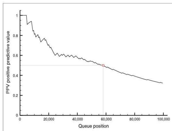
Figure 2 PPV calculated for each threshold in the top 100k of the final relevancy ranking, using the pseudo-curation results of 200 evenly distributed samples. The length of the final 'text-mining entry' component of the ORegAnno Publication Queue was chosen at 58,000, which yields a PPV of 50%.
