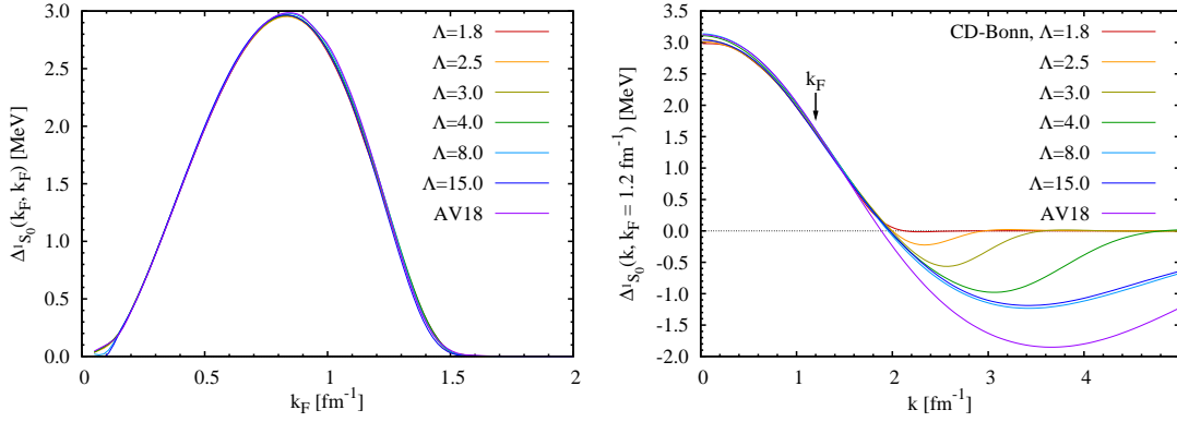
Figure 5.3: BCS infinite-matter pairing gaps calculated with a kinetic spectrum from our separable representations of V_{\text{low } k} /CD-Bonn potentials and bare Argonne v_{18} . Left panel: Fermi level gaps. Right panel: momentum-dependent gaps at k_F = 1.2 \text{ fm}^{-1} .
