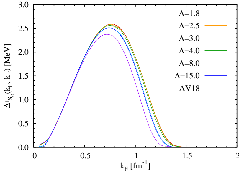
Figure 6.5: Neutron-neutron pairing gaps obtained at the Fermi level with the separable V_{low k} /CD-Bonn interactions at indicated RG cutoffs, as well as the Argonne V18 potential, and a s.p. spectrum produced by the SLy4 Skyrme EDF in SNM.
