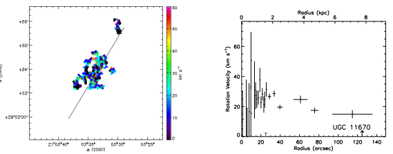
(184) UGC 11670
