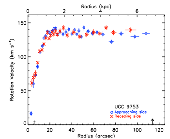
(126) UGC 09753
