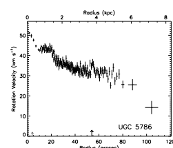
(90) UGC 05786
