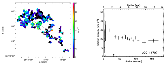
(185) UGC 11707
