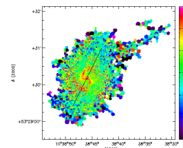
(90) UGC 05786
