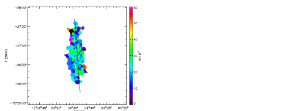
(163) UGC 10713
