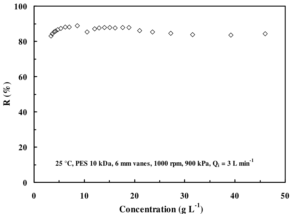
Figure 4.31 Variation of the membrane retention in the concentration tests of SDS solution till 46 g L -1 .
