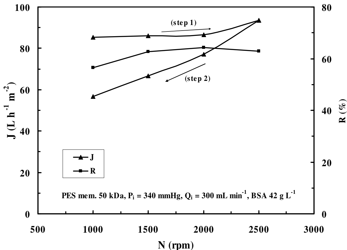
Figure 5.2 Permeate flux and BSA rejection of 50 kDa PES membrane as a function of rotation speed of inner cylinder.
