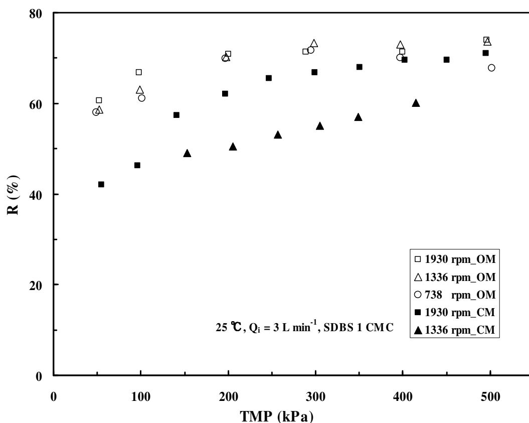
Figure 4.2 Effect of TMP on retention at different membrane rotating speeds for both PES and ceramic membranes.
