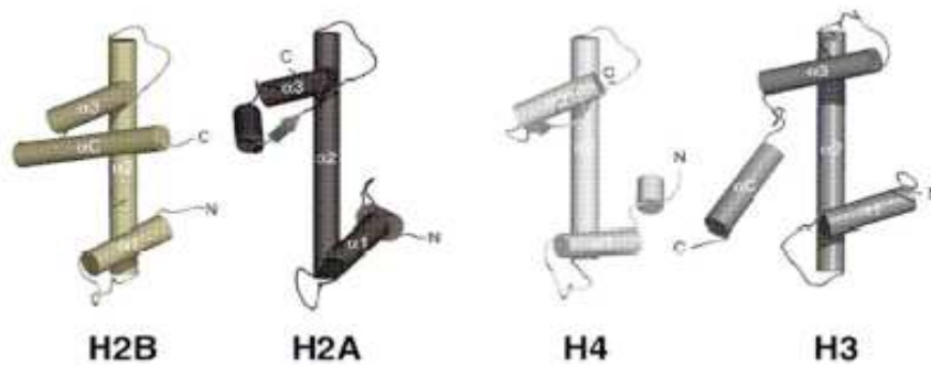
Figure I.2 Histone fold of the core histones (H2A, H2B, H3 and H4). All adopt the same secondary structure called as "histone fold", which consists of a sequence of three propellers \alpha represented by the cylinders. The histone fold is present at the base of histone dimerisation (H2A-H2B) and (H3-H4). Adapted from Sondermann et al., 2003
