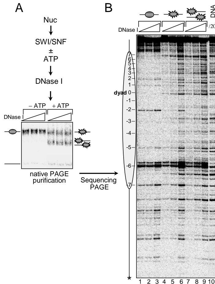
Figure III.2. DNase I footprinting analysis shows that nucleosome treatment with SWI/SNF resulted in perturbation of the histone-DNA interactions prior to nucleosome mobilization. Centrally positioned nucleosomes were reconstituted on 255 bp 601.2 DNA sequence and incubated with SWI/SNF at 29°C in the presence of ATP. Then the reaction was arrested with apyrase and aliquots were incubated with increasing amounts of DNase I for 2.5 minutes at room temperature. After arresting the DNase I digestion reaction, the samples were separated on a 5% PAGE under native conditions. The bands corresponding to either the non-slided particles (upper band) or slided particles (lower band) were excised from the gel, the DNase I digested DNA was eluted from the gel slices and run on a 8% sequencing gel. (A) Schematics of the experiment and 5% native PAGE fractionation of SWI/SNF treated and DNase I digested nucleosomes. (B) DNase I digestion pattern of control nucleosomes (lanes 1-3) and SWI/SNF treated nucleosomes isolated from the upper band (non-slided particles, lanes 4-6) and the lower band (slided particles, lanes 7-9). On the left side both the position of the histone octamer relative to the ends of the 601 DNA sequence and the nucleosome dyad are indicated. Lane 10, DNase I digestion pattern of naked DNA.
