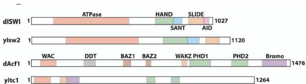
Figure I.18 Domain organization of ISWI subunits. Adapted from Gangaraju and Bartholomew, 2007.
