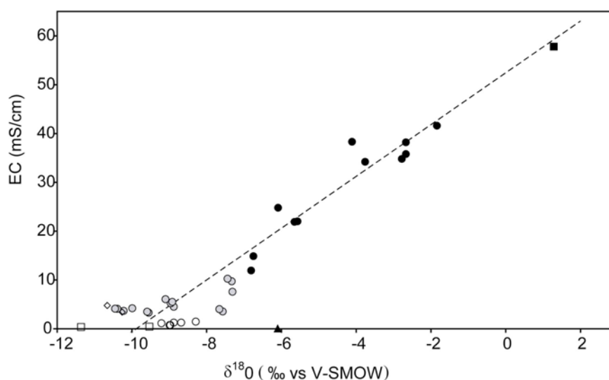
Fig. 4 \delta^{18}O vs EC (same symbols as in Fig. 3) for the water samples representation. The dotted black line stands for the linear trend between \delta^{18}O and EC for the saline groundwaters ( EC = 5.3041 \times \delta^{18}O + 52.43 ; r^2 = 0.88 ).
