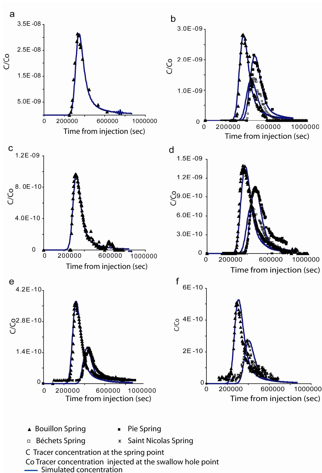
Fig 4.8 Comparison between simulated and measured BTCs for the tracer tests when conduit permeability =1.65 \times 10^{-5} m^2 between Jargeau and Bouillon Spring, and 5.5 \times 10^{-5} m^2 between Bouillon Spring and the confluence Loire - Loiret, hosted limestone permeability =5.7 \times 10^{-10} m^2 . a test 6/02/1973, b test 20/02/1998, c test 25/05/2001, d test 15/11/2001, e test 16/11/2006, f test 14/11/2007
