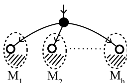
FIG. 6.6 – General form of the connected component containing \star of a map appearing in D_1(M) .
