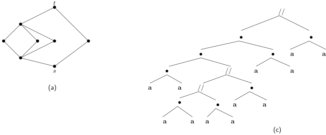
(a) (((a \bullet a) \bullet (((a \bullet a) // (a \bullet a)) // (a \bullet a))) \bullet (a \bullet a)) // (a \bullet a) (b)
