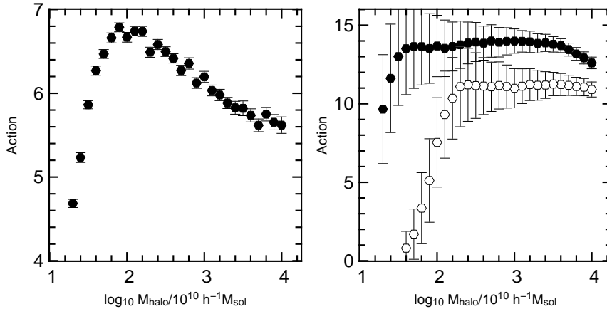
Figure 5. Left panel Normalized walk action S , Eq.(3), as a function of halo mass for merger trees extracted from the Millennium Run. We find again a transitional mass-scale around 1.0 \times 10^{12} h^{-1} M_{\odot} , which could be interpreted as the mean branch length reaching a maximum for that halo mass. Right panel The same as the left panel for merger trees constructed with the Markovian algorithm. Black symbols refer to the high resolution run, white symbols to the low resolution run. The transitional mass-scale is replaced by a plateau. Here the mass resolution plays an important role shaping the general trend for the action S . As in the length case, the dispersion in the measurements from Markovian trees is larger than the measurements coming from Millennium Run data.
