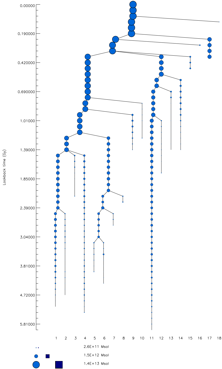
Fig. 2.2. Merger tree of a dark matter halo of mass \sim 10^{13}M_{\odot} constructed from a dark matter simulation. Each circle represents a dark matter halo with an area proportional to its mass. The horizontal levels mark each timestep in the simulation, and the lines between the circles show parenthood links. Time advances from the bottom to the top of the page. The mass of the smallest halos present in the tree is fixed by the resolution of the dark matter simulation. Figure kindly prepared by Dylan Tweed using data from the simulation presented in Figure 2.1.
