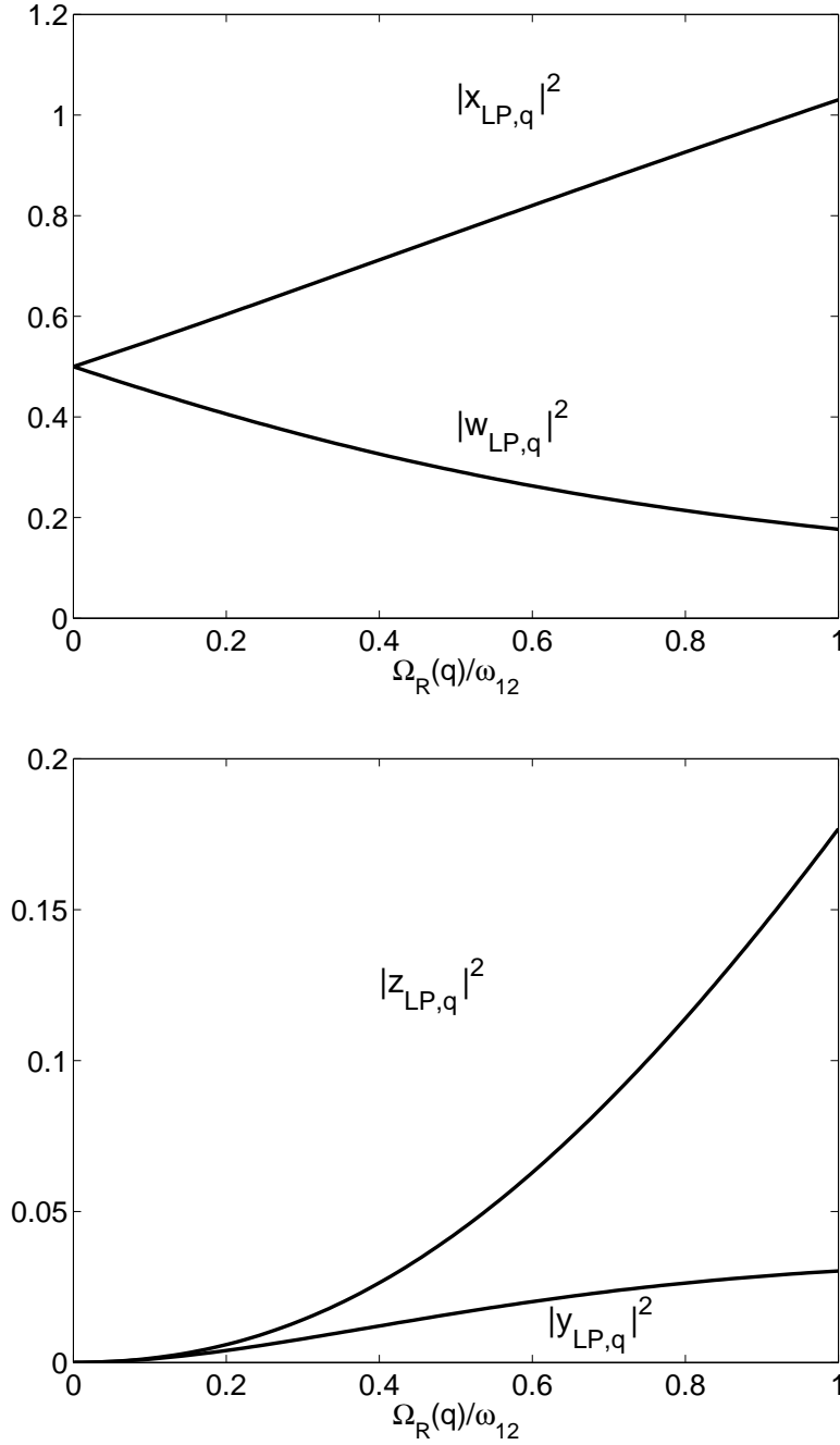
Figure 2.3: Mixing fractions for the Lower Polariton (LP) mode as a function of \Omega_R(q)/\omega_{12} . The calculation has been performed with \mathbf{q} such that \omega_{cav}(q) + 2D(q) = \omega_{12} . The Upper Polariton (UP) fractions (not shown) are simply |w_{UP,q}| = |x_{LP,q}| , |x_{UP,q}| = |w_{LP,q}| , |y_{UP,q}| = |z_{LP,q}| , |z_{UP,q}| = |y_{LP,q}| . See Ref. [25].
