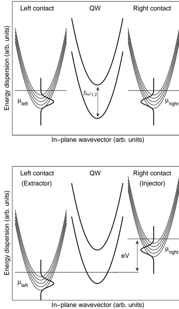
Figure 3.1: Top panel: sketch of the energy dispersion of the two quantum well subbands and of the minibands in the left and right contacts in the zero-bias case. Here the system is in thermal equilibrium and the Fermi level in the quantum well is the same as in the two contacts. The doping level in the contacts determines the equilibrium density in the quantum well. The subband and minibands have an energy dispersion versus the in-plane wavevector, which is a conserved quantity in the planar structure. This electronic structure is embedded in a planar microcavity, with a cavity photon mode quasi-resonant to the intersubband transition. Bottom panel: the same but with an applied voltage bias. Here, the left contact acts as an electronic extractor, while the right one is the injector. In the quantum well, non-equilibrium steady-state populations can be established in the two subbands.
