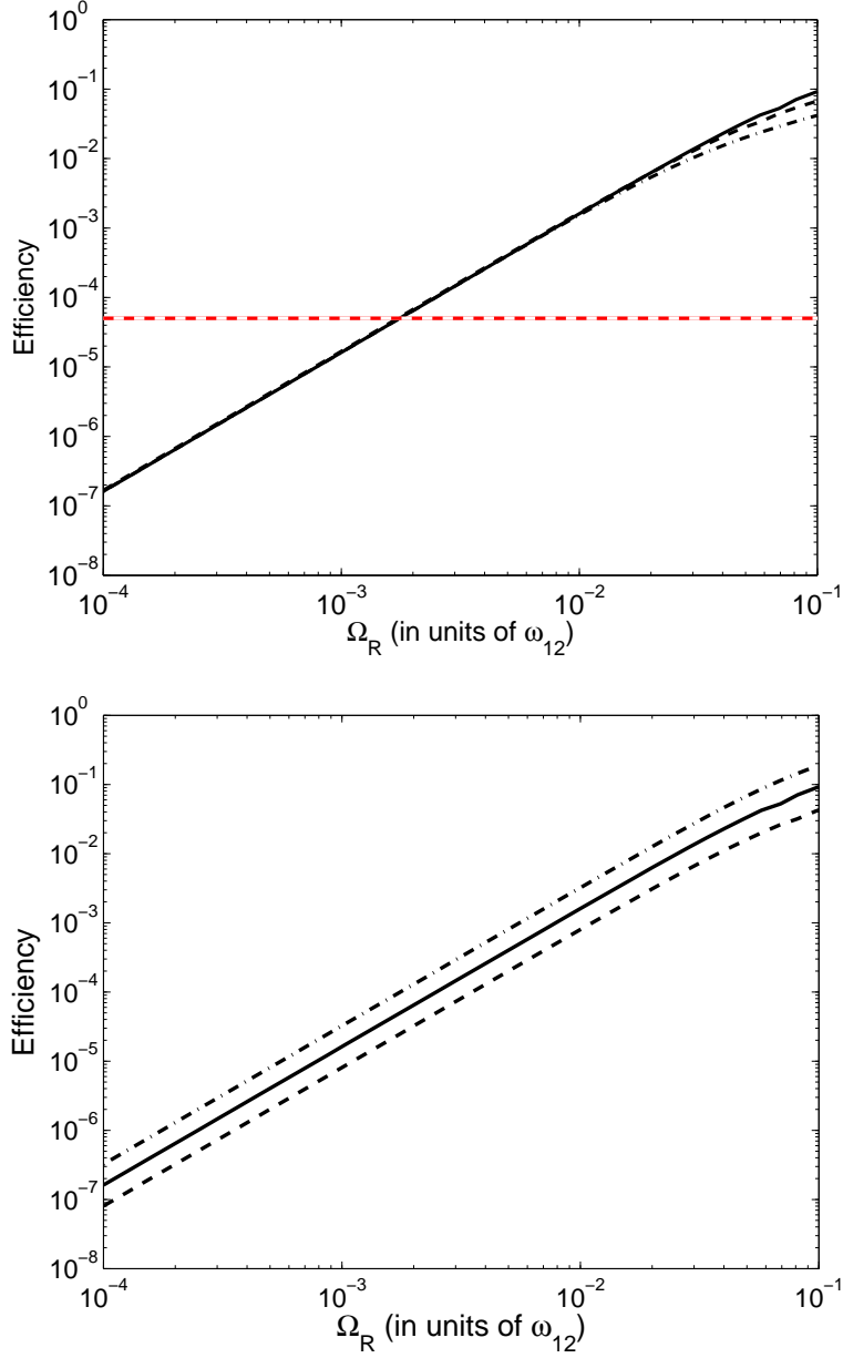
Figure 3.6: Quantum efficiency versus the corresponding resonant vacuum Rabi frequency at the voltage eV = \hbar\omega_{12} for \hbar\omega_{12} = 150 meV. The three lines in the top panel are obtained with different values of the coherence damping coefficients: \Gamma_X = \Gamma_Y = 0.1\omega_{12} (solid line), 0.05\omega_{12} (dashed line) and 0.025\omega_{12} (dashed-dotted line). The three lines in the bottom panel are obtained with different values of the non-radiative relaxation rate: \frac{1}{\tau} = 0.01\omega_{12} (dashed line), 0.005\omega_{12} (solid line) and 0.0025\omega_{12} (dashed-dotted line). In red is marked a typical efficiency value in the free space (no cavity) case.
