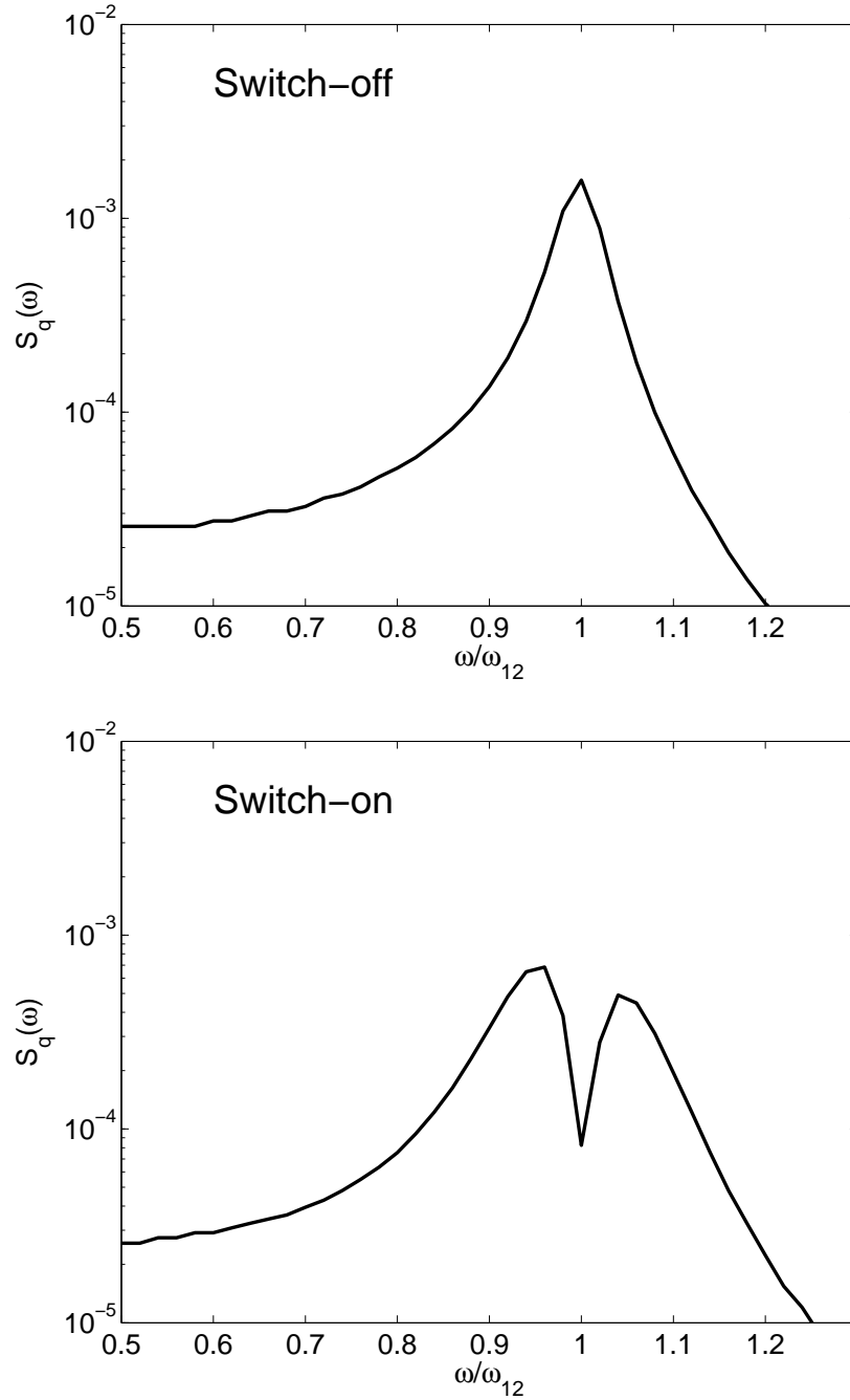
Figure 2.11: Spectra of emitted photons per radiant per unit time in the case of a switch off (top panel) and of a switch on (bottom panel). All the parameters are taken from Ref. [37].
