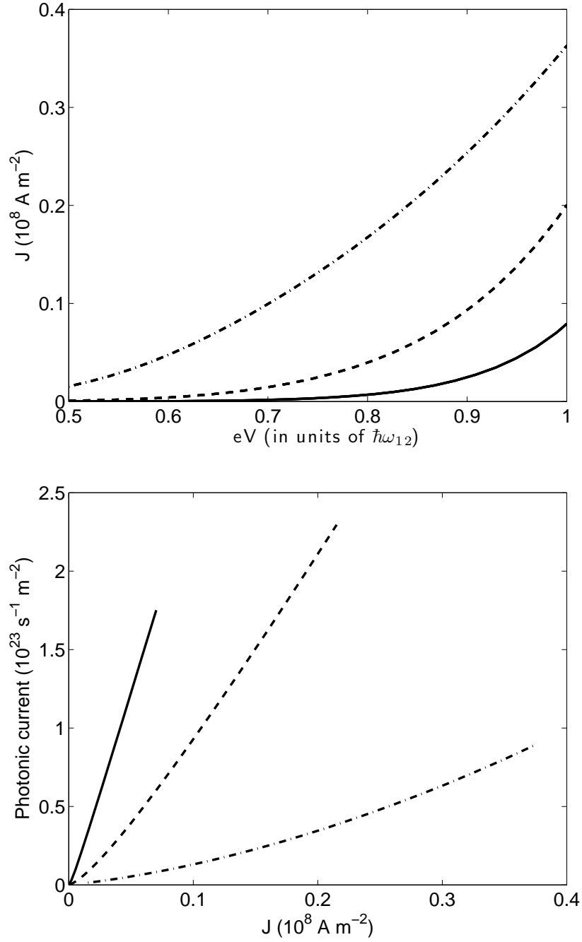
Figure 3.2: Current density versus applied voltage (top panel) and Photonic current density versus electronic current (bottom panel) for different values of the intersubband transition energy: \hbar\omega_{12} = 50 \text{ meV} , (dashed-dotted line), 100 \text{ meV} (dashed line) and 150 \text{ meV} (solid line).
