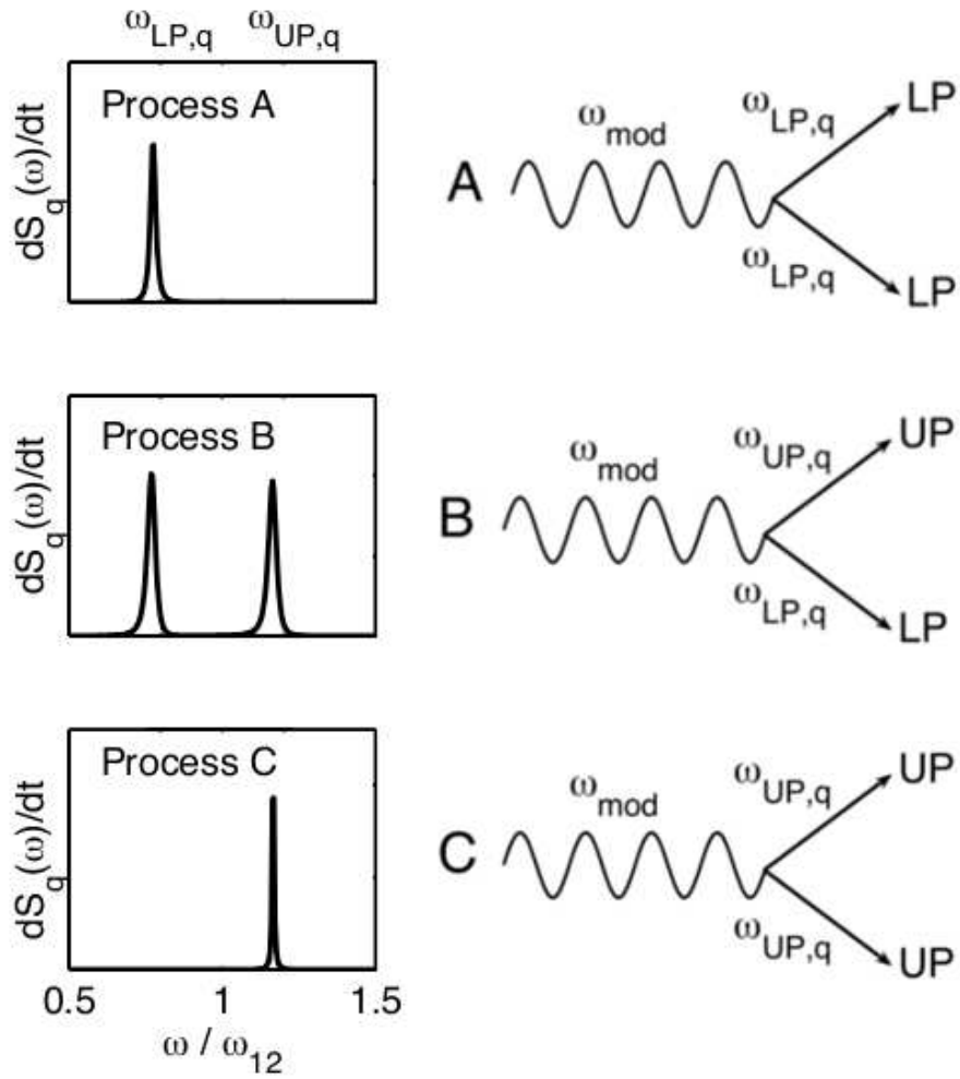
Figure 2.6: On the left are plotted the spectral densities of emitted photons (arb. u.) for the processes A, B and C of Fig. 2.5. On the right there is a schematic representation of the three phase-matched parametric processes involved.
