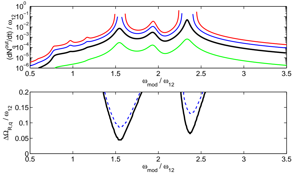
Figure 2.8: Top panel: rate dN_q^{\text{out}}/dt (in units of \omega_{12} ) of quantum vacuum fluorescence as a function of \omega_{\text{mod}}/\omega_{12} for different values of the normalized modulation amplitude \Delta\Omega_R(q)/\omega_{12} = 0.01, 0.04, 0.07, 0.1 (from bottom to top) and \Gamma/\omega_{12} = 0.025 . Other parameters as in Fig. 2.5. Bottom panel: instability boundaries for \Gamma/\omega_{12} = 0.025 (solid black) and 0.05 (dashed blue). Above the lines, the system is parametrically unstable.
