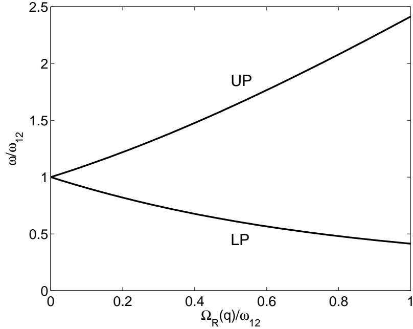
Figure 2.2: Normalized polariton frequencies \omega_{LP,q}/\omega_{12} and \omega_{UP,q}/\omega_{12} as a function of \Omega_R(q)/\omega_{12} . The calculation has been performed with \mathbf{q} such that \omega_{cav}(q) + 2D(q) = \omega_{12} . See Ref. [25].
