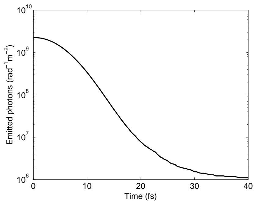
Figure 2.12: Total number of emitted Casimir photons as a function of the full width half maximum length (FWHM) of the pump pulse. All the other parameters are taken from Ref. [37].
