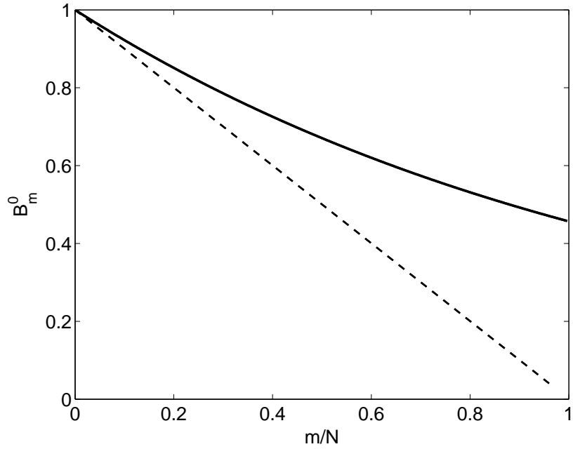
Figure 5.2: The solid line represents the bosonicity factor B_m^{n=0} versus m/N for the pump and signal polariton modes considered in Fig. 5.1. For pure bosons B_m^n is always 1. The dashed line is the same quantity for pure matter excitations. For m/N \ll 1 , deviations from perfect bosonicity are negligible.
