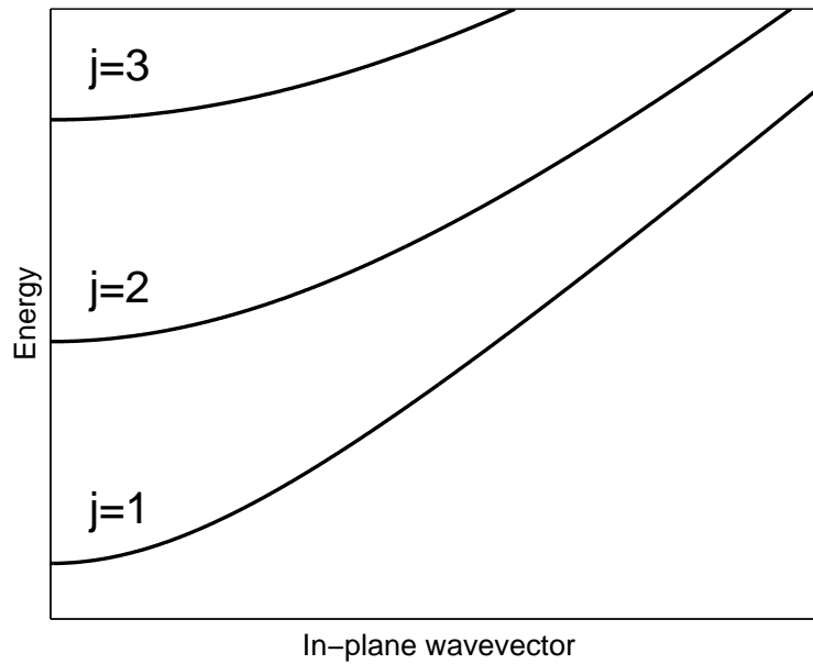
Figure 1.2: Energy dispersion of a planar microcavity as a function of the wavevector in the plane normal to the growth direction. The index j indexes different photonic branches corresponding to different values of the quantized wavevector along the growth direction.
