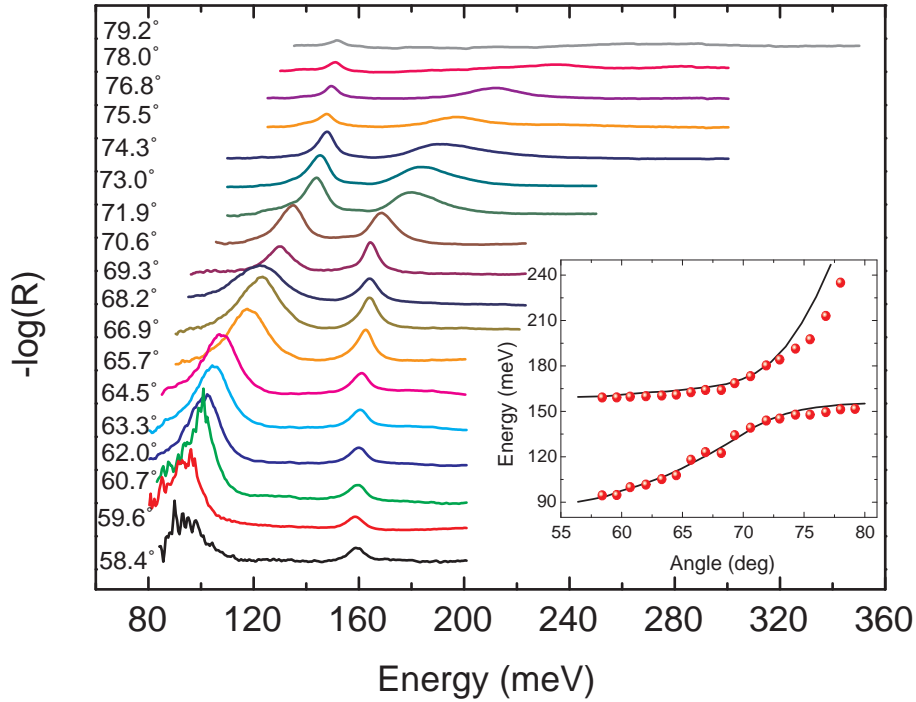
Figure 1.5: Reflectivity spectra as a function of the incident angle. In the inset the position of the peaks (full dots) is compared with the theoretical results of transfer matrix calculations (line). Image taken from Ref. [39].
