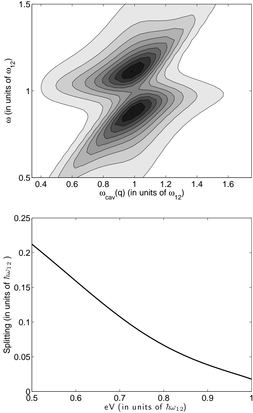
Figure 3.5: Top panel: contour plot of the electroluminescence (arb. units) as a function of the bare cavity photon energy \omega_{cav}(q) and of the emission frequency \omega for an applied voltage eV = 0.5\hbar\omega_{12} . Bottom panel: minimum polariton splitting as a function of the applied voltage for \hbar\omega_{12} = 150 meV.
