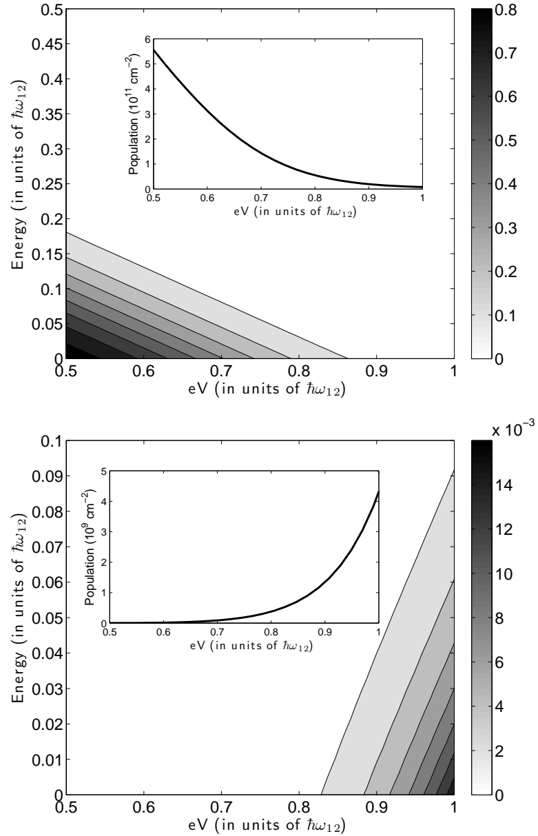
Figure 3.3: Electron occupation number in the first (top panel) and second (bottom panel) conduction subband as a function of kinetic energy and applied voltage. In the insets there are the integrated density of electrons in the two subbands versus voltage. In these simulations \hbar\omega_{12} = 150 \text{ meV} .
