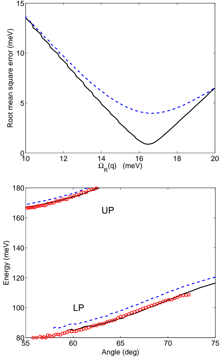
Figure 2.9: Top panel: root mean square deviation from measured dispersion of the calculated polariton energies as a function of the vacuum Rabi energy, the only fitting parameter. The solid black line refers to the \bar{H}_{bos} , while the dashed blue one to the bosonic RWA Hamiltonian. Bottom panel: angular dispersions of the lower and upper polaritons in the two cases compared to experimental data (red circles). The \Omega_R(q) used are the ones that minimize the error.
