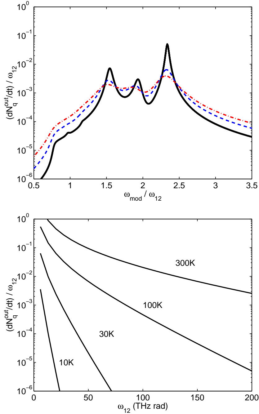
Figure 2.7: Top panel: rate dN_q^{out}/dt (in units of \omega_{12} ) of emitted photons as a function of \omega_{mod}/\omega_{12} for different values of the damping \Gamma/\omega_{12} = 0.025 (solid black), 0.05 (dashed blue), 0.075 (dot-dashed red). Other parameters as in Fig. 2.5. Bottom panel: normalized rate of emitted photons from a black-body emitter as a function of \omega_{12} for different temperatures.
