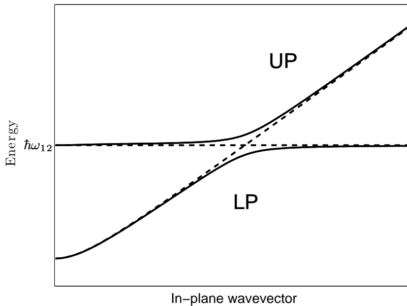
Figure 1.3: Energy dispersions of excitations in a microcavity embedded quantum well as a function of the wavevector in the plane normal to the growth direction. Dashed lines represent the dispersion of the intersubband excitation (dispersionless) and of the bare microcavity photon mode. Solid lines represent the upper (UP) and lower (LP) polariton branches.
