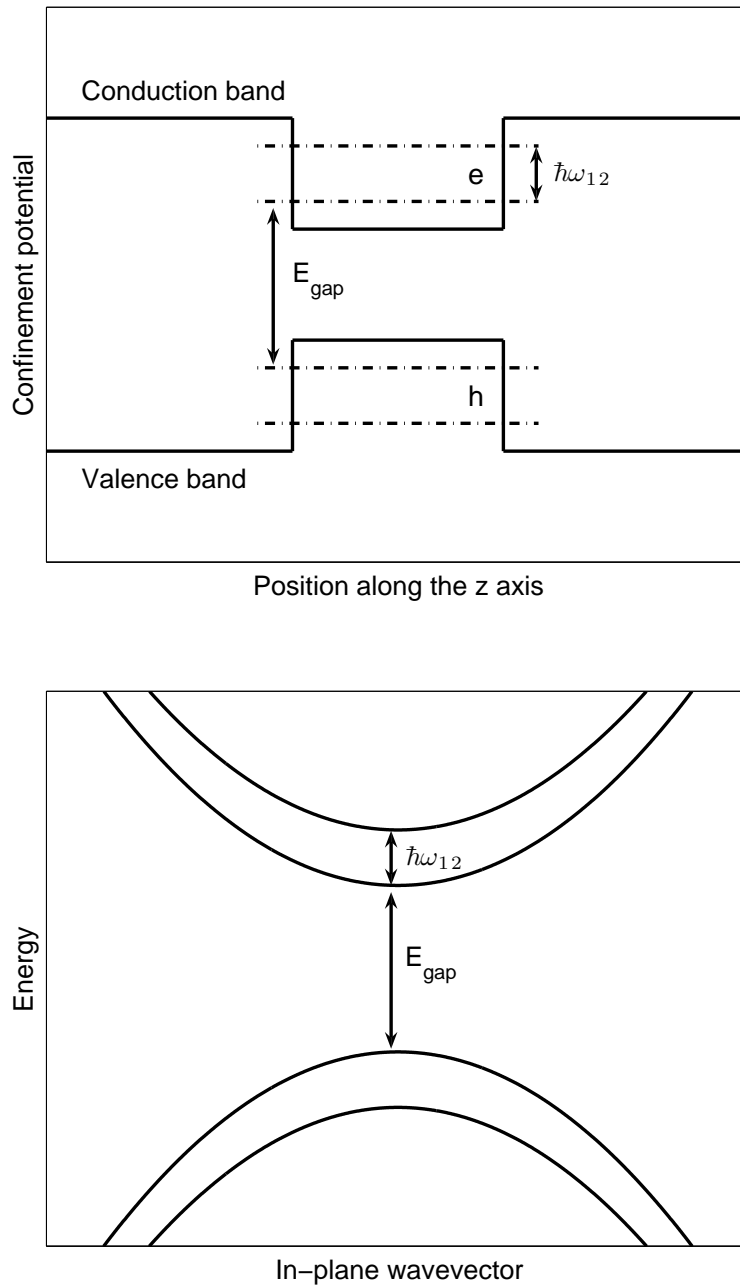
Figure 1.1: Top panel: schema representing the band structure of a semiconductor quantum well. The electronic confinement and the presence of subbands are well visible. Bottom panel: the corresponding band dispersion, as a function of the wavevector in the plane normal to the growth direction.
