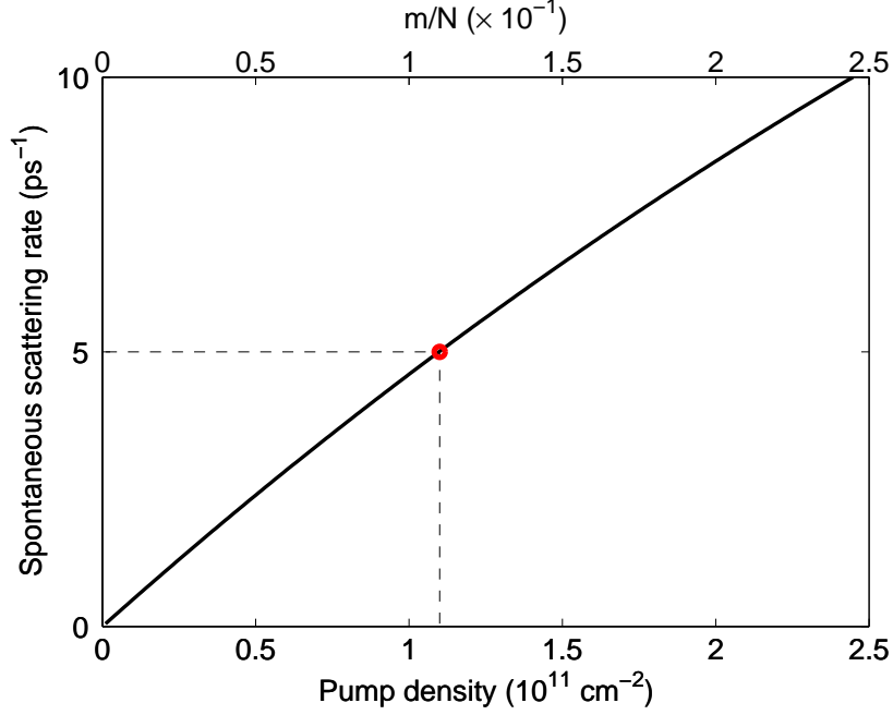
Figure 5.3: Spontaneous scattering rate \Gamma_{sc}^{m,n=0} from the pumped polariton to the signal polariton mode for the process depicted in Fig. 5.1 versus the pump polariton density m/S . The electron density in the ground state is N/S = 10^{12} \text{ cm}^{-2} . In the considered range of excitation densities, m/N < 0.25 , i.e., much smaller than the onset of electronic population inversion. Other GaAs parameters are given in the text.
