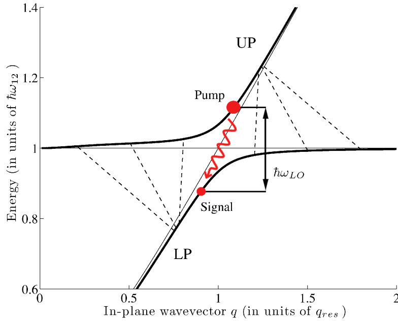
Figure 5.1: A typical energy dispersion (in units of the intersubband transition energy \hbar\omega_{12} ) of intersubband cavity polaritons versus in-plane wavevector (in units of the resonant wavevector q_{res} ). Due to the interaction with bulk optical phonons, a polariton pumped in the upper polariton (UP) branch can scatter into a final state (signal mode) in the lower polariton (LP) branch by emitting an optical phonon with energy \hbar\omega_{LO} (36 meV for GaAs). The considered modes have Hopfield coefficients \beta_{UP,\mathbf{q}} = \beta_{LP,\mathbf{q}} = 0.5 . The dashed lines indicate the same kind of scattering process by changing the in-plane momentum of the initial state along the upper polariton branch.
