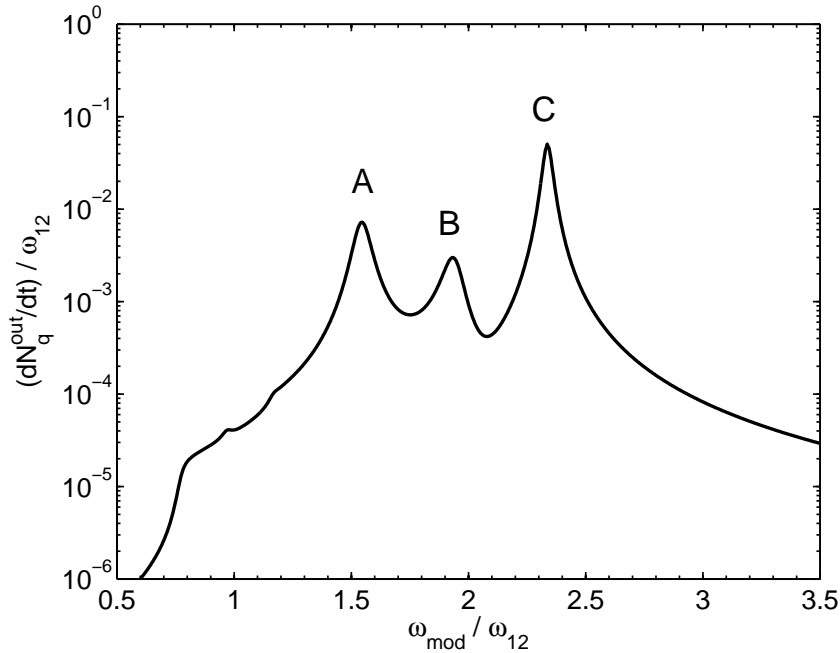
Figure 2.5: Rate of emitted photons dN_q^{out}/dt (in units of \omega_{12} ) as a function of the normalized modulation frequency \omega_{mod}/\omega_{12} . Parameters: (\omega_{cav}(q) + 2D(q))/\omega_{12} = 1 , \Gamma/\omega_{12} = 0.025 , \bar{\Omega}_R(q)/\omega_{12} = 0.2 , \Delta\Omega_R(q)/\omega_{12} = 0.04 . The letters A, B and C indicate three different resonantly enhanced processes.
