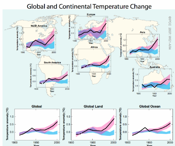
FIGURE 1 SPM-. Comparison of observed continental- and global-scale changes in surface temperature with results simulated by climate models using natural and anthropogenic forcings. Decadal averages of observations are shown for the period 1906–2005 (black line) plotted against the centre of the decade and relative to the corresponding average for 1901–1950. Lines are dashed where spatial coverage is less than 50%. Blue shaded bands show the 5–95% range for 19 simulations from 5 climate models using only the natural forcings due to solar activity and volcanoes. Red shaded bands show the 5–95% range for 58 simulations from 14 climate models using both natural and anthropogenic forcings.
