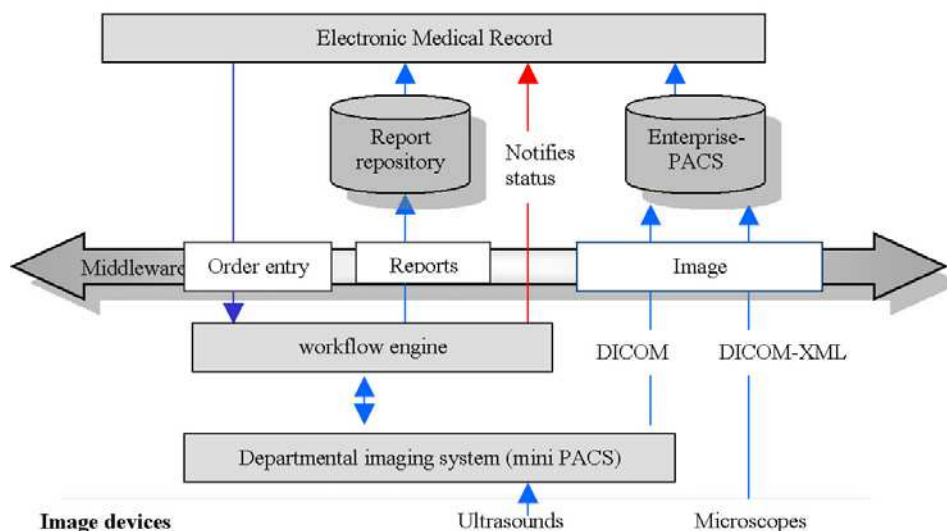
Fig. 3. Architecture used for cardiology (left) and haematology (right).
