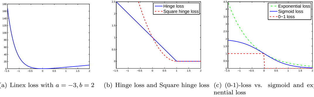
Figure 1.3: Classification loss functions, the horizontal axis indicates the value of yf(\mathbf{x}) while the vertical axis is the output value for the loss function.
