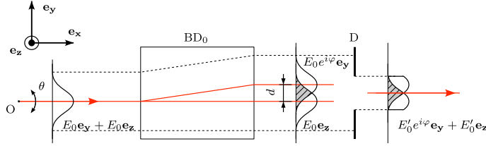
Fig. 2. Experimental setup: measurement area. A collimated 6.6 mm He-Ne laser beam can be rotated around e_z by means of a piezo driven kinematic mount. After passing through a parallel beam displacer (40 mm calcite prism, BD_0 ), the two resulting crossed polarized rays present a phase shift \varphi dependent on the angle of incidence \theta . We limit the two beams to their overlapping part using a diaphragm ( D ), and analyze the emerging light ray into the analysis area.
