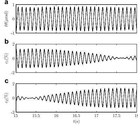
Fig. 7. Zoom of Fig. 6: fast signals \delta\theta (a), c_1 (b), c_2 (c) around minimums of C_1 and C_2 . The reconstructed angular position \delta\theta is independent of the working point.
