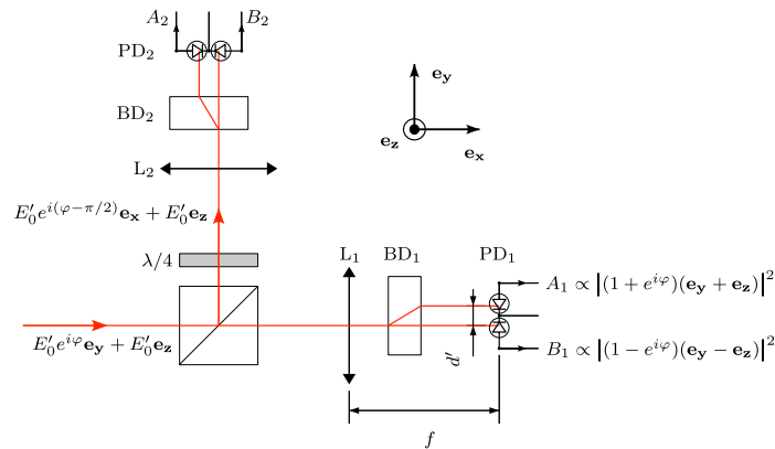
Fig. 3. Experimental setup: analysis area. The light coming from the measurement area is split into two arms. In each one, a 5 mm calcite prism (beam displacers BD_n , n = 1,2 ) oriented at 45^\circ with respect to the measurement beam displacer ( BD_0 ) projects the polarizations to have them interfere. The two beams emerging BD_n are focused (plano convex lens L_n , f = 25 mm) on the two segments of a two quadrant photodiode PD_n to record their intensities A_n , B_n . Those are used to reconstruct \varphi and thus measure \theta . In the second analyzing arm ( n = 2 ), a quarter wave plate ( \lambda/4 ) is added in order to subtract \pi/2 to the phase shift \varphi .
