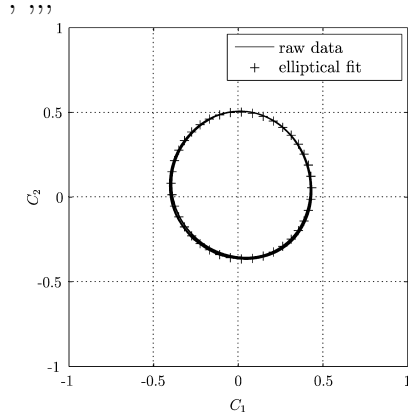
Fig. 5. Due to experimental imprecisions, the measurement lays on a tilted ellipse in the C_1 , C_2 plane. These deviations to the C_{\max} radius circle can easily be corrected [13]. We present the raw data to show that corrections are small anyway.
