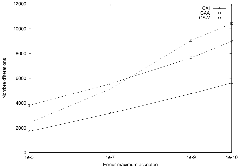
FIG. 5.5 – CFR- 15 noeuds
