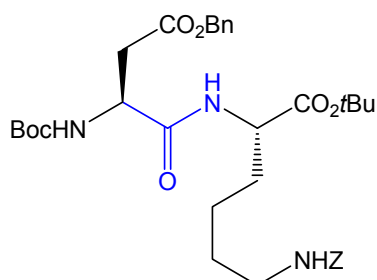
réversine 121 N^{\alpha} -Boc-Asp(OBn)-Lys(Z)-OtBu
