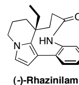
(-)-Rhazinilam
