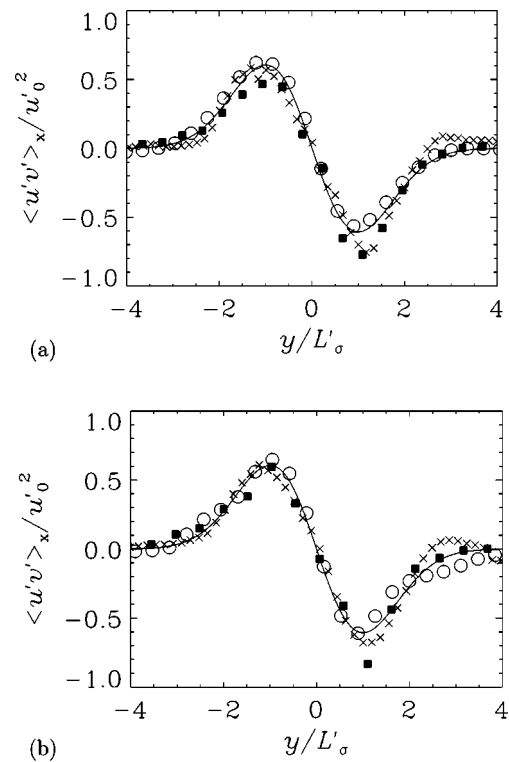
FIG. 7. Streamwise-averaged profile of the Reynolds stress u'v' for the slender spheroid (a) and the cylinder (b) at three downstream distances: x/D=1000 (■), x/D=1000 (○), and x/D=5000 (×). F=32 and Re \approx 5000 . Solid lines correspond to the theoretical prediction (8) found in self-preserving wakes.
