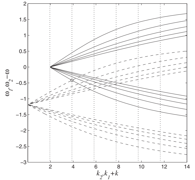
FIG. 3. Dispersion relations of the Kelvin modes. The solid lines (resp. dashed lines) correspond to the first five branches of the Kelvin modes with azimuthal wavenumber m_1=5 (resp. m_2=6 ). The solid lines have been translated by k=\pi/h and the dashed lines have been translated by \omega=1.18 . The vertical dotted lines correspond to k=n\pi/h , with n an integer, ( h=1.62 , \omega=1.18 ).
