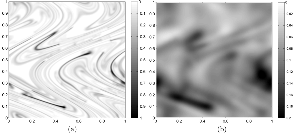
FIGURE 14. Spatial distribution of a strip of scalar in a Sine flow at t = 7 for a Péclet number equal to (a) 10^5 and (b) 10^3 . All points of the strip have been translated into the unit square in order to model a periodic initial condition (and flow) composed of a column of strips infinite in x and located at y = \dots - 2, -1, 0, 1, 2, \dots
