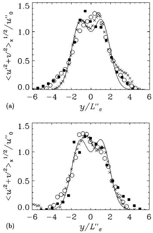
FIG. 9. Streamwise-averaged profile of the turbulent kinetic energy for the slender spheroid (a) and the cylinder (b) at three downstream distances: x/D=170 (■), x/D=1000 (○), and x/D=5000 (×). F=32 and Re\approx 5000 . Solid lines correspond to the fitting function of Eq. (11).
