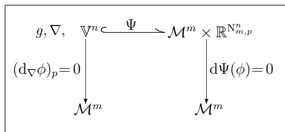
Figure 5.1: Generalized isometric embedding
