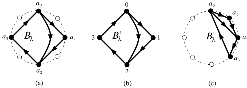
Figure 3.1: (a) Digraph B_\lambda admissible for n = 8 and C = 2 ; (b) Its associated digraph B_\lambda^4 ; (c) Non-admissible digraph B'_\lambda that has also B_\lambda^4 as associated digraph.
