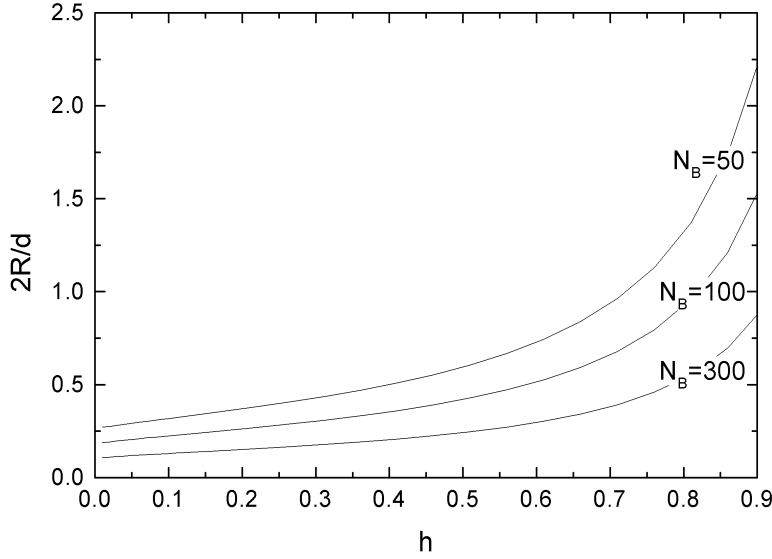
Figure 11.7: Reduced diameter 2R/d as a function of the reduced magnetic field h .
