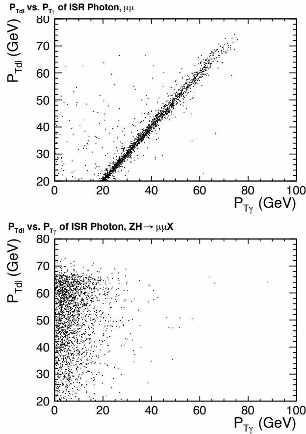
Figure 6.10: Correlation between P_{\text{Tdl}} and P_{\text{T}\gamma} for the \mu\mu process (top) and for the Higgs-strahlung \mu\mu X process (bottom).
