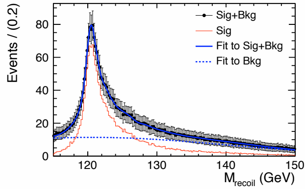
Figure 6.32: Fit to the signal plus background using Kernel Estimation for eeX -channel with polarization mode e_L^- e_R^+ in MD analysis, with Bremsstrahlung recovery.
