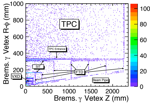
Figure 3.10: Vertices of Bremsstrahlung photons. The accumulation of vertices corresponds to the passive material of detector components as labeled. Figure is drawn using the Higgs-strahlung sample with Z \rightarrow e^+e^- .
