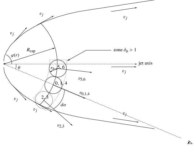
Fig. 1. Geometric side view of the jet formation zone (“on-blob” case). v_j represents the velocity of the jet, the blobs are numbered from 0 to 6, v_{0\rightarrow6} are the velocities of the blobs, \theta is the viewing angle with respect to the jet axis, \varphi(r) is the opening angle, r_b is the radius of an individual blob, and R_{\text{cap}} is the distance of the blobs from the SMBH. In this sketch, the contributions to the total flux of the blobs No. 2 and 3 would be rejected, since they lie outside the jet.
