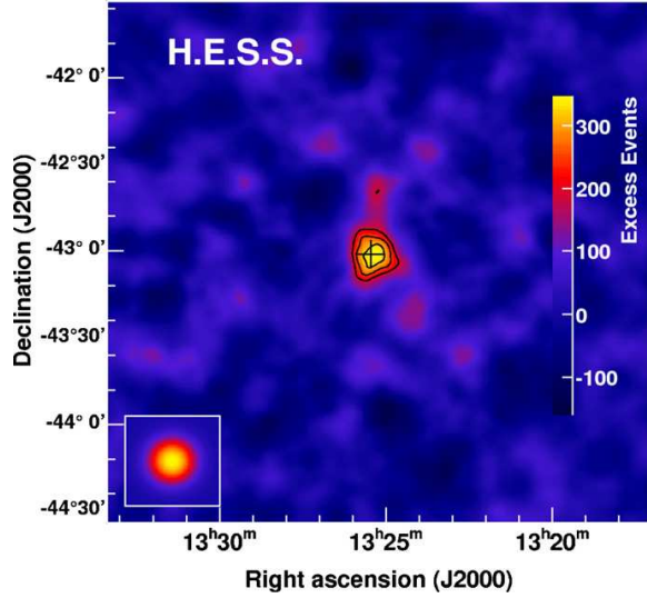
Figure 1. Smoothed excess sky map centered on the Cen A radio core (cross). Overlaid contours correspond to statistical significances of 3, 4, and 5 \sigma , respectively. The inset in the lower left corner shows the excess expected from a point source (derived from Monte Carlo simulations). The integration radius is 0:1225 and the map has been smoothed with a two-dimensional Gaussian of radius 0:02 to reduce the effect of statistical fluctuations. The cosmic-ray background in each bin is estimated using the template background method (Rowell 2003).
