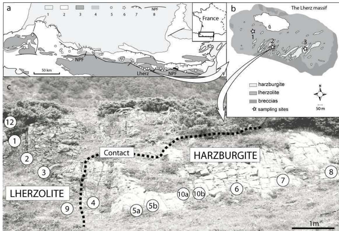
Fig. 1: (a) Distribution of the Pyrenean peridotite bodies along the North Pyrenean Fault (NPF), from Lagabriele and Bodinier (2008) after Choukroune (1978). 1: Oligocene and post-Oligocene sediments; 2: Mesozoic and Eocene sediments; 3: Paleozoic basement; 4: area of LP-HT Pyrenean metamorphism; 5: lherzolite bodies; 6: granulites; 7: main thrusts external zones; 8: North Pyrenean Fault. (b) Harzburgites and lherzolites intermingling in the Lherz massif (Le Roux et al., 2007); the location of the sampling sites are indicated on the map, 1: distal lherzolite; 2: profile through a contact; 3: distal harzburgites. (c) Detailed sampling site 2 through a harzburgite-lherzolite contact.
