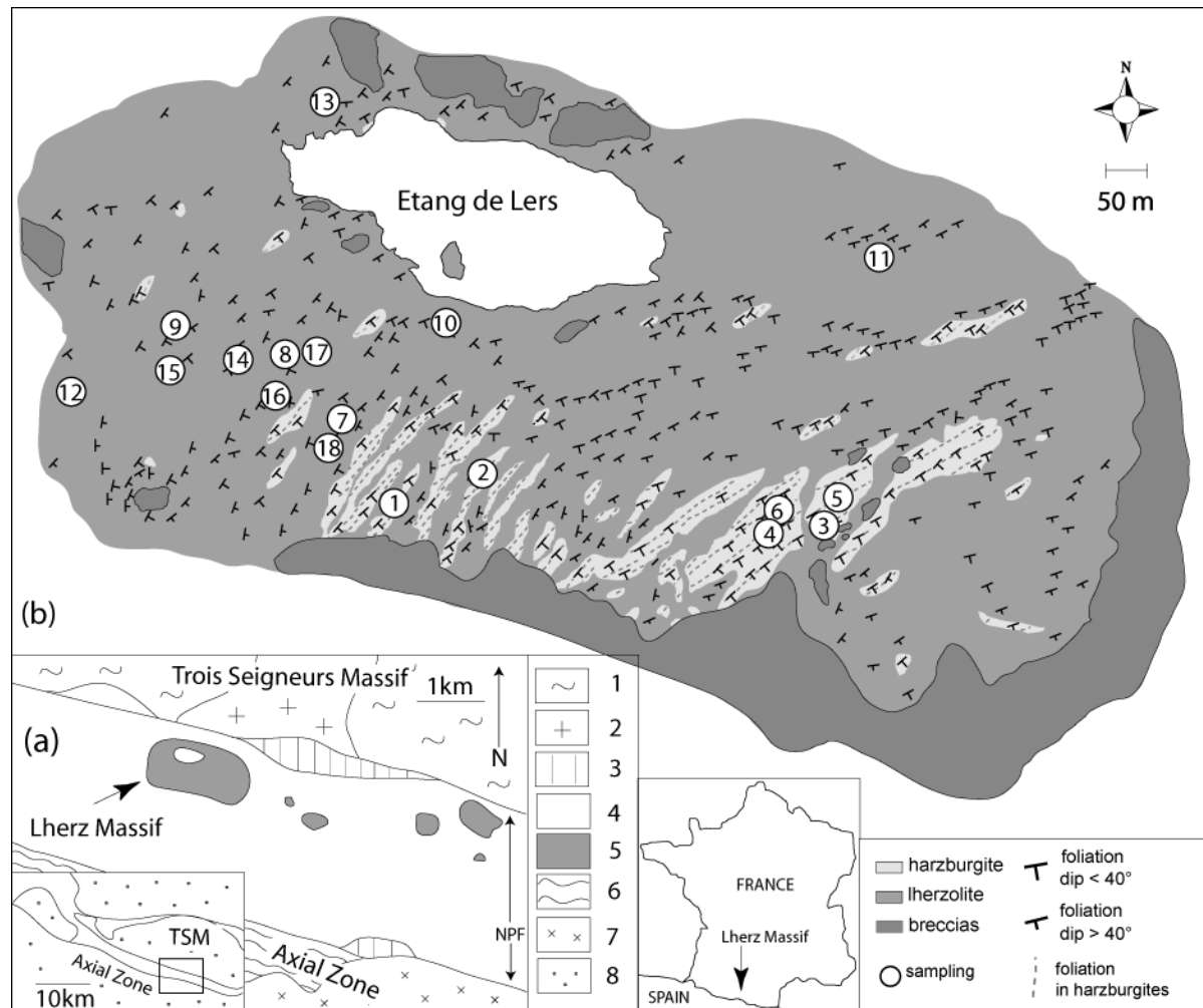
Fig. 1: (a) Localization and geological context of the Lherz Massif (Azambre and Ravier, 1978; Kornprobst and Vielzeuf, 1984; Monchoux, 1970; Vielzeuf, 1980). 1- Schists; 2- Mesozoic and Cenozoic rocks; 3- Granulites; 4- Metamorphic Mesozoic rocks; 5- Peridotites; 6- Granulite occurrences; 7- Hercynian basement; 8- Late Tertiary sediments. (b) Geological map of the Lherz Massif (Le Roux et al., 2007) with the location of analyzed samples.
