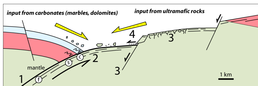
Fig. 3: Possible geological setting and mode of emplacement of the ultramafic bodies and associated clastic rocks (Lagabriele and Bodinier, 2008). Blue: Jurassic platform carbonates; pink: continental crust; green: mantle; 1: detachment leaving late foliation in mantle rocks; 2: LT shear zone(s), cataclasites (c) and exhumation to seafloor; 3: late normal faulting, weathering and brecciation; 4: gravity sliding and sedimentary reworking.
