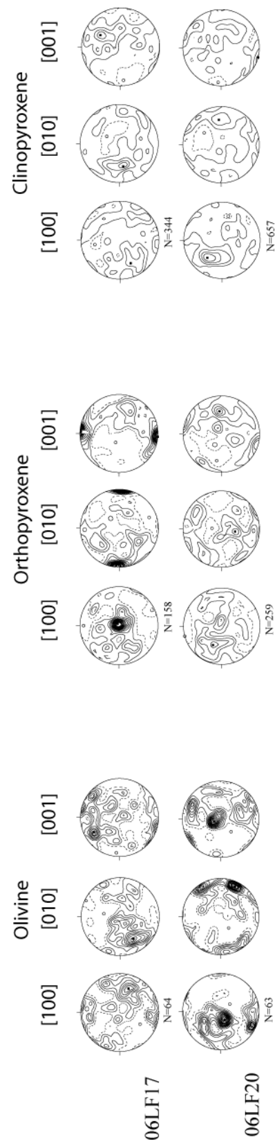
Figure 1 : Crystal-preferred orientations of olivine, orthopyroxene and clinopyroxene in harzburgites, lherzolites and websterites from the Lherz massif. Lower hemisphere equal area projections in the geographic reference frame (N at the top, E on the right). Contours at 0.5 of multiple of an uniform distribution intervals. 1 measurement per grain. N= Number of grains measured.
