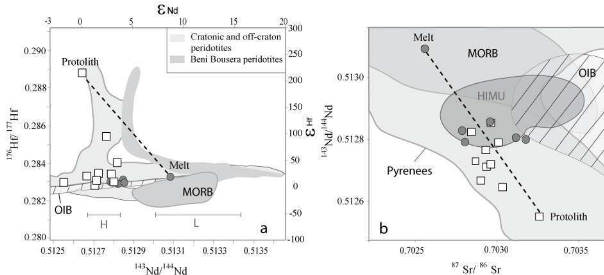
Fig. 3: (a) ^{176}\text{Hf}/^{177}\text{Hf} (and \epsilon_{\text{Hf}} ) versus ^{143}\text{Nd}/^{144}\text{Nd} (and \epsilon_{\text{Nd}} ) for 16 clinopyroxene separates from Lherz harzburgites (open squares) and lherzolites (solid circles), compared with the fields of Beni Bousera peridotites (Pearson and Nowell, 2004), cratonic and off-craton peridotites (Pearson and Nowell, 2004), MORB (Vervoort et al., 1999; Nowell et al. 1998) and Ocean-Island Basalts - OIB - (Salters and White, 1998). \epsilon_{\text{Nd}} and \epsilon_{\text{Hf}} are defined as ((^{143}\text{Nd}/^{144}\text{Nd}_{\text{sample}} / ^{143}\text{Nd}/^{144}\text{Nd}_{\text{CHUR}}) - 1) \times 10000 and ((^{176}\text{Hf}/^{177}\text{Hf}_{\text{sample}} / ^{176}\text{Hf}/^{177}\text{Hf}_{\text{CHUR}}) - 1) \times 10000 respectively (e.g. Blichert-Toft and Albarede, 1997). \epsilon_{\text{Nd}} and \epsilon_{\text{Hf}} are present-day values. The Nd isotopic ranges of Pyrenean harzburgites (H) and lherzolites (L) (Downes et al., 1991) are also shown for comparison. (b) ^{143}\text{Nd}/^{144}\text{Nd} versus ^{87}\text{Sr}/^{86}\text{Sr} for the same clinopyroxene separates compared with the fields of Pyrenean peridotites (Downes, 1991), MORB, OIB and HIMU (Hofmann, 1997; Zindler and Hart, 1986 and reference therein). The isotopic data for this study have been measured by TIMS and MC-ICP-MS techniques and corrected to 105 Ma, the age of exhumation. The differences between corrected and non-corrected isotopic ratios range between 1 \times 10^{-6} to 5 \times 10^{-6} .
