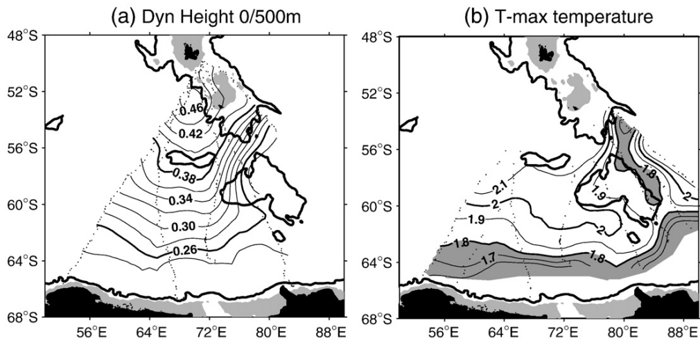
Fig. 8. Horizontal distribution of (a) surface dynamic heights (dyn m) relative to 500 m and (b) temperature at the T\text{-max} of the Upper Circumpolar Deep Water. The T\text{-max} colder than 1.8\text{ °C} is dark shaded.
